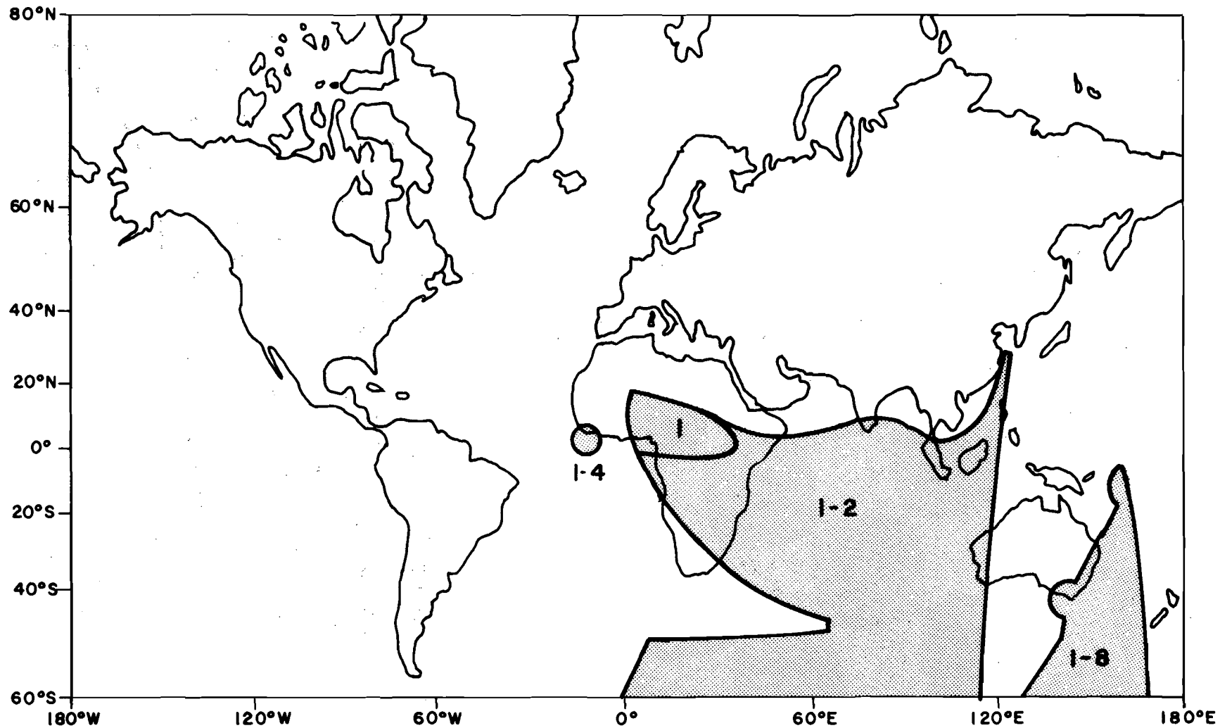
FIGURE 2. INADEQUATE SIGNAL COVERAGE DURING LA REUNION - ARGENTINA OUTAGE (-30 dB RECEIVER)
