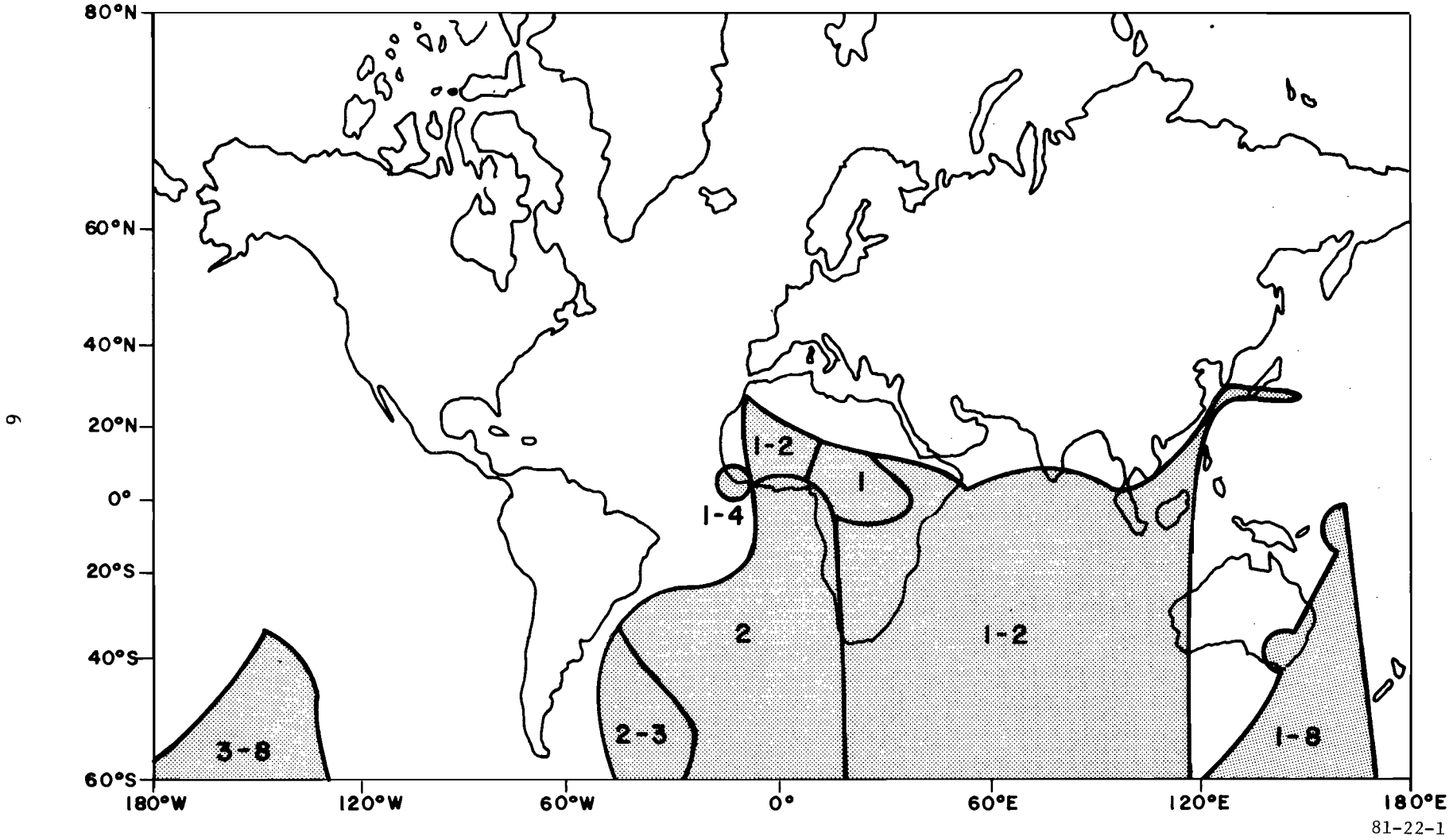
FIGURE 1. INADEQUATE SIGNAL COVERAGE DURING LA REUNION - ARGENTINA OUTAGE (-20 dB RECEIVER)
