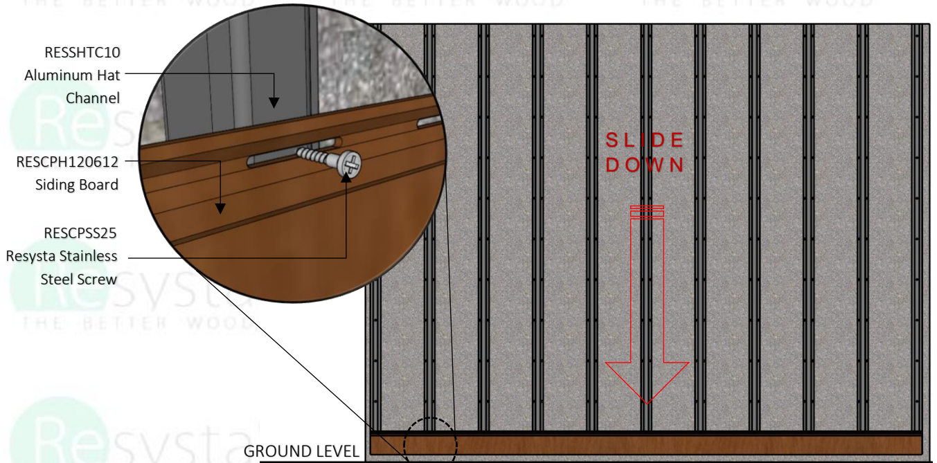
FRONT ELEVATION RESYSTA HORIZONTAL SIDING
