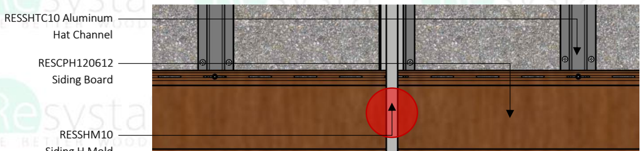
Gap Siding Spacing Ref. Table 1.2
