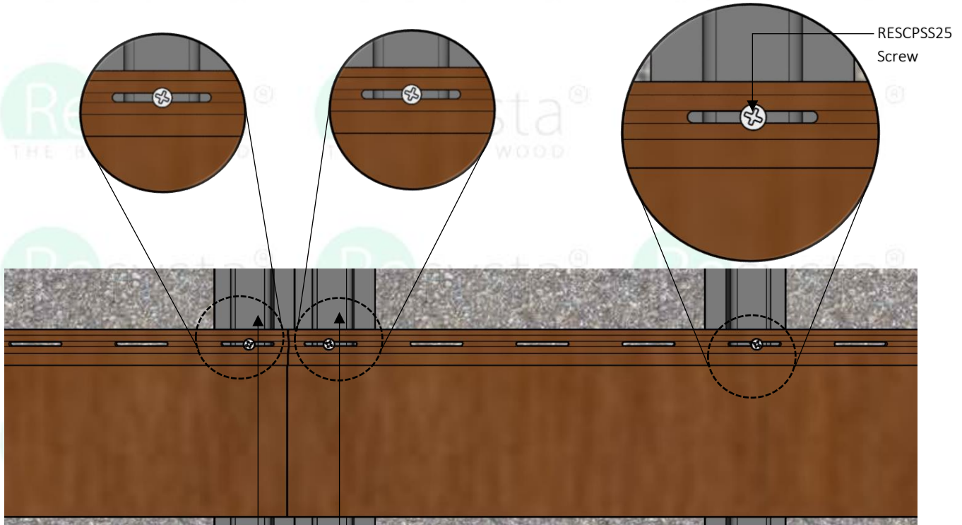
FRONT ELEVATION RESYSTA HORIZONTAL SIDING
