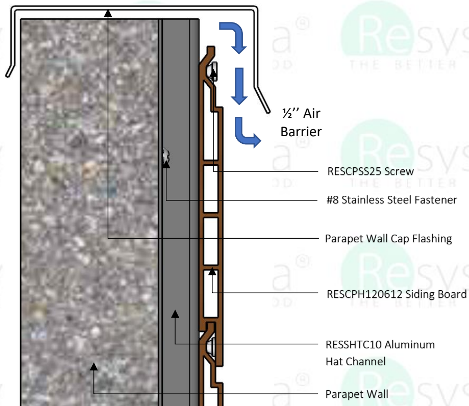
SIDE ELEVATION
