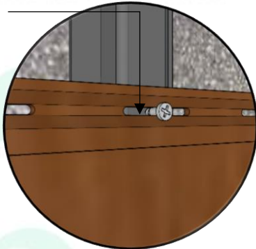
ISOMETRIC DETAIL SIDING BOARD INSTALLATION
