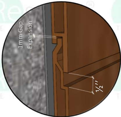
ISOMETRIC DETAIL RESYSTA HORIZONTAL SIDING
