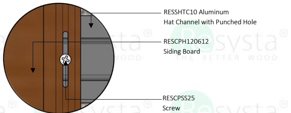
ISOMETRIC DETAIL RESYSTA VERTICAL SIDING
