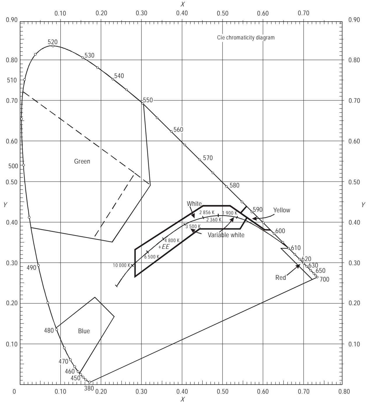
Figure A1-1. Colours for aeronautical ground lights
