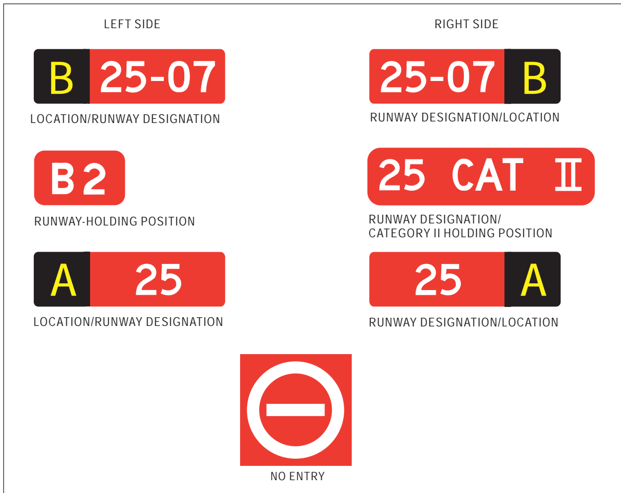
Figure 5-30. Mandatory instruction signs
