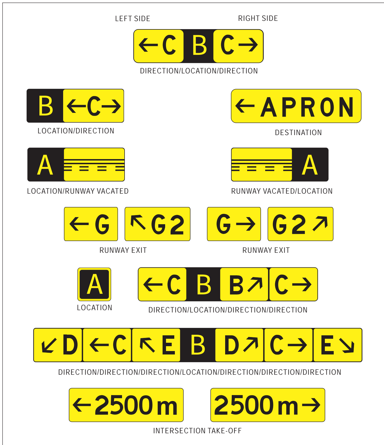
Figure 5-31. Information signs
