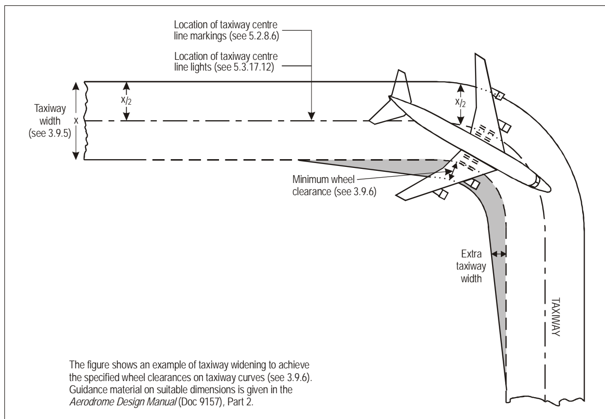
Figure 3-2. Taxiway curve
