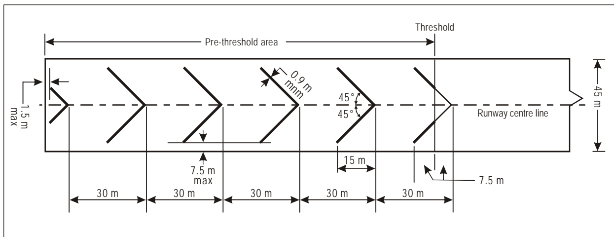
Figure 7-2. Pre-threshold marking
