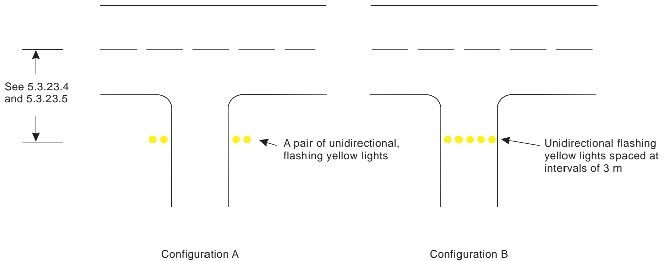
Figure 5-29. Runway guard lights
