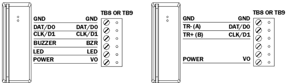
Typical 2-wire RS-485 Device (OSDP Reader for Example)
