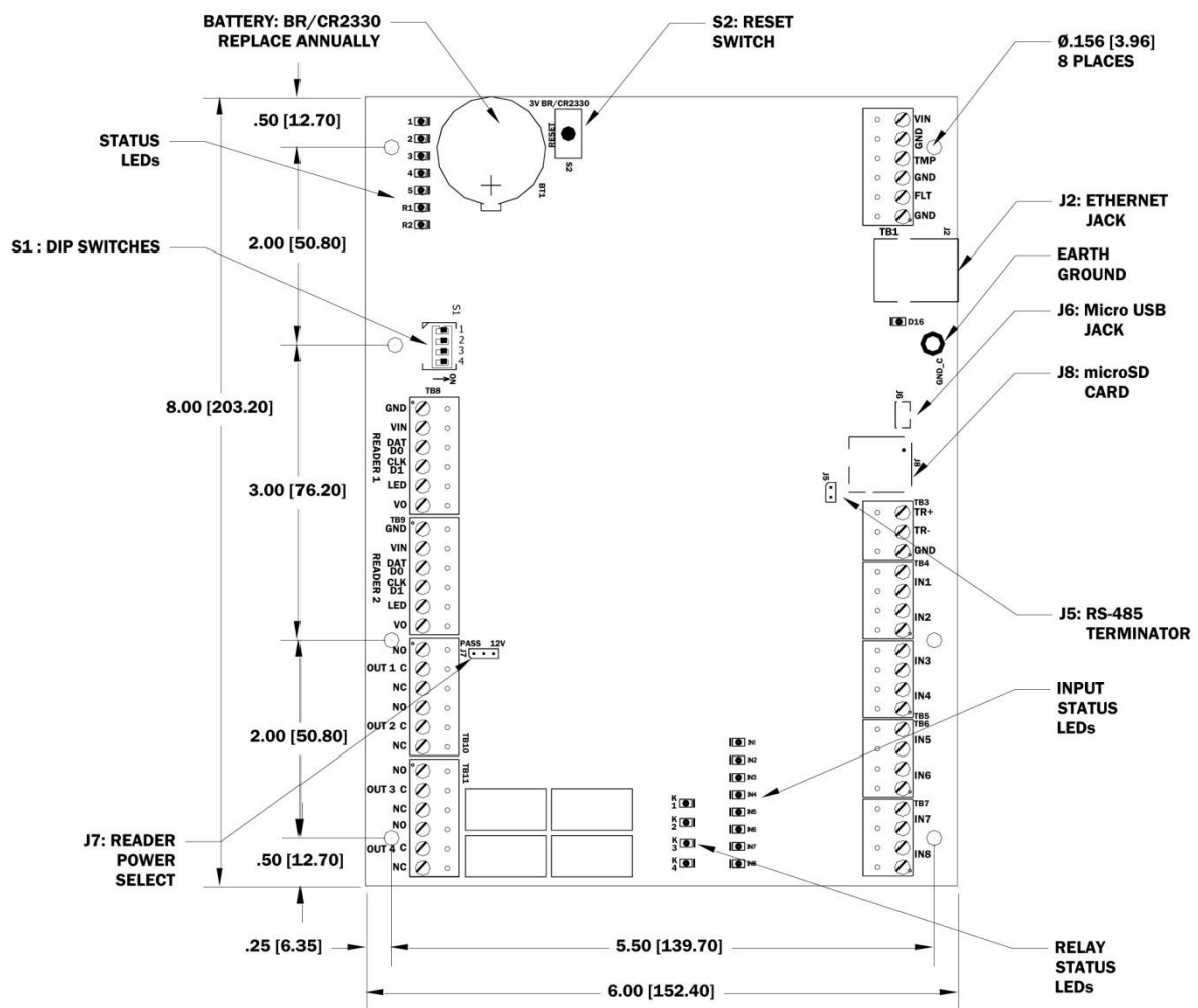
ICMLP-1502 Layout
