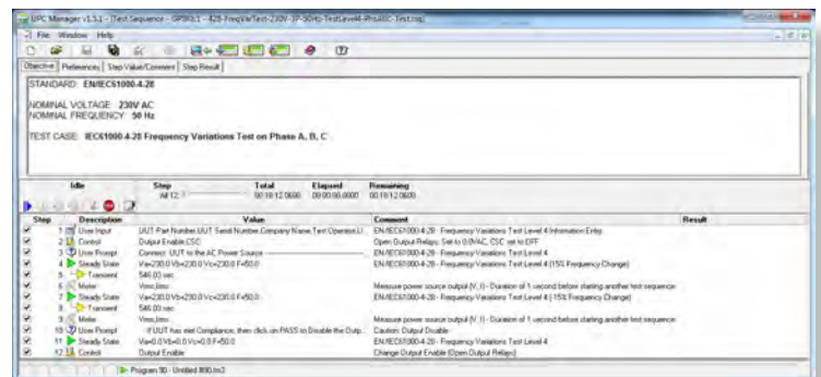
Figure 13: IEC 61000-4-28 Test Execution Control Screen
