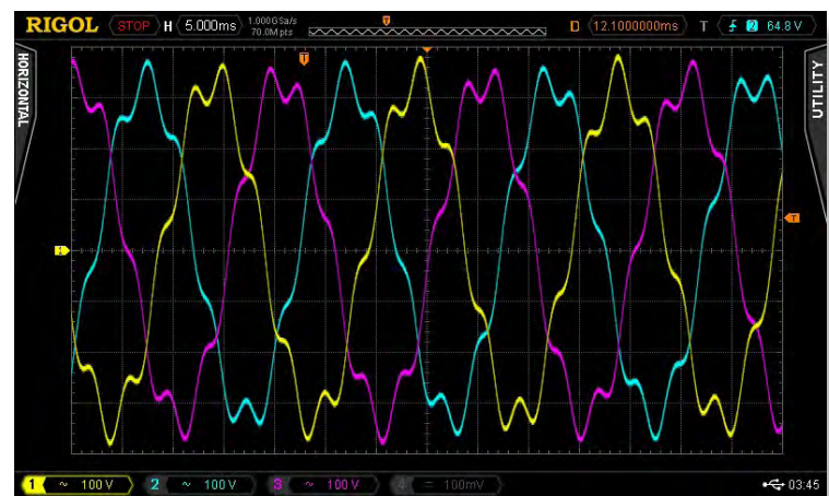
Figure 7: IEC 61000-4-13 Inter Harmonic Frequency Sweep Test
