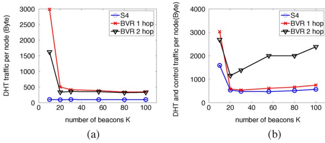
Fig. 7. Control traffic overhead comparison. (a) Location directory setup traffic. (b) Overall control traffic.
