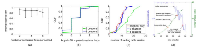
Fig. 20. Experiments on the 42-node testbed. (a) Routing success rate under multiple concurrent flows. (b) CDF of the hop count difference to pseudo optimal. (c) Routing table size. (d) Routing performance under node failure.
