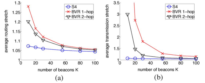
Fig. 3. S4 has routing and transmission stretches close to 1, which is consistently smaller than those of BVR algorithms across all numbers of beacons. (a) Routing stretch. (b) Transmission stretch.
