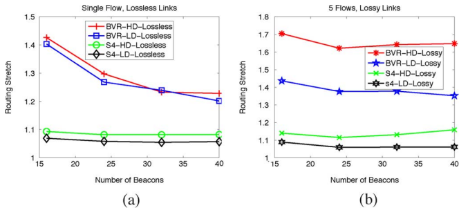
Fig. 10. Compare routing stretch under different numbers of beacons, network densities, and traffic patterns. (a) Lossless links with one flow. (b) Lossy links with five flows.
