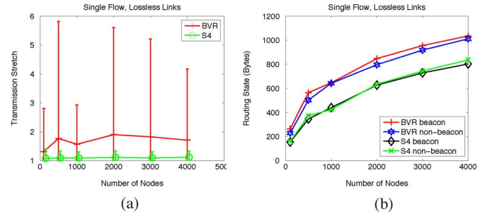
Fig. 15. Comparison under different network sizes. (a) Transmission stretch. (b) Routing state.
