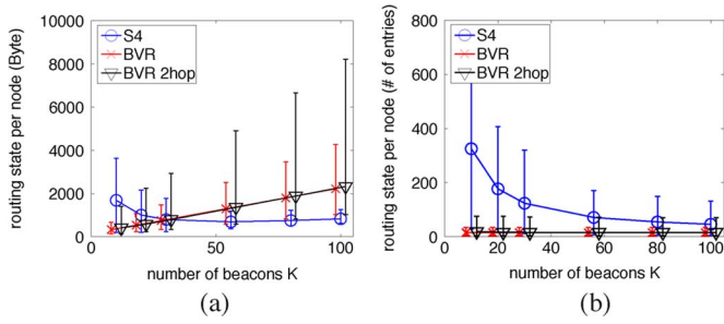
Fig. 4. Routing state comparison, where the errorbars show that when K = \sqrt{N} , the routing state in S4 is half of routing state in BVR. (a) Number of bytes. (b) Number of routing table entries.
