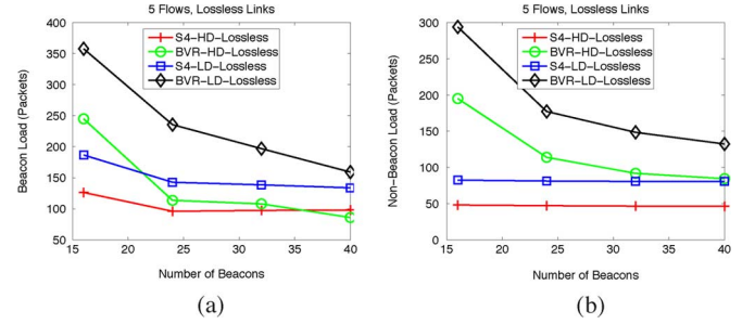
Fig. 14. Node load of data traffic under different numbers of beacons and network densities with lossless Links (five flows). (a) Beacon load. (b) Nonbeacon load.
