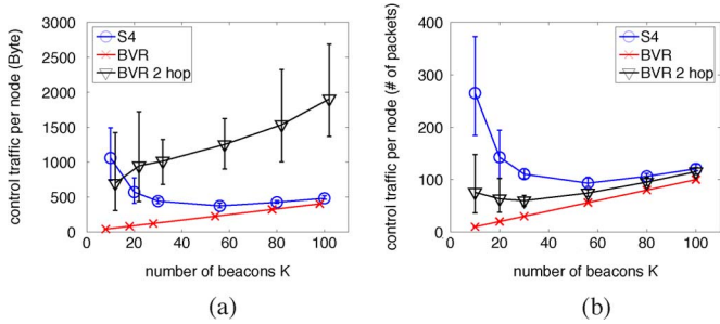
Fig. 5. Initial control traffic to set up routing state. The errorbars show minimum, mean, and maximum traffic across all nodes. The control traffic of S4 decreases gracefully as the number of beacons increases. When K = \sqrt{N} , the overhead of S4 is 65% higher than that of BVR 1-hop, but much less than BVR 2-hop. (a) Number of bytes. (b) Number of packets.
