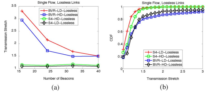
Fig. 11. Transmission stretch comparison. (a) Average transmission stretch. (b) CDF of transmission stretch.
