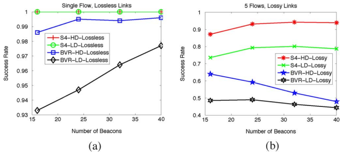
Fig. 9. Compare routing success under different numbers of beacons, network densities, and traffic patterns. (a) Lossless links with one flow. (b) Lossy links with five flows.
