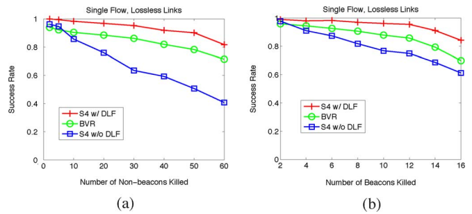
Fig. 17. Impact of DLF on success rate (1000 nodes, 32 beacons, low density). (a) Random nonbeacon failures. (b) Random beacon failures.
