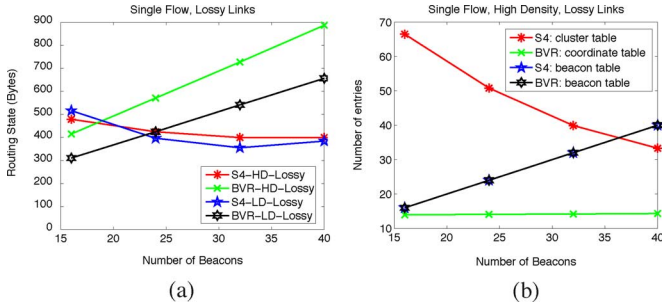
Fig. 13. Routing state comparison under different numbers of beacons and network densities with lossy links (single flow). (a) Average routing state. (b) Number of routing table entries.
