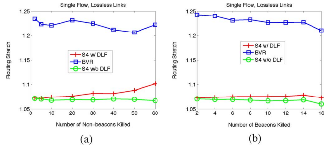
Fig. 18. Impact of DLF on routing stretch (1000 nodes, 32 beacons, low density). (a) Random nonbeacon failures. (b) Random beacon failures.
