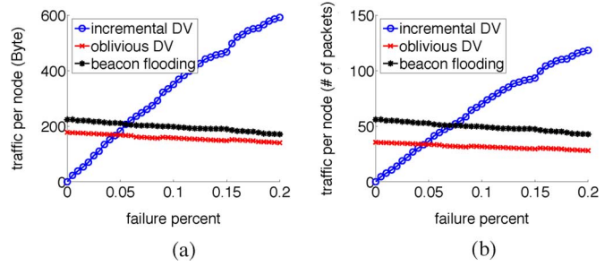
Fig. 6. Control traffic overhead of updating routing state due to topology changes. (a) Number of bytes. (b) Number of packets.
