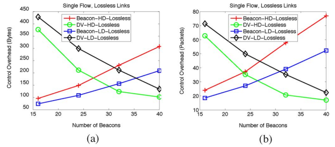
Fig. 12. Control traffic overhead under different numbers of beacons and network densities. (a) Control traffic in bytes. (b) Control traffic in packets.
