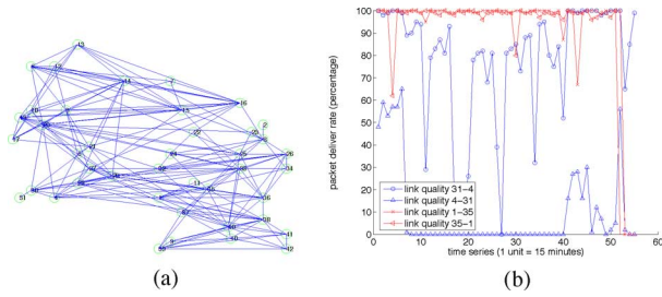
Fig. 19. Testbed measurement. (a) Topology snapshot. (b) Link quality.
