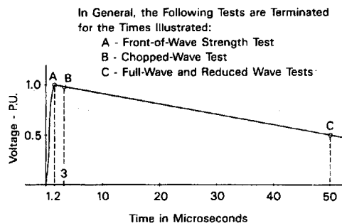
Figure 12 – TYPICAL IMPULSE TEST WAVESHAPE
