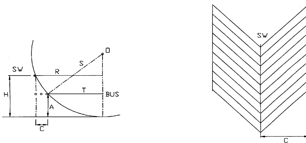
Exhibit B.5-5 — Calculations for shield wire protection of 500 kV substation
