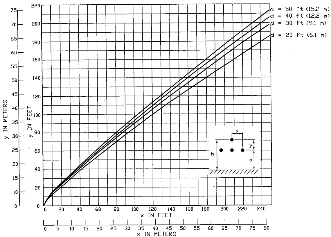
Figure 4-11 — Single shield wire protecting horizontal conductors—0.1% exposure. Height of shield wires above conductors, y , as a function of horizontal separation, x , and height of protected conductors, d
