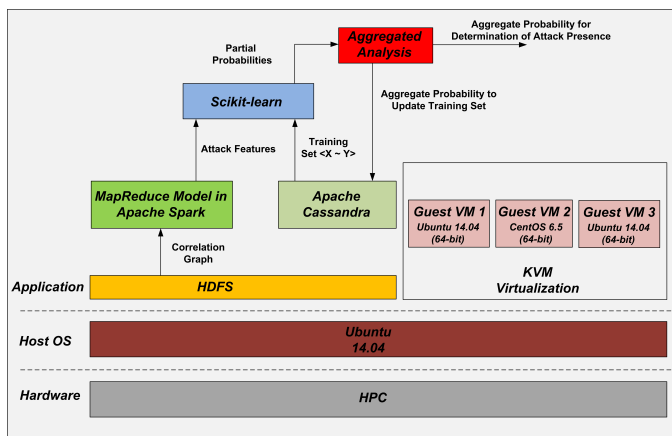
Fig. 7: Software stack on HPC node
