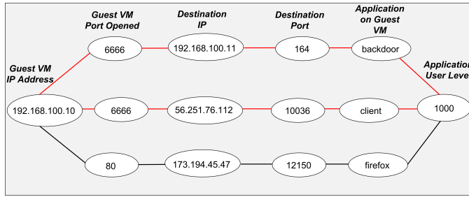
Fig. 3: Potential attack paths in the correlation graph as flagged up by MapReduce parser
