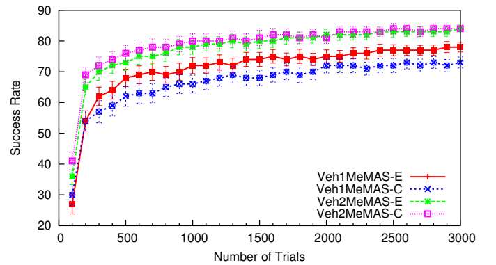
Fig. 12. Average success rate performance of tank agents in both MeMAS-E and MeMAS-C on completing the missions in AMNT.
