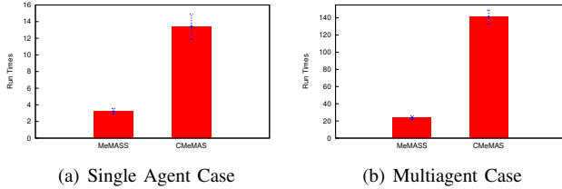
Fig. 10. Average Run Time (s) of MeMASS and CMeMAS in MNT. All experiments are run on Intel i7-3770 CPU (4 cores), 3.4 GHz, and 8G memory.
