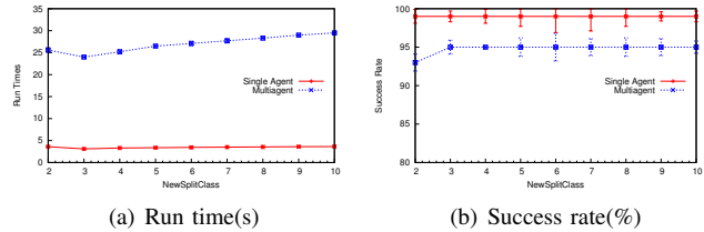
Fig. 7. Impact of the parameter NewSplitClass on the MeMASS performance in the MNT domain.
