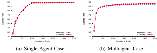
Fig. 9. Average Success Rate of MeMASS and CMeMAS in MNT.
