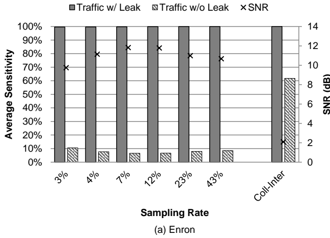
Fig. 5. Capability of differentiating real leak from coincidental matches of our AlignDLD approach with different sampling rates and Coll-Inter.
