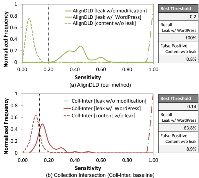
Fig. 2. Detection comparison of leak through WordPress in AlignDLD (a) and collection intersection (b). In each subfigure, each of the 3 curves shows the distribution of sensitivity values under one of 3 scenarios: leak without transformation, leak with WordPress transformation, or content without leak. With a threshold of 0.2, AlignDLD detects all the leaks. In comparison, collection intersection performs worse as shown in the table on the right.
