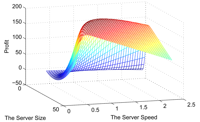
Fig. 4. The mesh of G(m, s) .
