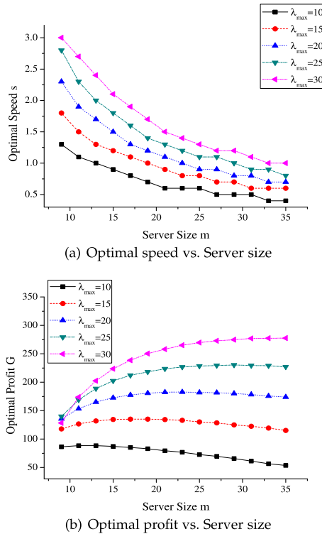
Fig. 7. Optimal speed and profit versus server size.
