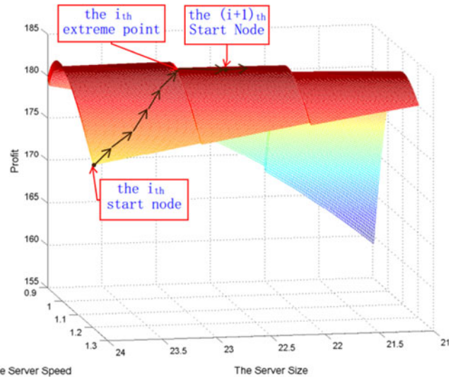
Fig. 6. The searching process.
