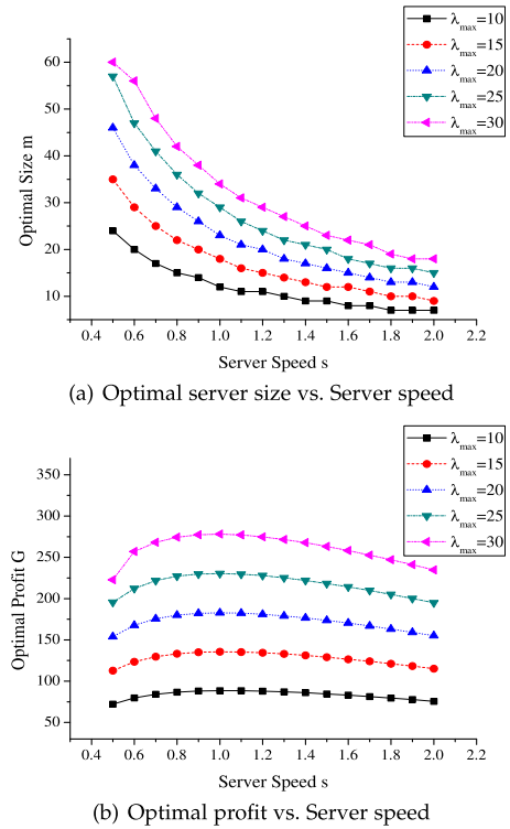
Fig. 8. Optimal server size and profit versus server speed.
