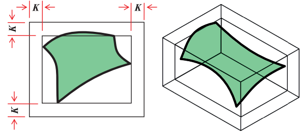
Fig. 5. We expand the AABBs by K in all three dimensions to guarantee that the surface patch is completely enclosed.
