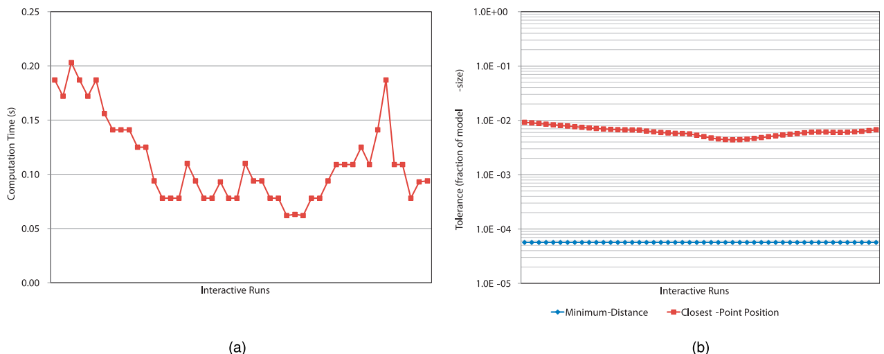
Fig. 16. Interactive times for evaluating the minimum distance between two NURBS surfaces and the corresponding distance and position tolerances scaled with respect to the maximum model size. (a) Computation time. (b) Tolerance.
