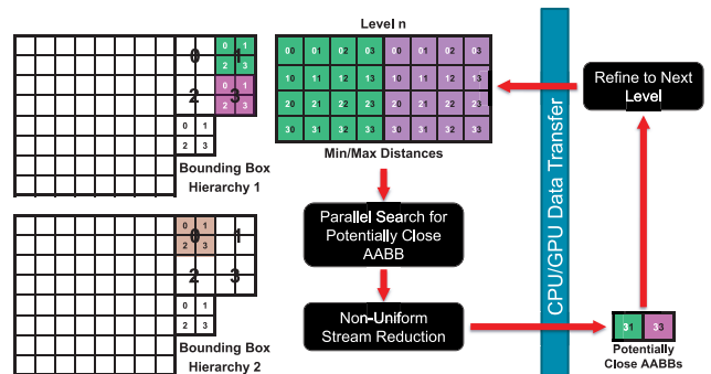
Fig. 10. We perform minimum distance computation between two NURBS surfaces with the help of AABB hierarchies for both the surfaces. We compute a list of potentially close bounding-boxes at each level using the GPU and then refine on the CPU until we reach a set of potentially close bounding-boxes at the lowest level.
