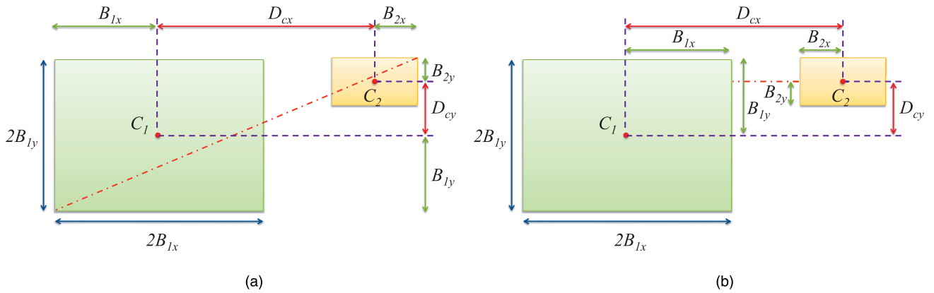
Fig. 11. Computing the maximum and minimum distance between two AABs. The equations are similar to the point-AABB distance case. See (13)-(20). (a) Maximum distance. (b) Minimum distance.
