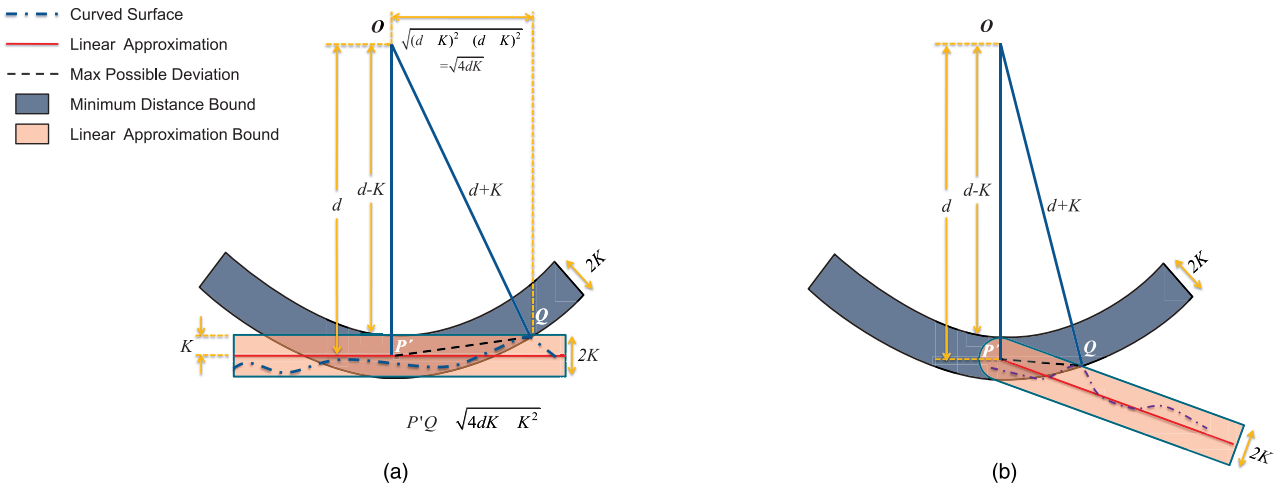
Fig. 9. Illustration to evaluate the bound for the computed closest point location when the closest point on the plane lies either (a) inside or (b) on the edge of the triangle approximating the surface. (a) Case 1. (b) Case 2.
