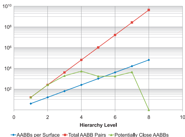
Fig. 12. Plot showing the actual number of AAB pairs compared during a typical minimum distance computation. The number of pairs being tested in parallel remains almost constant after level 3 of the hierarchy. Note logarithmic scale used for the y -axis.
