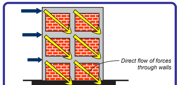
Figure 5: Avoiding open ground storey problem – continuity of walls in ground storey is preferred.
