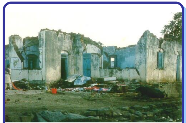
(a) Building with no horizontal lintel band: collapse of roof and walls
