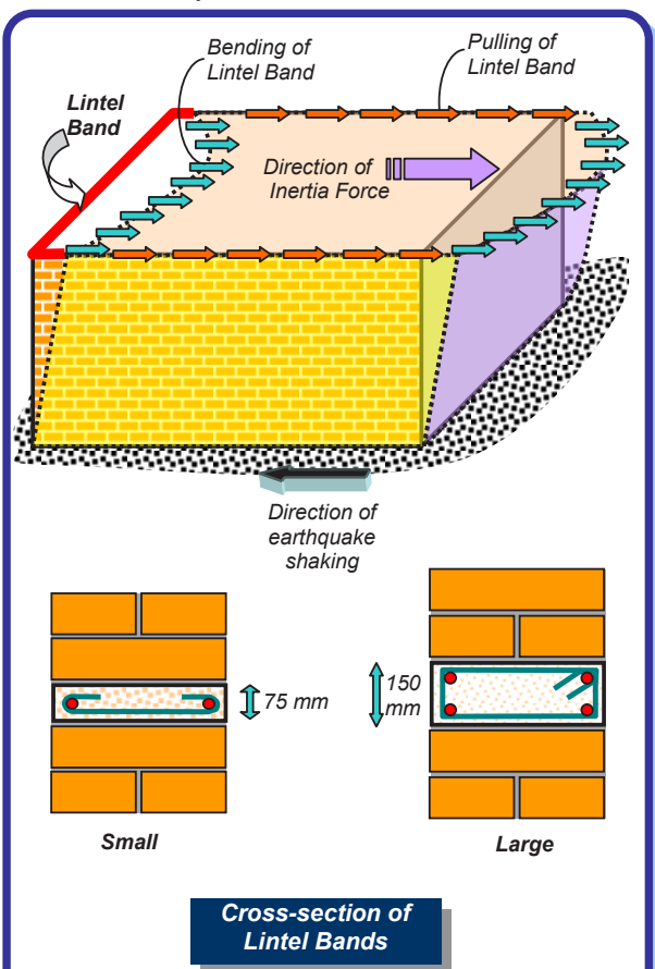
Figure 3: Bending and pulling in lintel bands – Bands must be capable of resisting these.
