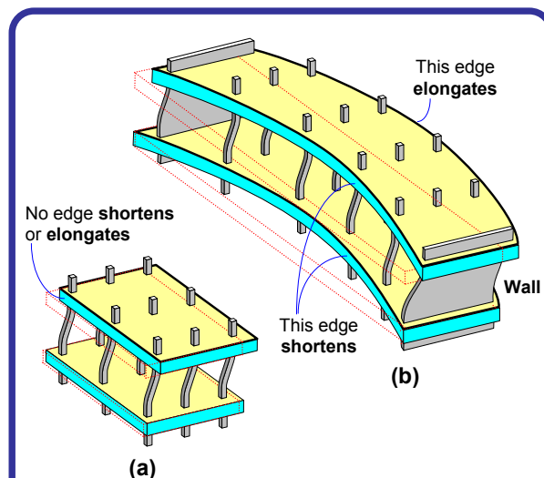
Figure 2: In-plane deformation in horizontal diaphragms – (a) absent, if plan aspect ratio is up to 3, and (b) present, if plan aspect ratio exceeds 5
