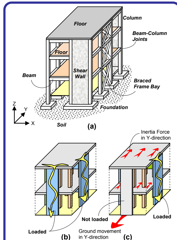
Figure 1: Load paths for different load actions – (a) key structural elements constituting load paths, (b) vertical load paths, and (c) lateral load paths
