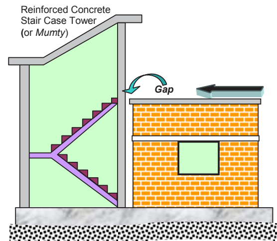
(b) Building with separated staircase
