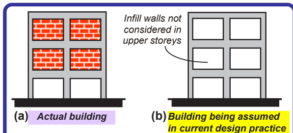
Figure 4: Open ground storey building – assumptions made in current design practice are not consistent with the actual structure.
