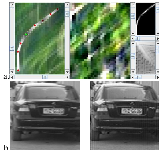
Fig. 6 a. User interface for drawing an estimate PSF, b. and c. Input and output images of inverse filtering
