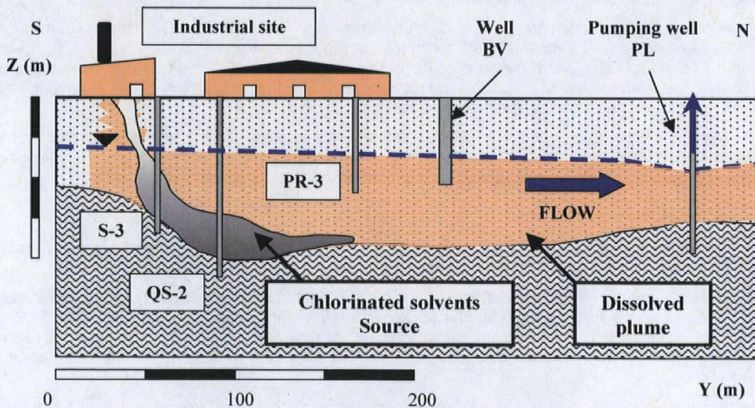
Figure 2 : South – North section of the site
