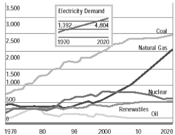
Fig. 3. Electricity generation by fuel (billions of kilowatt-hours).
