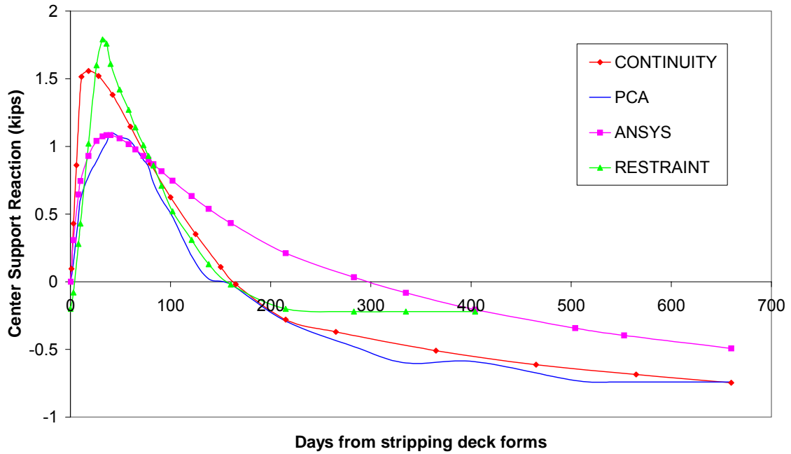
Figure 58. Verification with Beam1/2.
