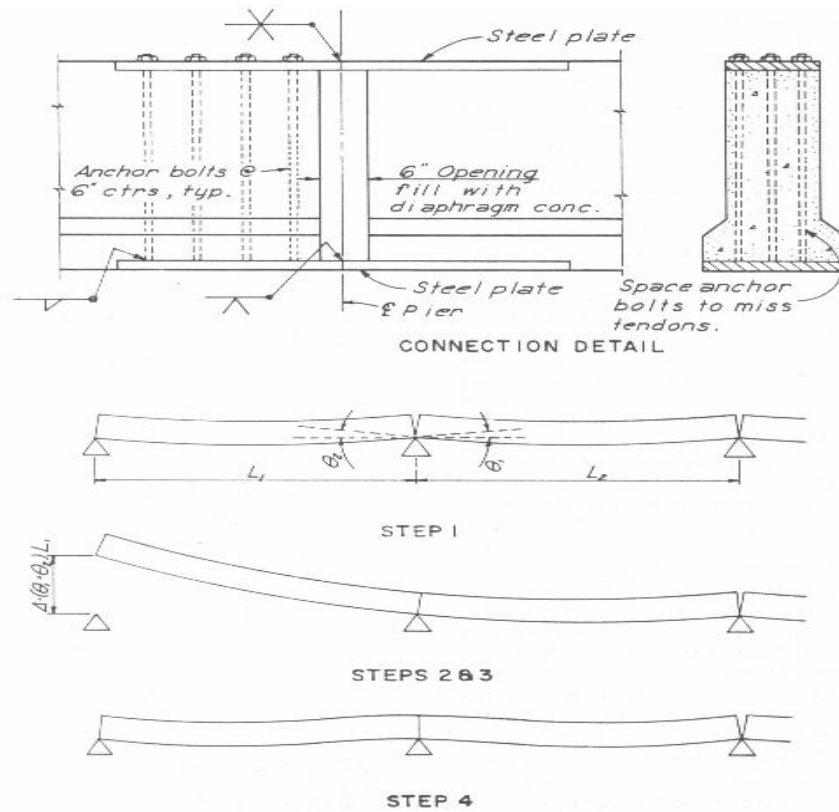
Figure 4. Bishop's post-tensioning method.
