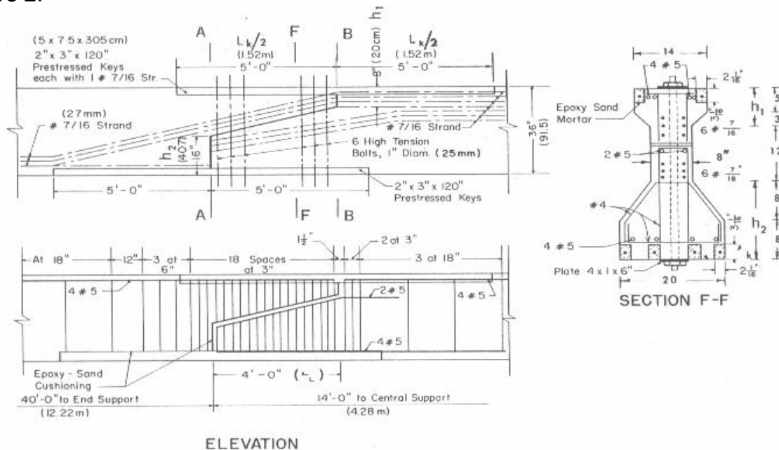
Figure 2. Keyed scarf connection. (12)
