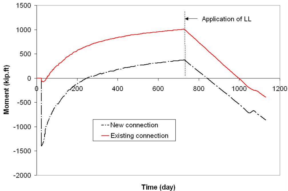
Figure 95. Comparison of support moments ( C=2.0 , \epsilon=600 \times 10^{-6} in/in).
