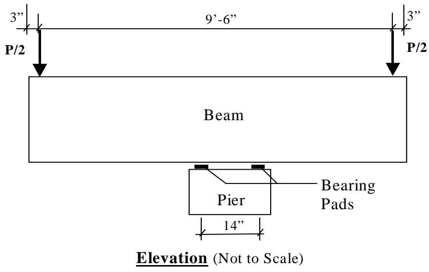
Figure 71. Test setup of beams 1, 2, 1R and 2D.
