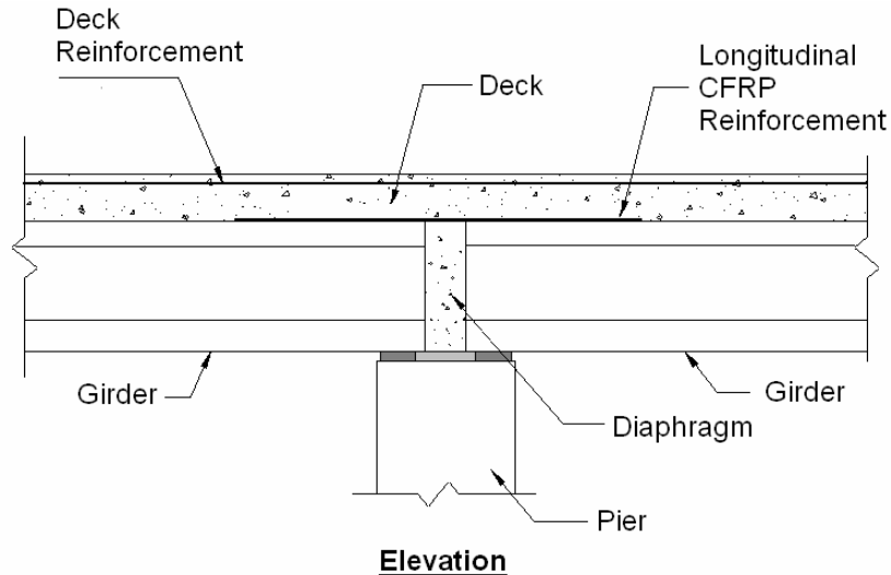
Figure 68. New connection.
