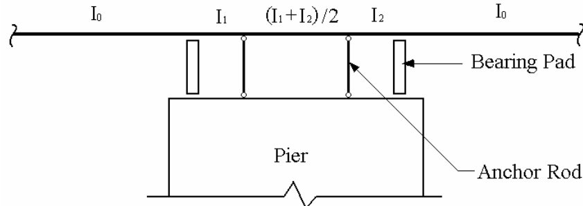
Figure 35. Model 2 support detail.
