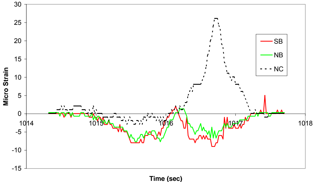
Figure 20. Readings of bottom gages when a truck is passing over.
