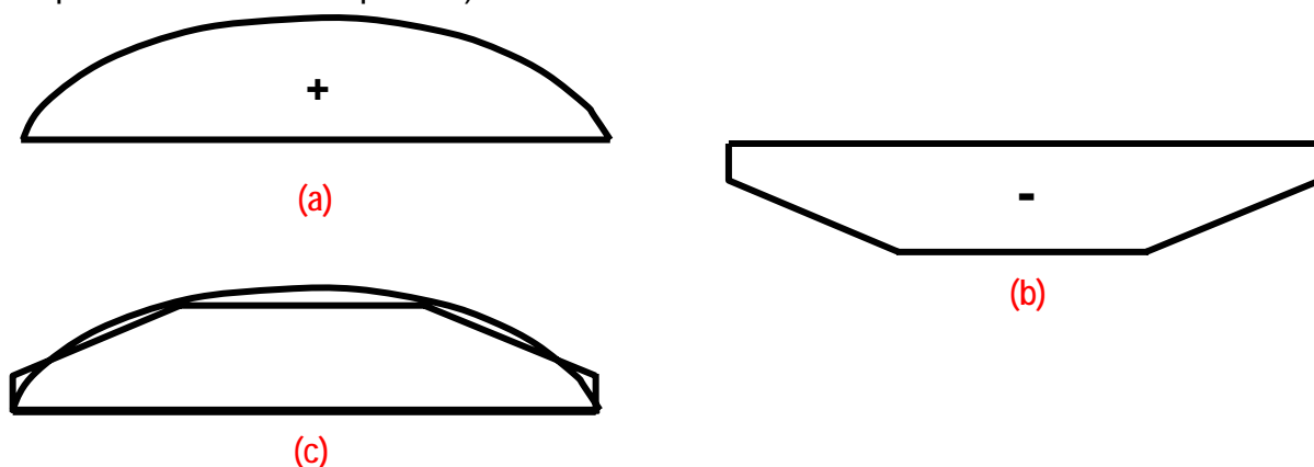
Figure 44. Moment diagrams due to dead load and prestressing forces, and net result.
