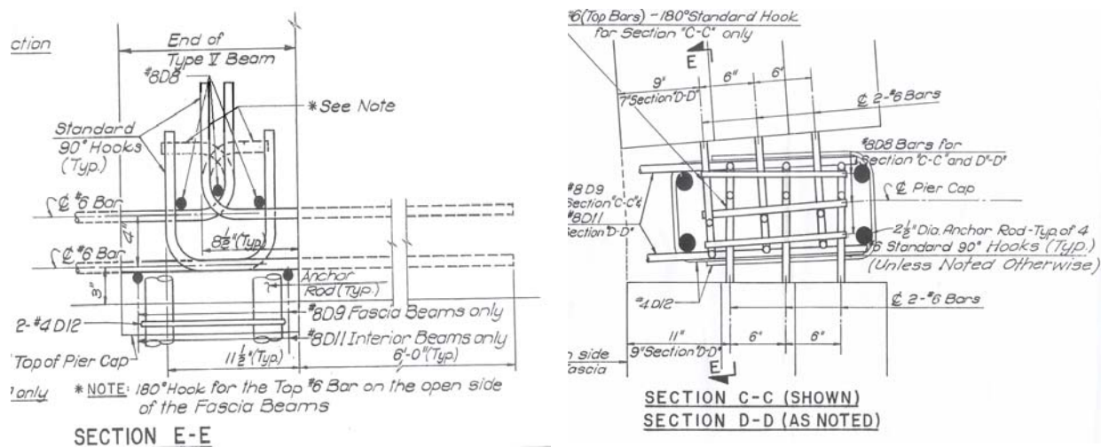
(a) Elevation
