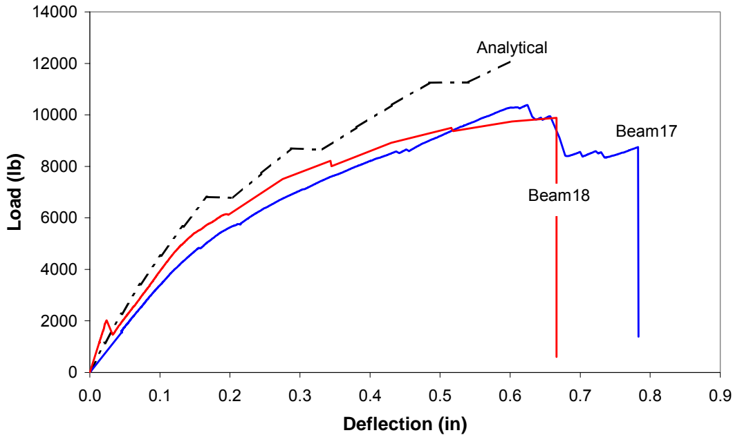
Figure 90. Analytical and test results of beams 17 and 18.
