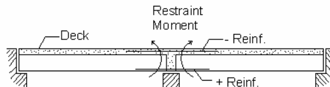
b) Formation of restraint moment
