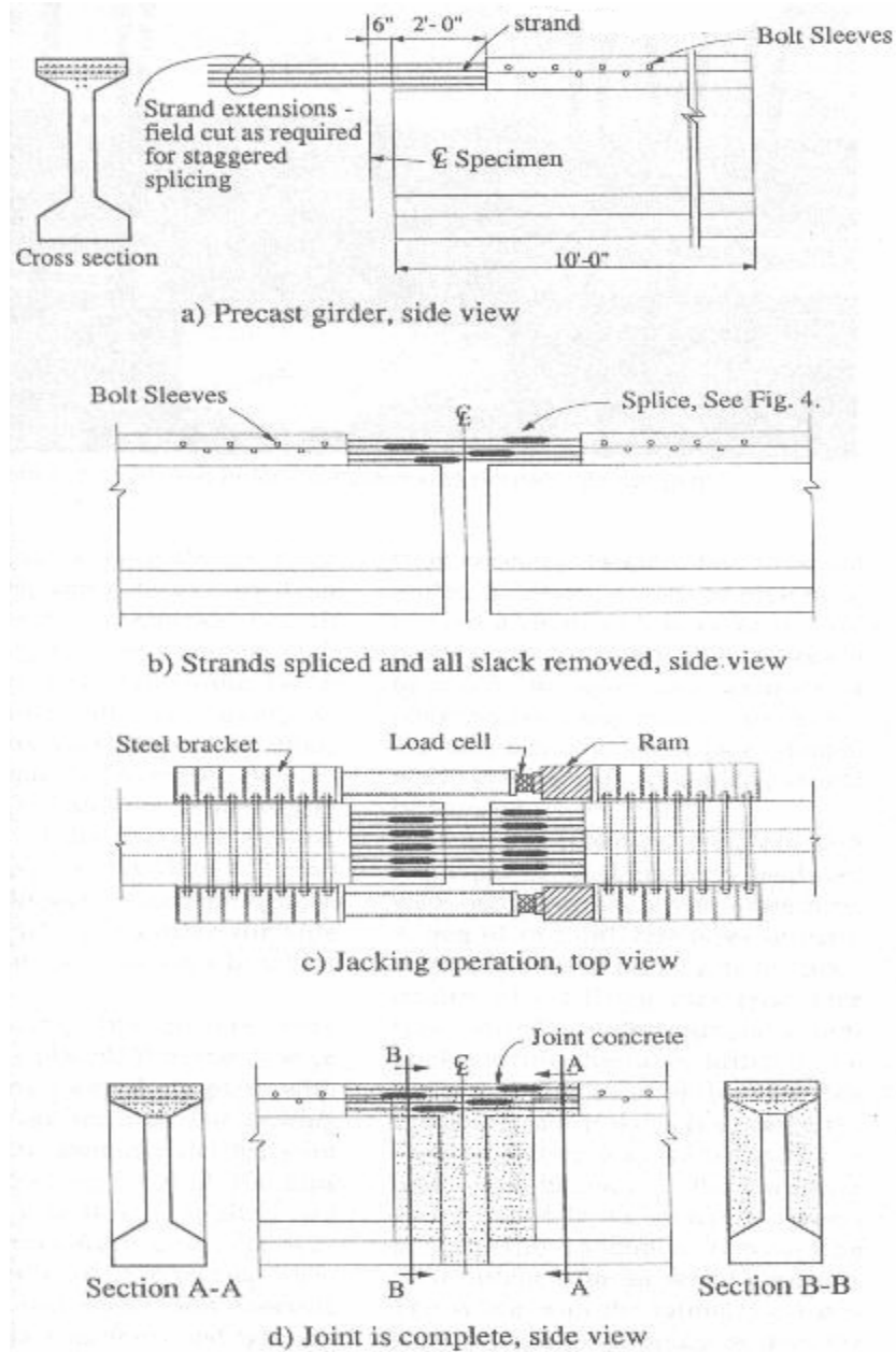
Figure 5. Post-tensioning of pre-strands.
