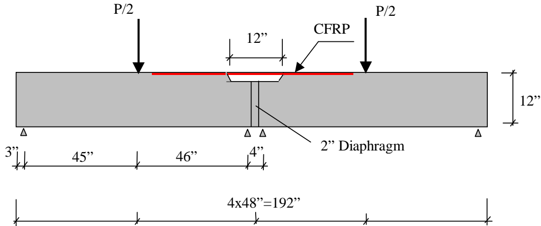
Figure 78. Beam 5 setup.
