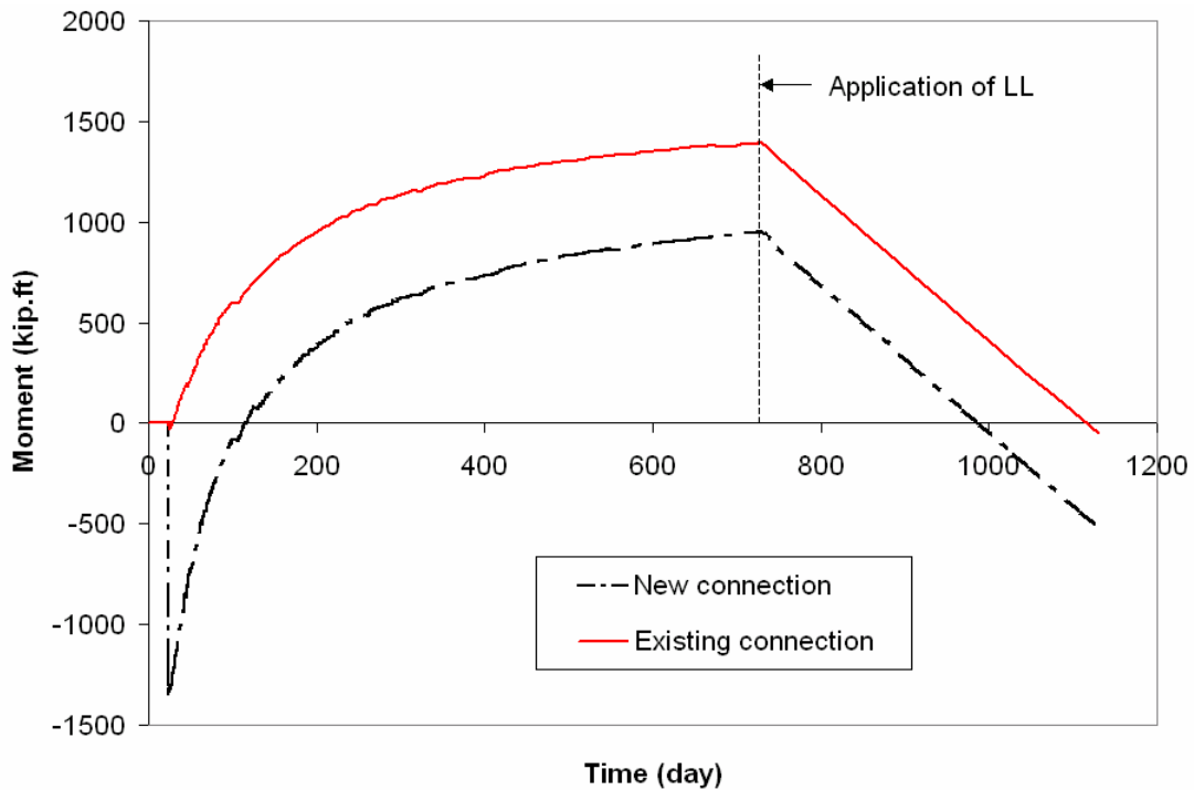
Figure 93. Comparison of support moments ( C=3.25 , \epsilon=600\times 10^{-6} in/in).
