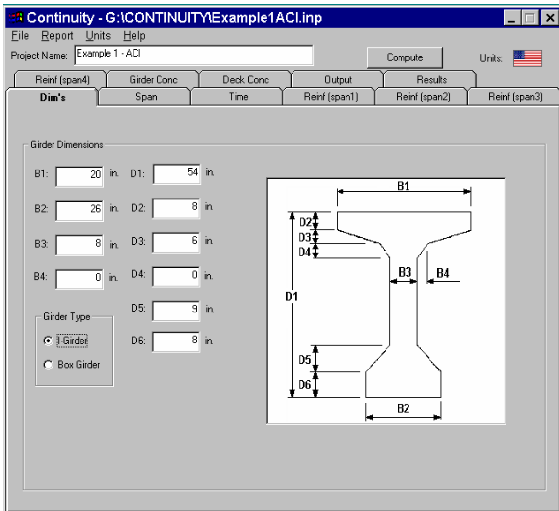
Figure 59. I-girder dimensions.
