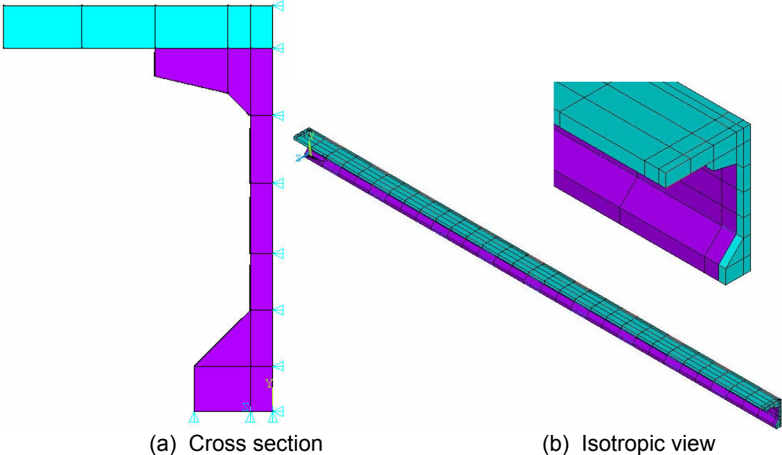
Figure 47. Finite element model.
