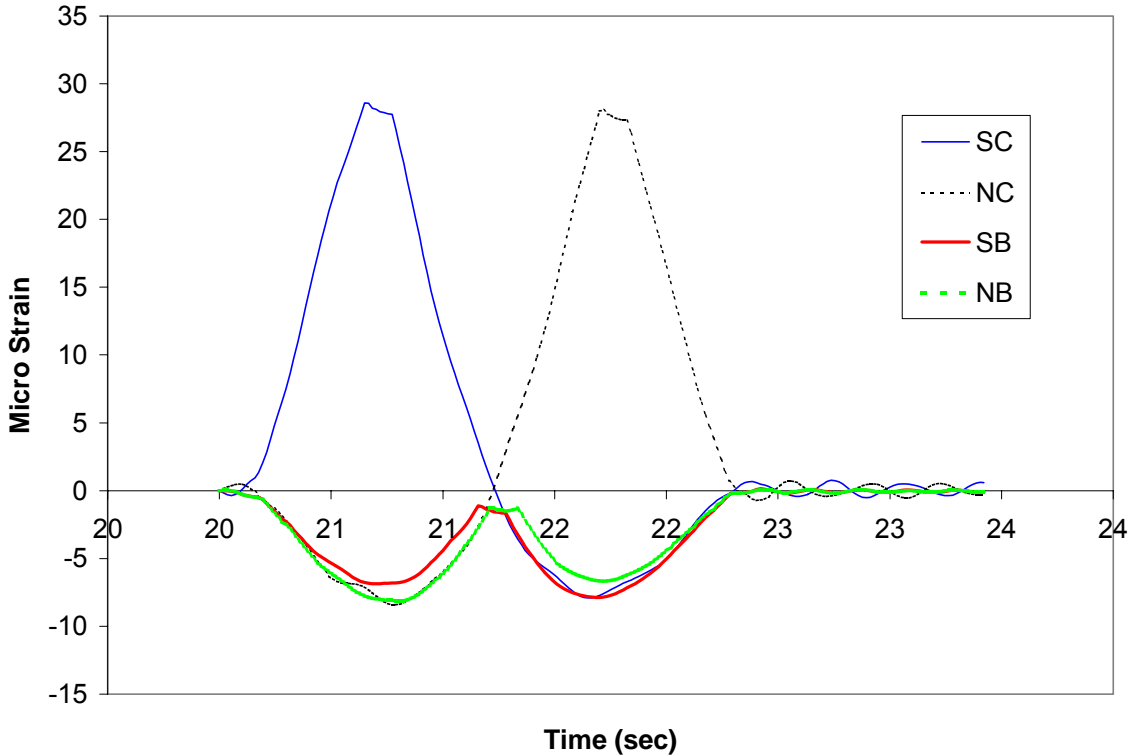
Figure 21. Theoretical strains at mid-spans and girder ends.
