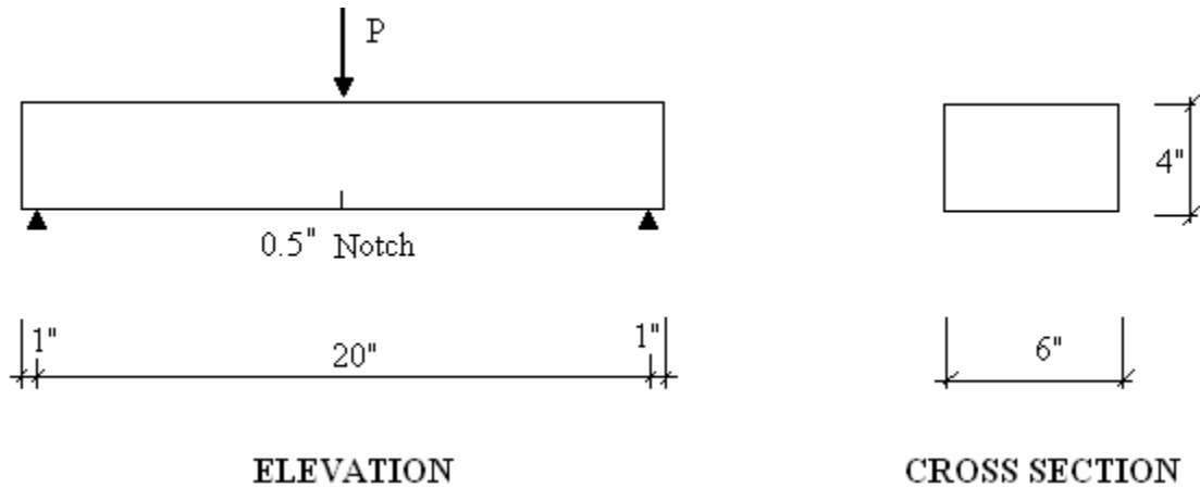
(a) Beam 6
