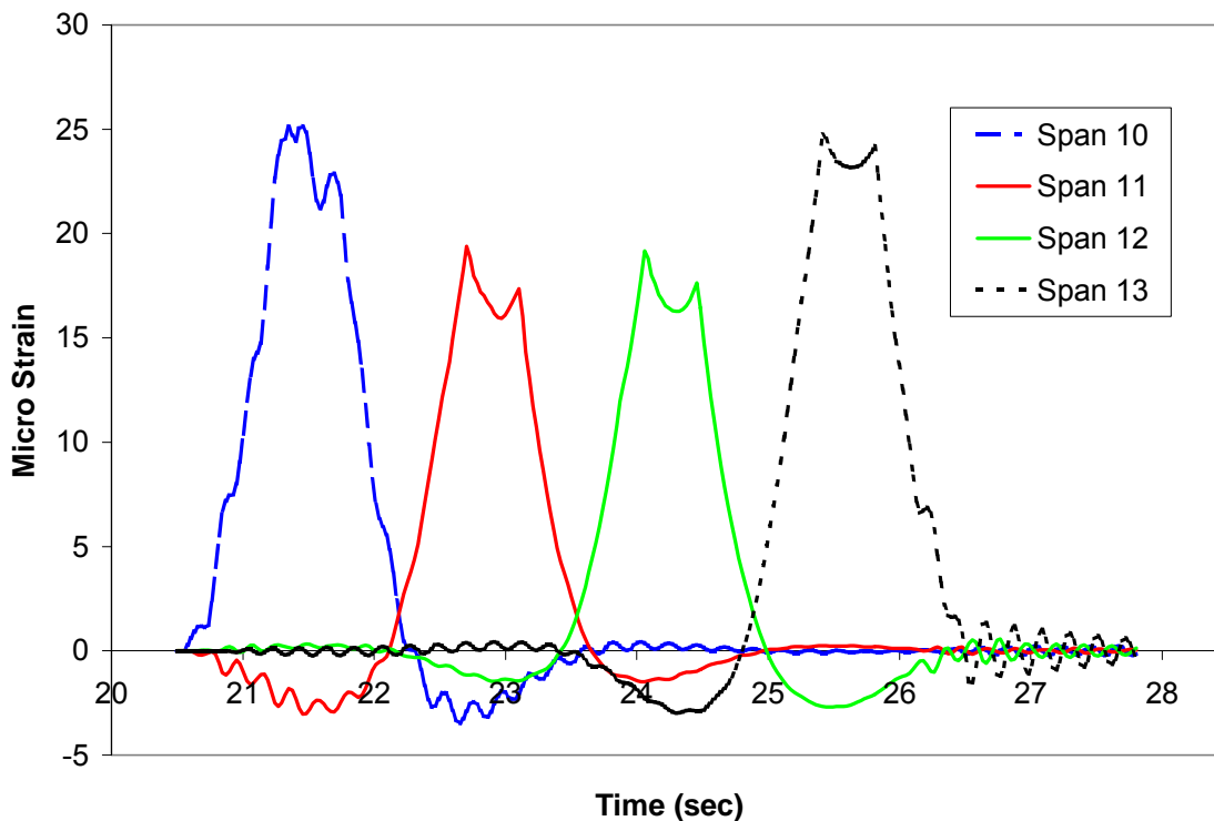
Figure 37. Analytical mid-span strains from model 3.
