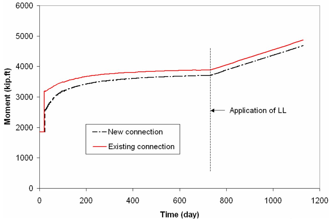
Figure 92. Comparison of midspan moments ( C=3.25 , \epsilon=600 \times 10^{-6} in/in).
