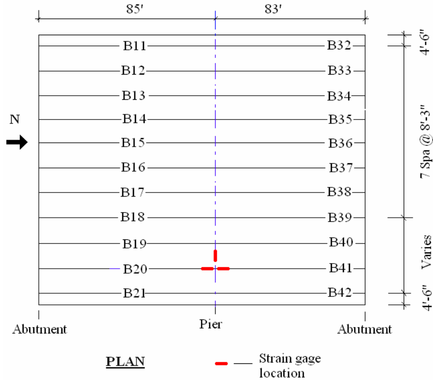
Figure 9. Layout and instrumentation of I-287 NB over Skyline Dr, Mahwah, NJ.
