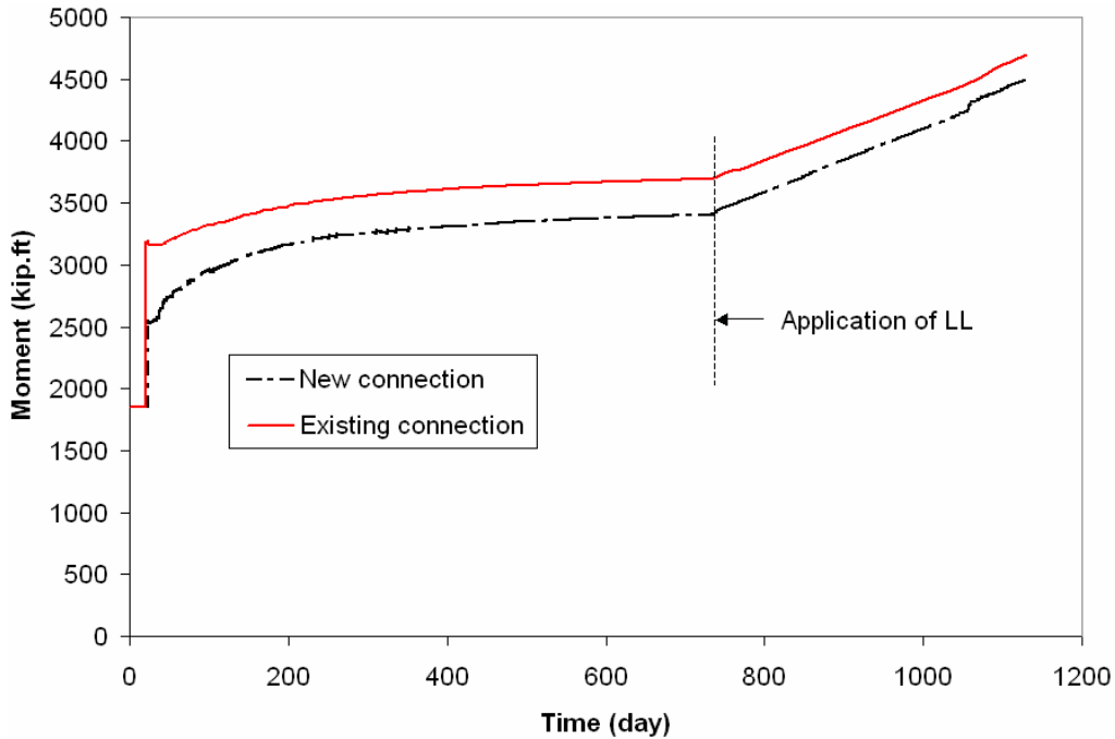
Figure 94. Comparison of midspan moments ( C=2.0 , \epsilon=600 \times 10^{-6} in/in).
