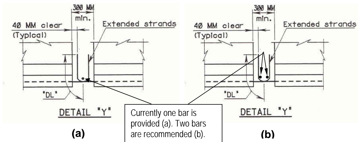
Figure 45. Positive restraint moment connection (New Jersey)
