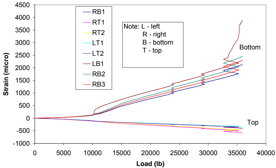
(b) Strain in rebar
