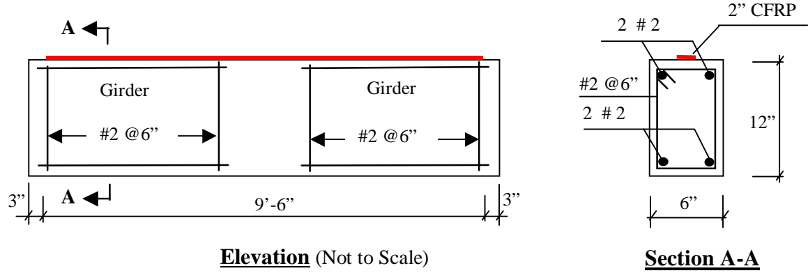
Figure 70. Details of beams 2, 1R and 2D.
