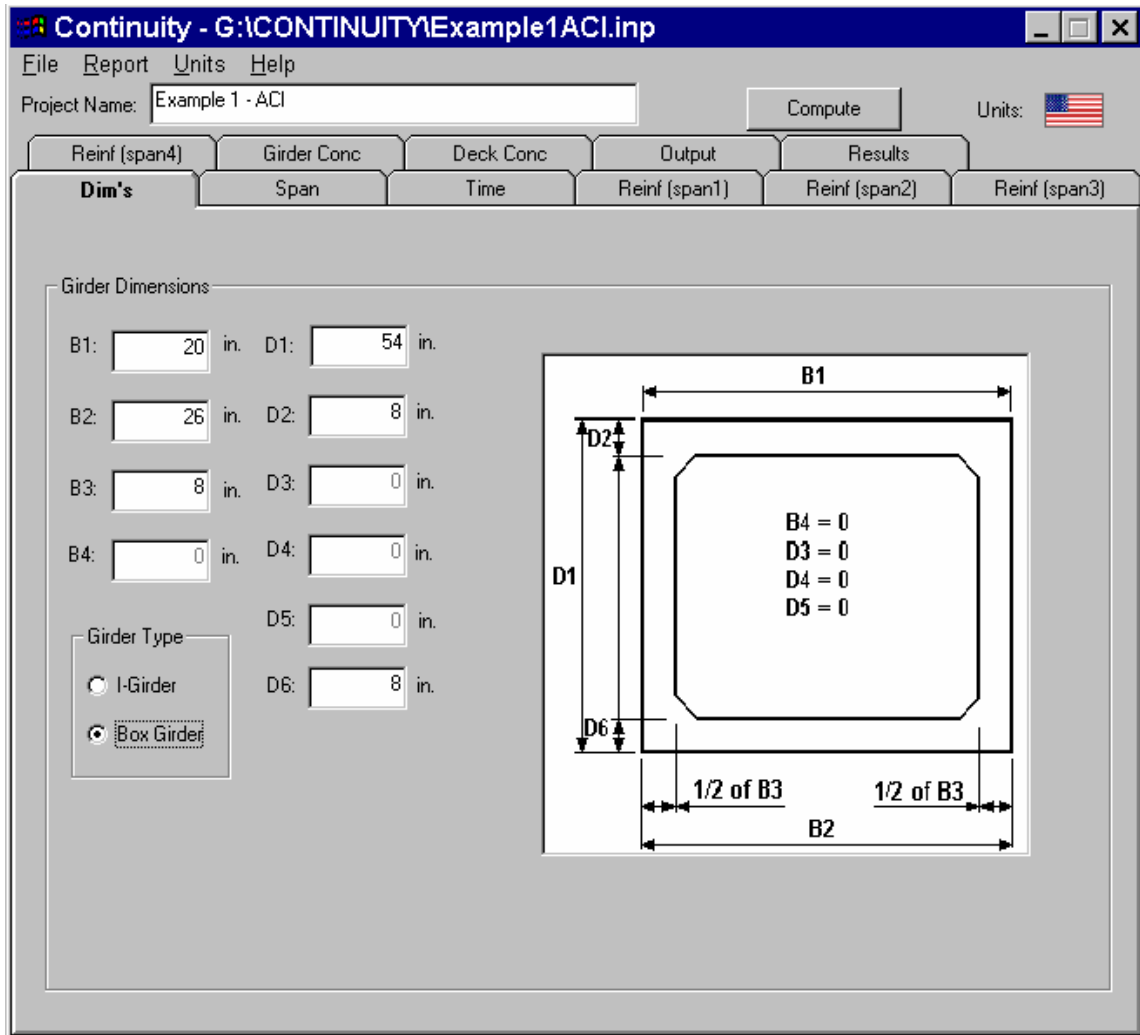
Figure 60. Box-girder dimensions.
