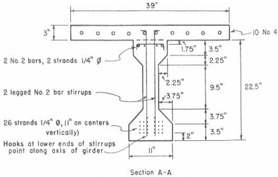
Figure 48. Cross section of PCA specimens.
