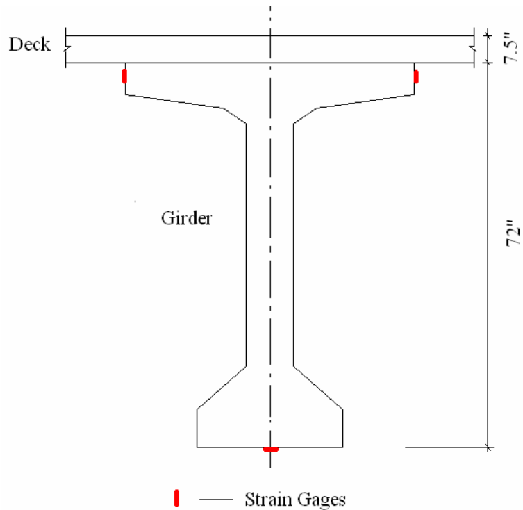
Figure 18. Instrumentation on girders.
