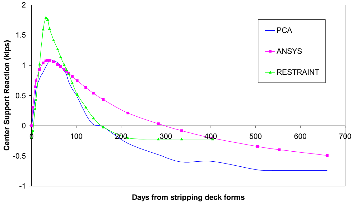
Figure 50. Comparison of central support reaction of beam 1/2.
