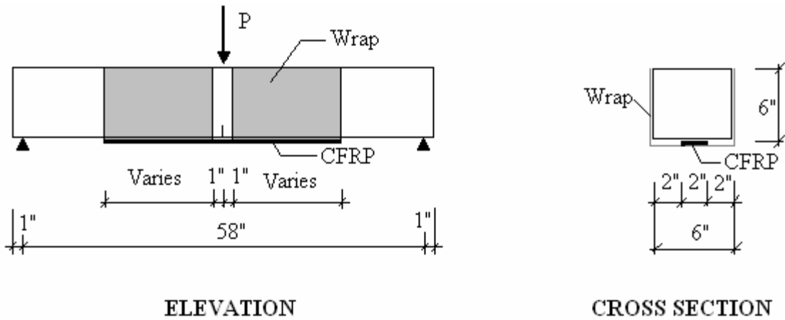
(b) Beams 15 and 16 with bonding length of 18" and 24", respectively.
