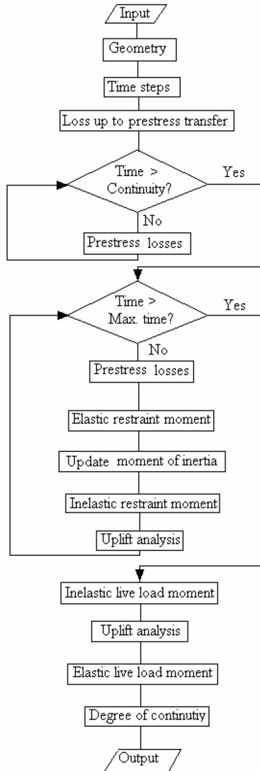
Figure 56. Flow chart of CONTINUITY.
