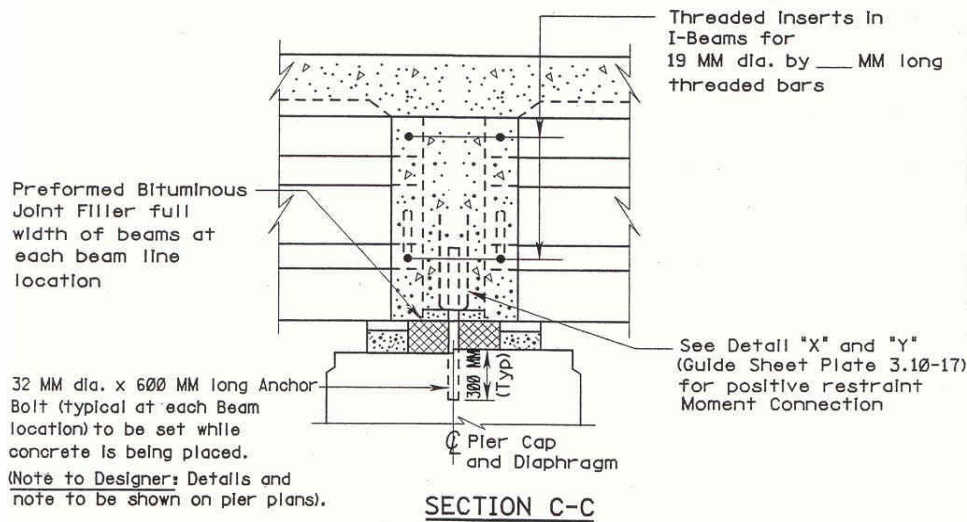
Figure 42. Continuity joint details (New Jersey).
