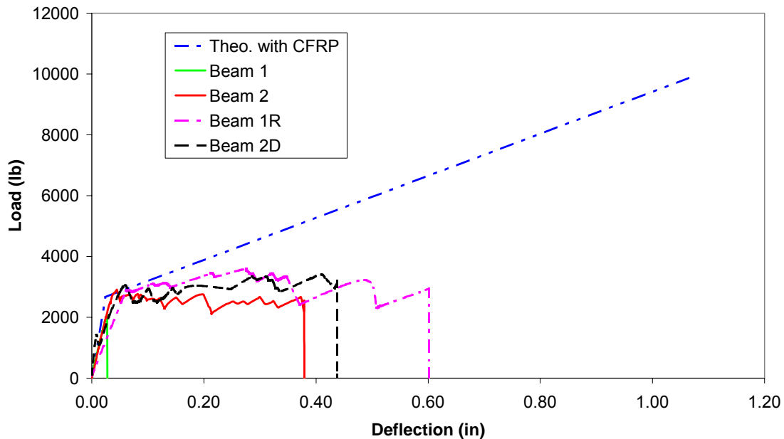
Figure 73. Test results of beams 1, 2, 1R and 2D.
