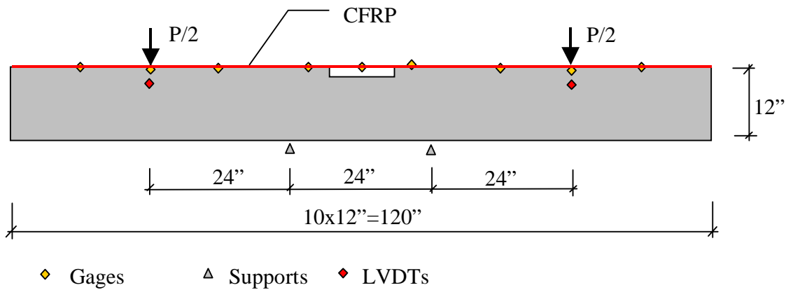
Figure 75. Test setup of beams 3 and 4.
