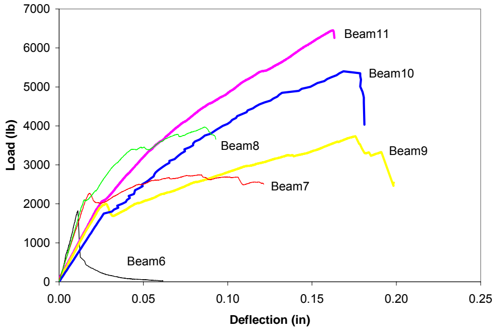
Figure 82. Load-deflection of beams 6 to 11.
