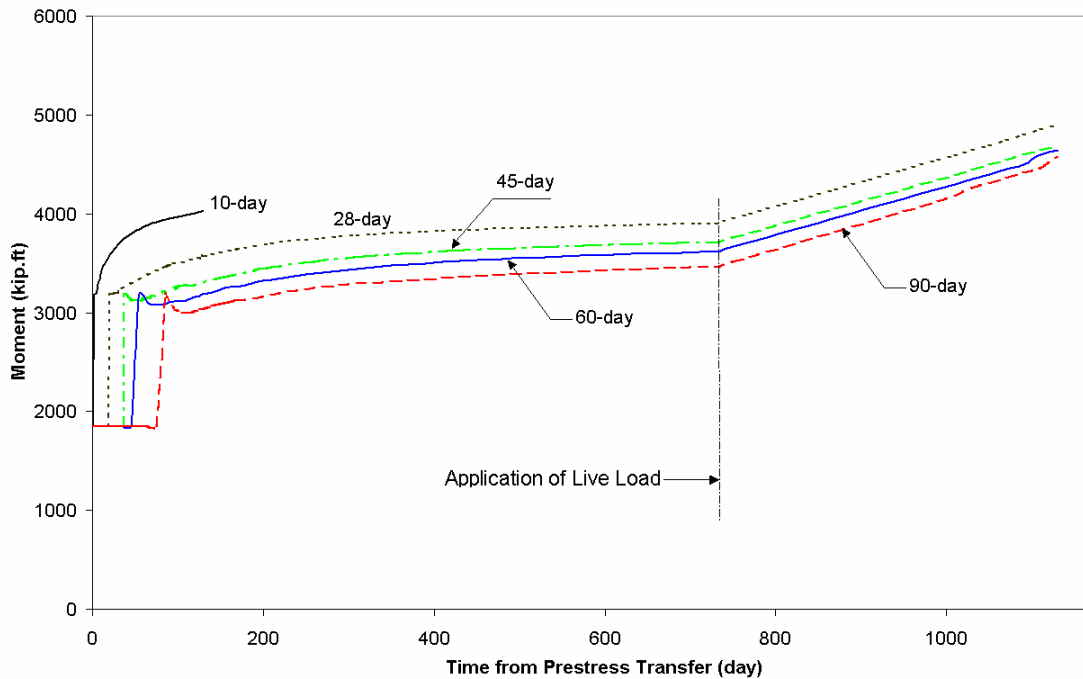
Figure 52. Variation of mid-span moment with girder age at deck casting.
