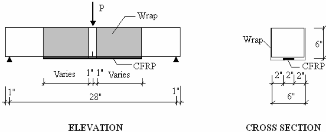
(a) Beams 12 to 14 with bonding length of 6", 9" and 12", respectively.
