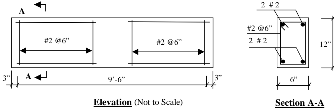
Figure 69. Beam 1 details.
