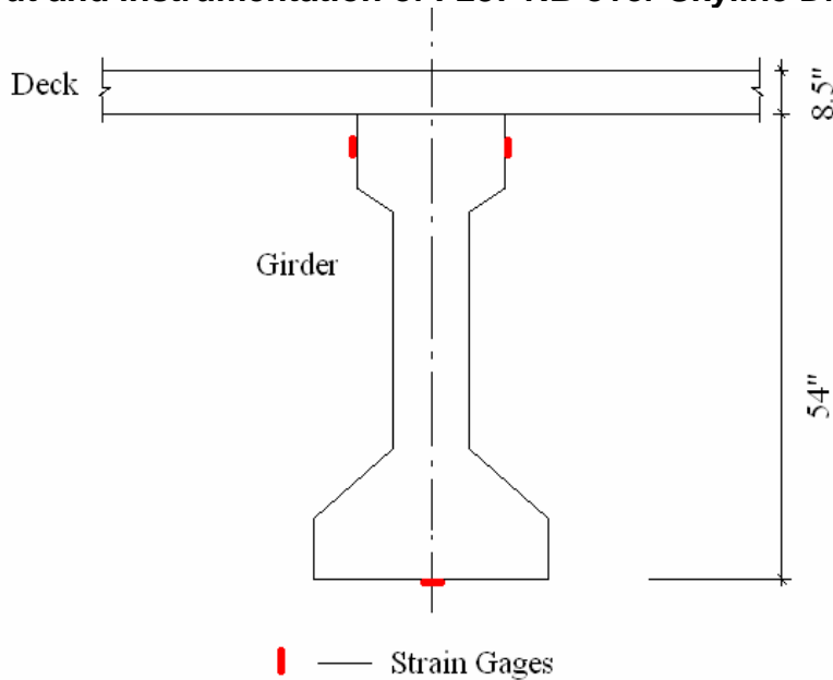
Figure 9. Layout and instrumentation of I-287 NB over Skyline Dr, Mahwah, NJ.
