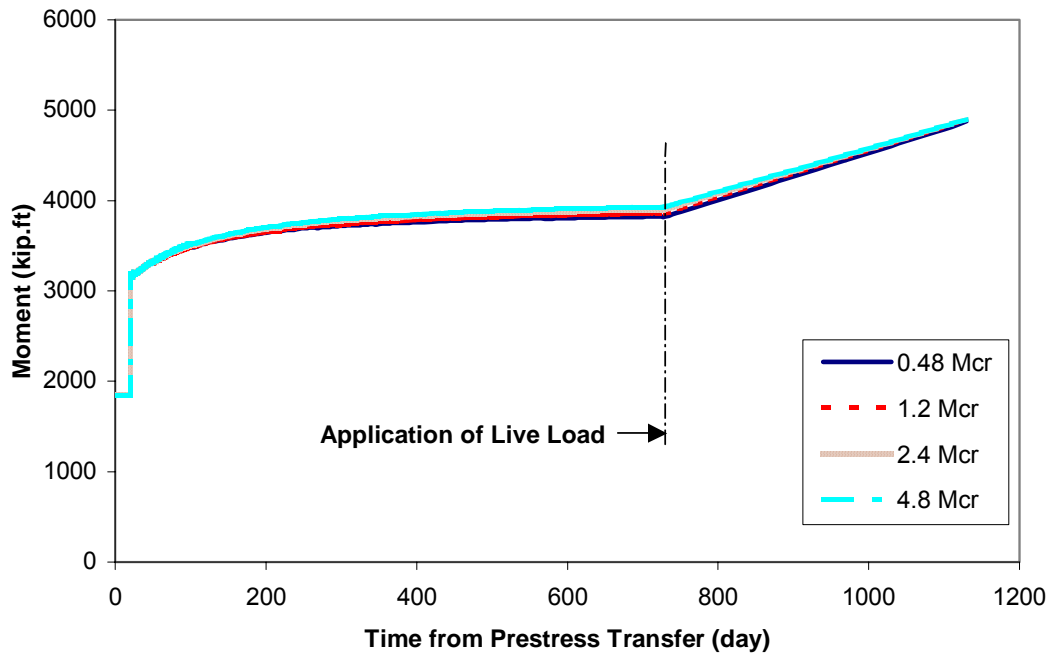
Figure 55. Variation of mid-span moment with amount of +M reinforcement.
