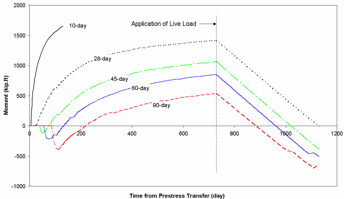
Figure 53. Variation of central support moment with girder age at deck casting.
