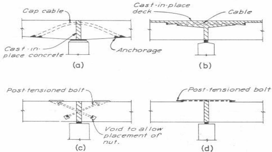
Figure 3. Partial post-tensioned connections.
