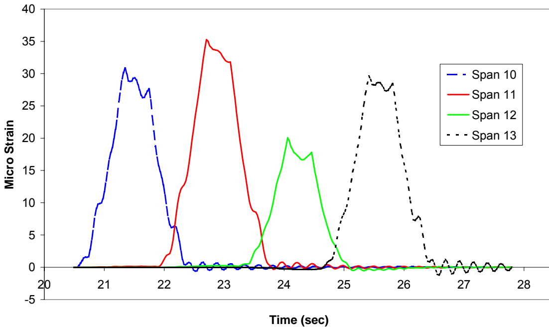
Figure 36. Analytical mid-span strains from model 2.
