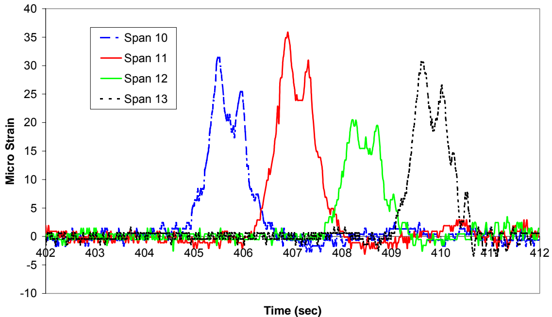
Figure 31. Strain history of mid-span gages from test.
