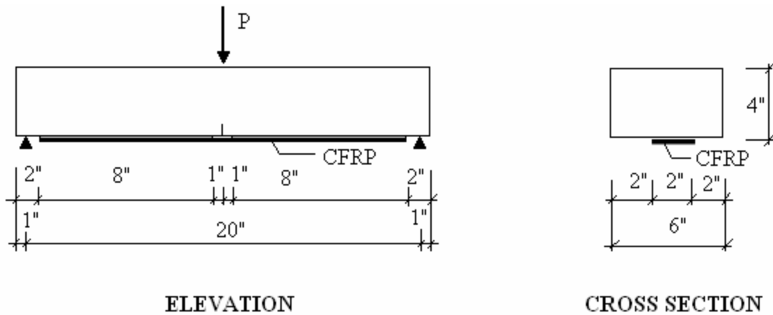
(b) Beams 7 and 8
