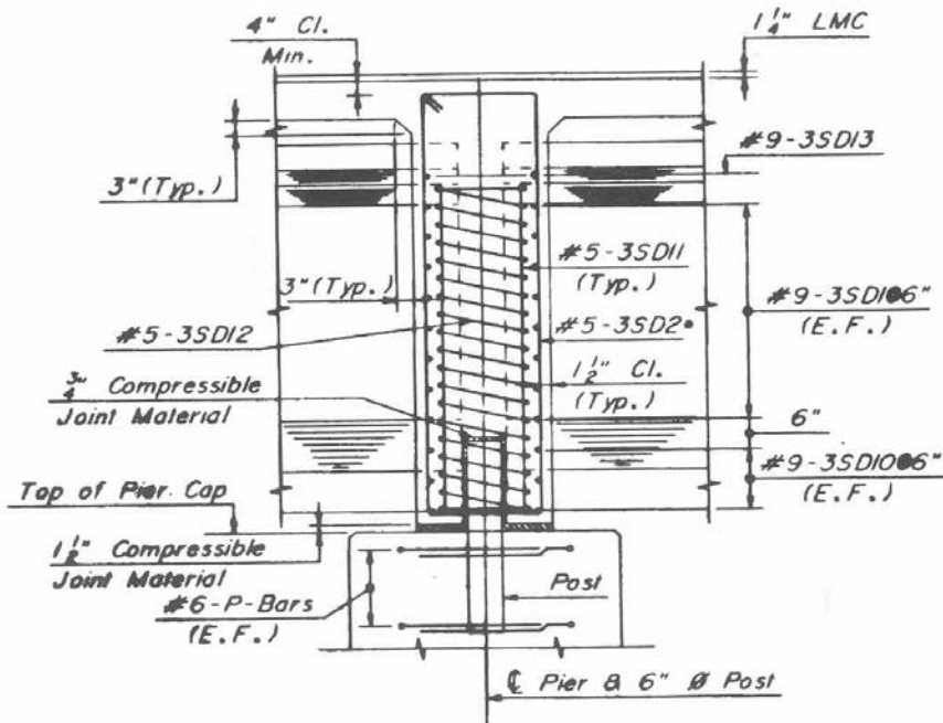
(b) Section
