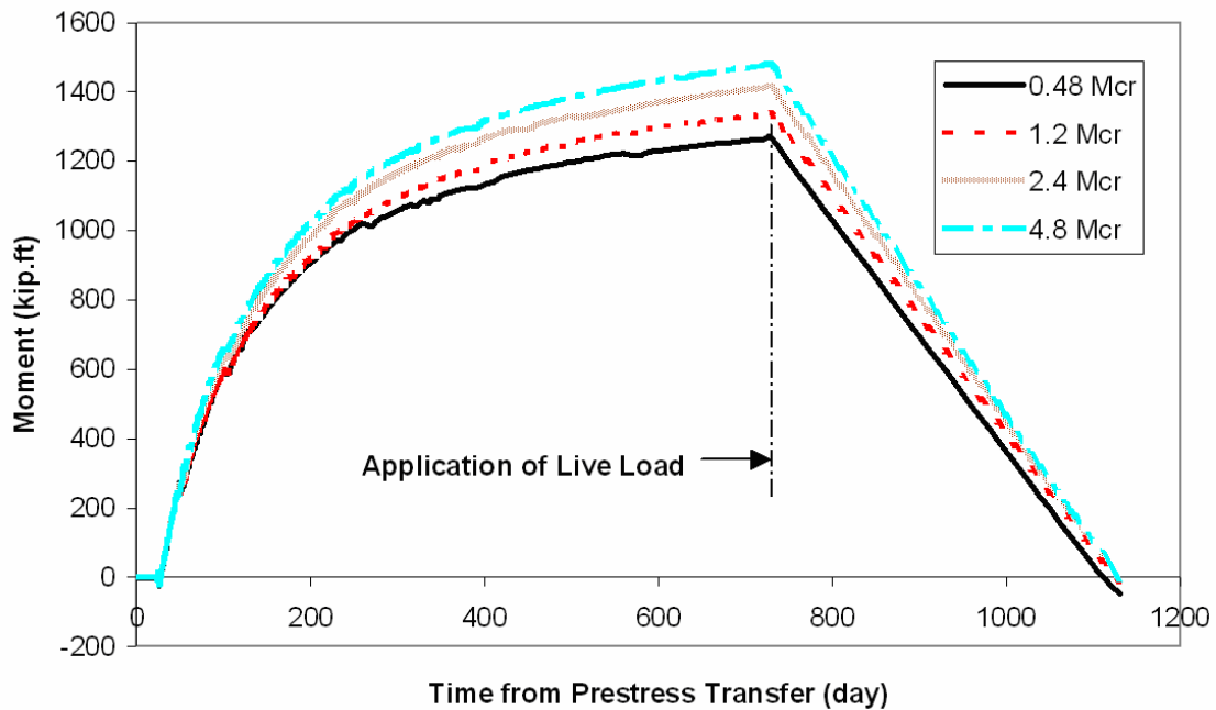
Figure 54. Variation of support moment with amount of +M reinforcement.
