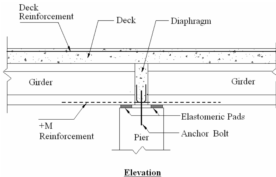
Figure 8. Support details.
