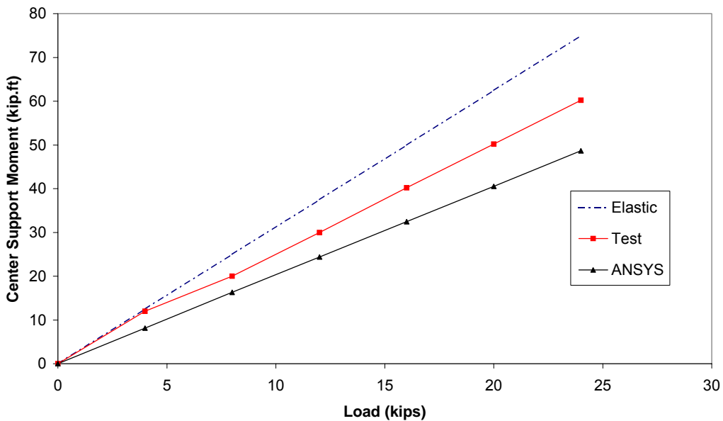
(c) Girder age of 684 days.
