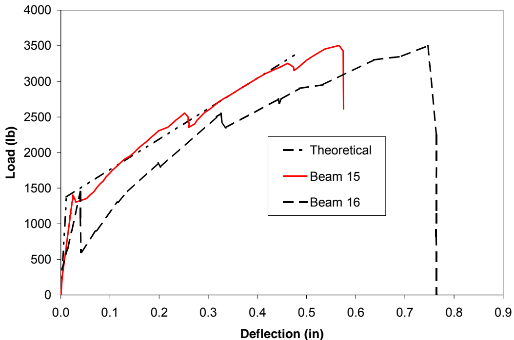
Figure 87. Load-deflection curves for beams 15&16 with diff. bonding length.
