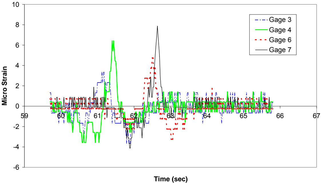
Figure 30. Bottom gages near supports.
