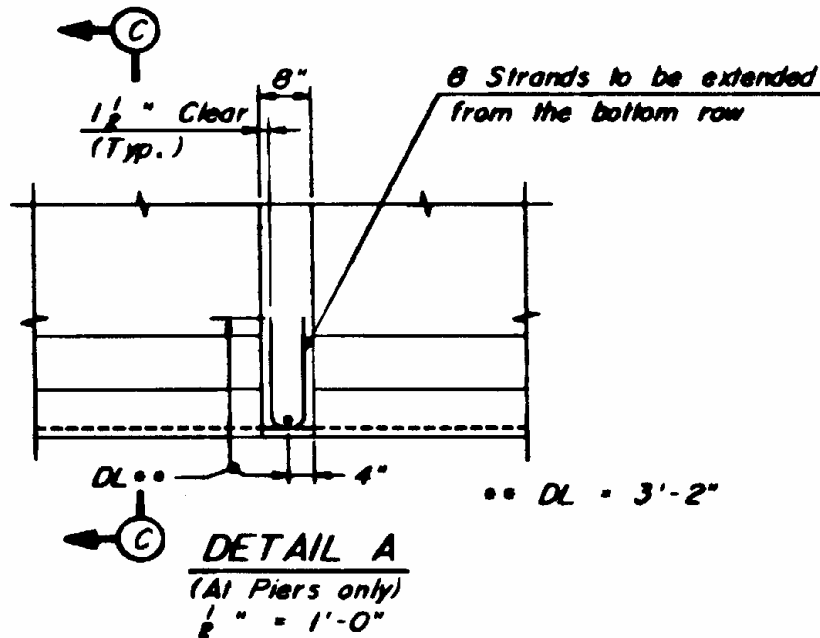
Figure 15. Positive moment connection over piers (from design drawing).
