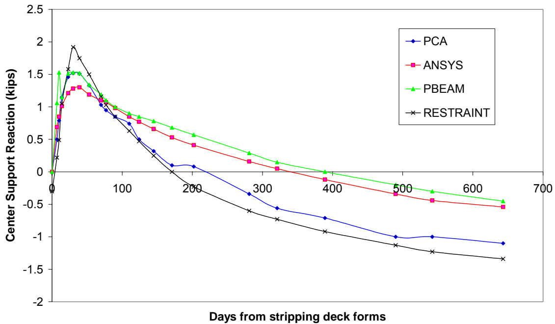
Figure 49. Comparison of central support reaction of beam3 and 4.
