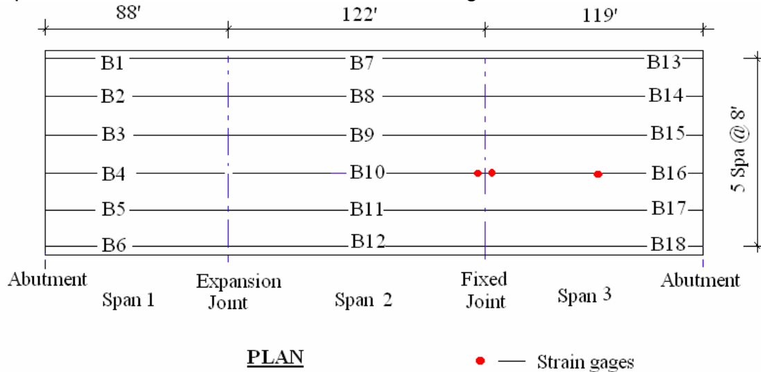
Figure 17. Instrumentation on I-287 NB over Darlington Ave, Mahwah, NJ.
