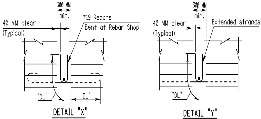
(a) New Jersey
