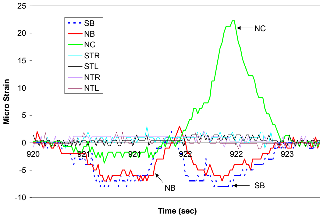
Figure 19. Typical readings (all gages).
