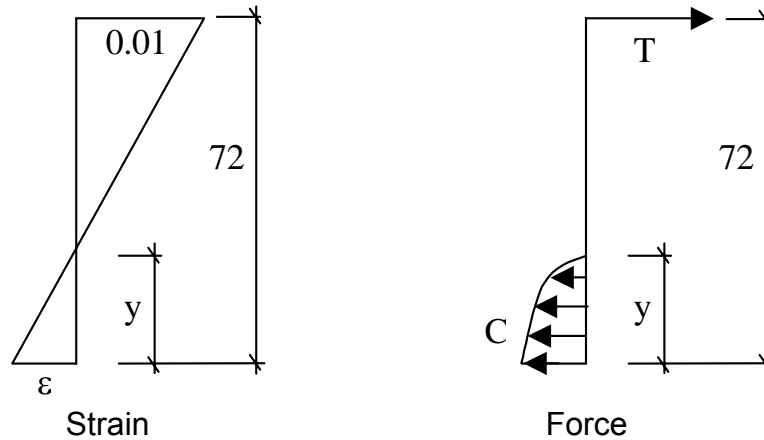
Figure 91. Cross sectional analysis.
