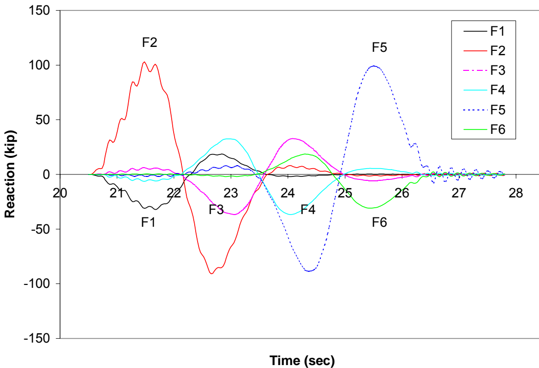
Figure 34. Reaction in anchor rods from model 1.
