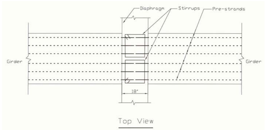
Figure 46. Wider continuity connection similar to that used by TNDOT.
