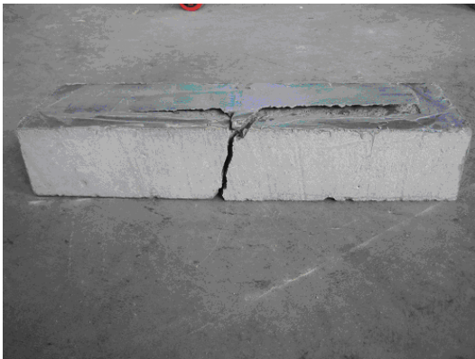
(a) & (b) Debonding of CFRP without wrap (beam7).
