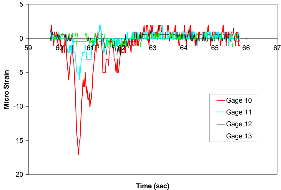
Figure 29. Girder top gages near supports.
