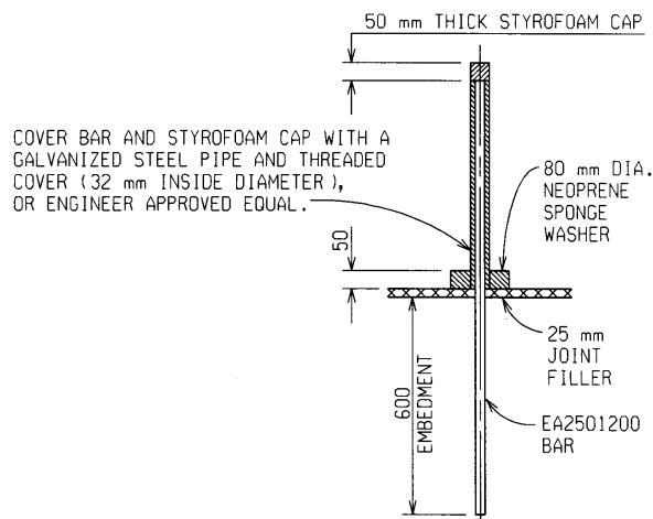
Figure 43. Bar sheath and Styrofoam cap (Michigan).
