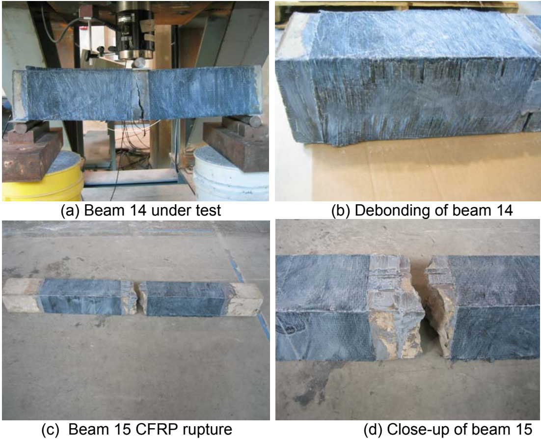
Figure 85. Test setup and failure modes of beams 12 to 16.
