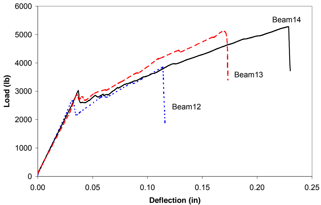
Figure 86. Load-deflection curves for beams 12-14 with diff. bonding length.
