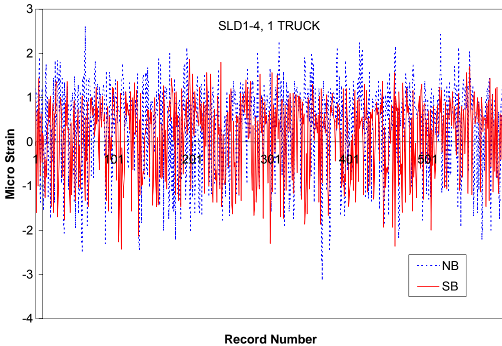
(b) Response of Gages NB and SB when There Was A Truck Passing.
