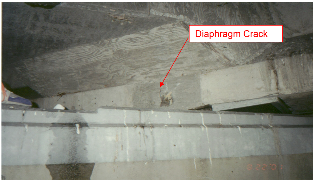
Figure 11. Diaphragm bottom crack, I-287 NB over Skyline Drive.
