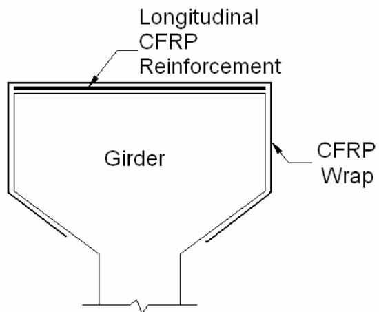
CFRP Detail
