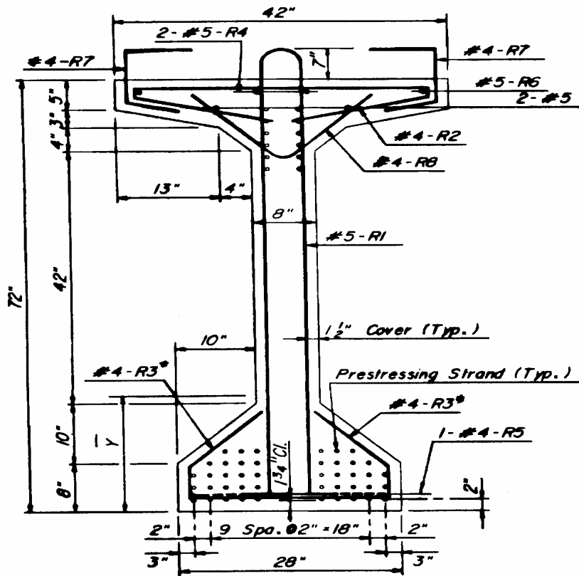
Figure 13. Girder cross section (from design drawing).
