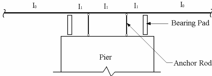
Figure 33. Model 1 support detail.
