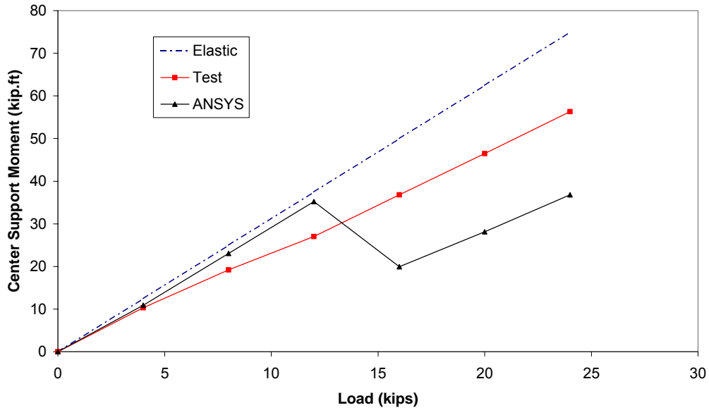
(b) Girder age of 55 days.
