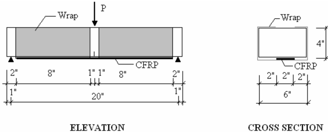
(c) Beams 9 to 11
