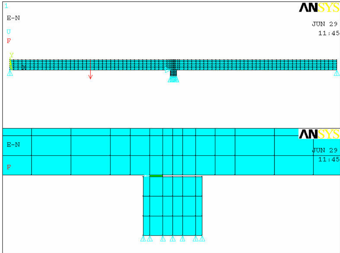
Figure 38. 2-D finite element model of a 2-span bridge.
