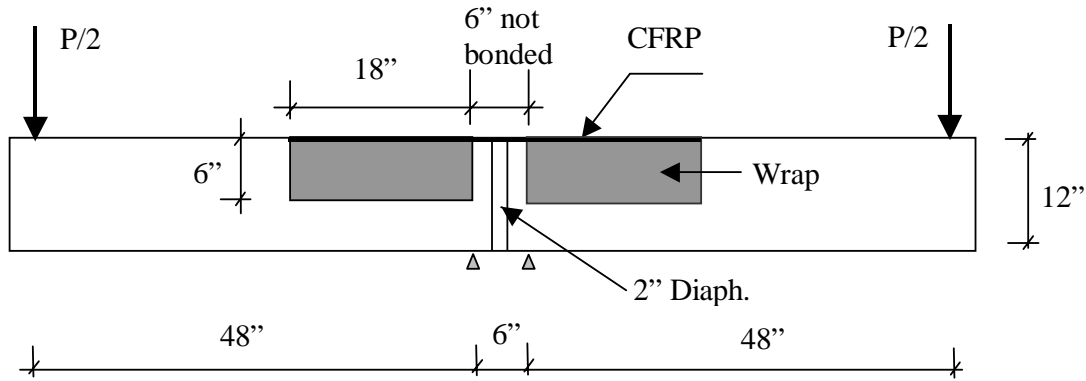
Figure 88. Detail of beams 17 and 18.
