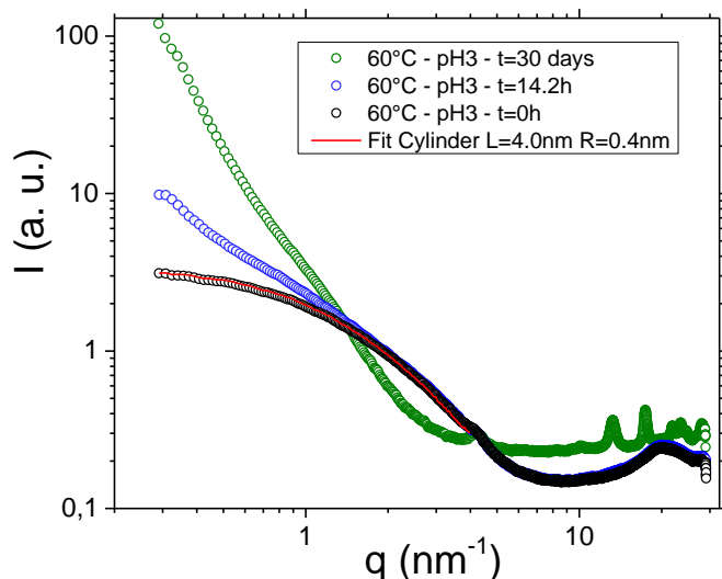
Figure 4. In-situ SWAXS measurements kinetic of thorite formation at pH = 3 at 60°C. Description of STEP I, II and III. At low q values ( < 4 \text{ nm}^{-1} ), experiment at t_0 is fitted with a cylinder form factor model, P(q) .
