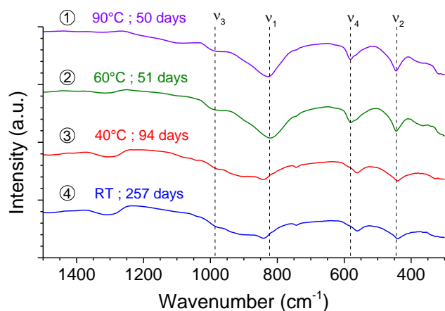
Figure 1. PXRD patterns (a), Raman (b) and infrared spectra (c) obtained for samples prepared with starting silicate and thorium(IV) concentrations of 0.21 \text{ mol}\cdot\text{L}^{-1} in nitric reactive media at initial pH = 3 at 90°C for 50 days (1), 60°C for 51 days (2), 40°C for 94 days (3) and at room temperature for 257 days (4). Characteristic XRD lines of \text{ThO}_2 and \text{ThSiO}_4 were extracted from references 40 and 7 , respectively.
