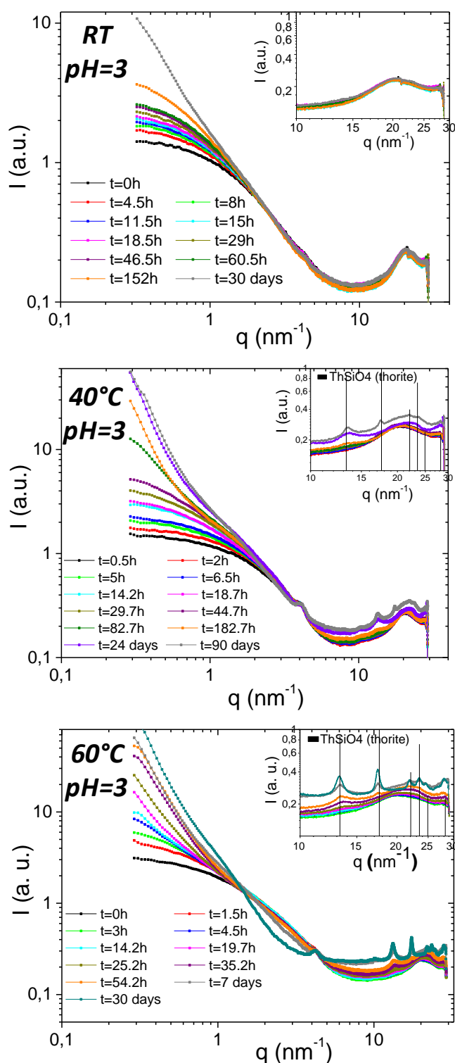
Figure 3. In-situ SWAXS measurements kinetics at room temperature (RT), 40^\circ\text{C} and 60^\circ\text{C} for \text{pH} = 3 . The inset graphics refer to a focus in the q range from 10 \text{ nm}^{-1} to 30 \text{ nm}^{-1} .
