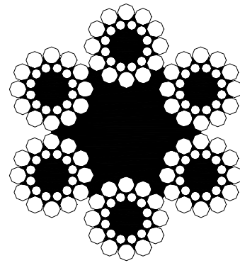
FIGURE 31. Type III, marine (cables), class 3, 6 by 24, (mooring lines), construction 3, (Seale).
