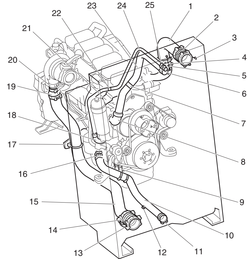
1.3 m 2 radiator for the DC13
