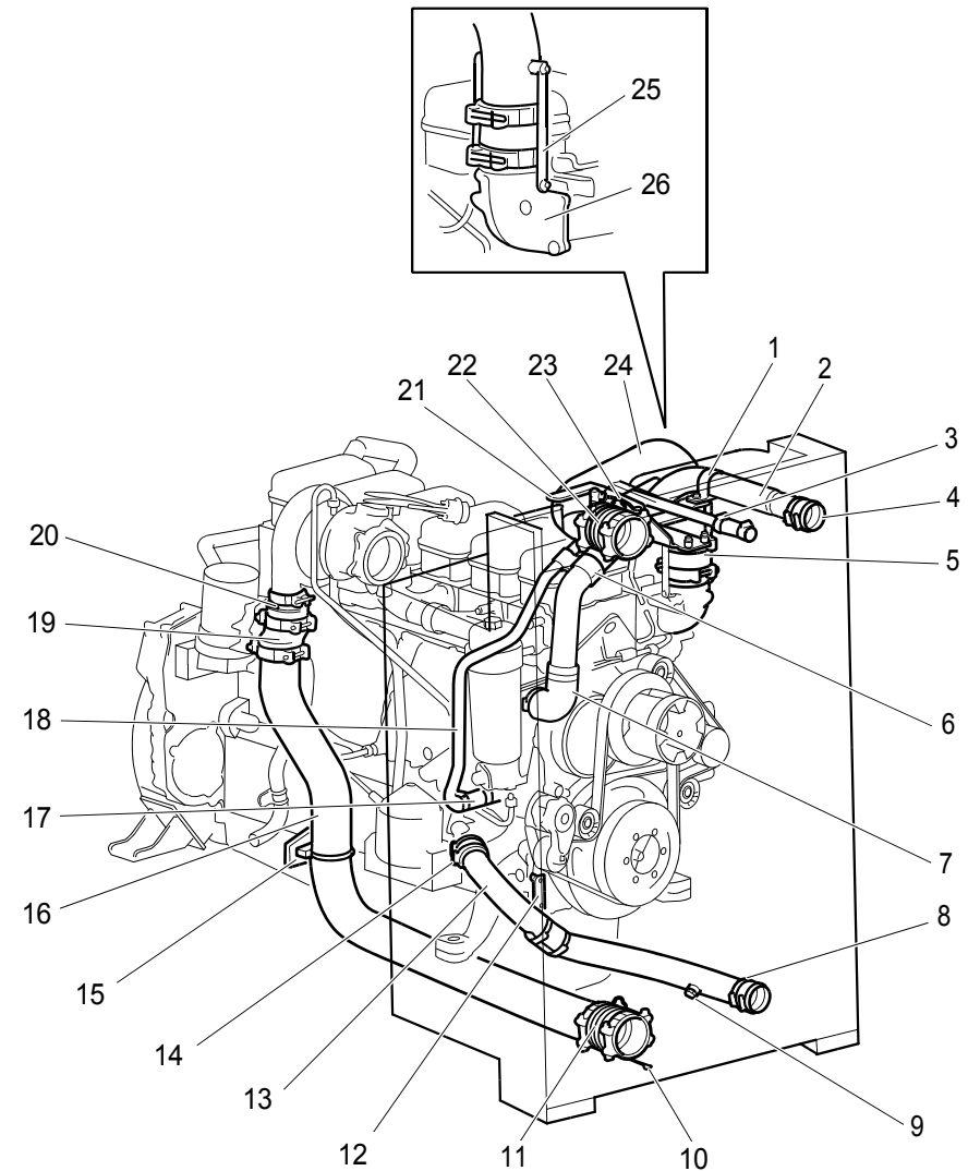
1.1 m 2 radiator for the DCI3 with a high turbocharger.
