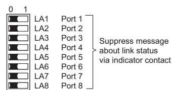
Fig. 2: 8-pin DIP switch on RS2-TX
