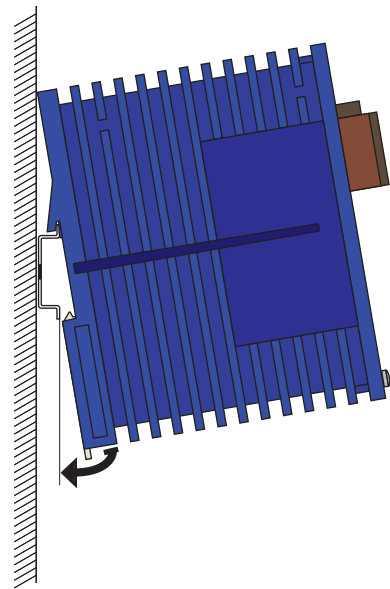
Fig. 6: Assembling the RS2-TX
