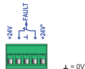
Fig. 5: Pin configuration of 5pin terminal block
