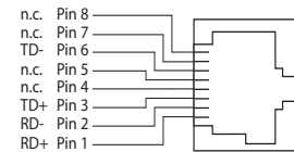
Fig. 3: Pin configuration of an TP/TX interface
