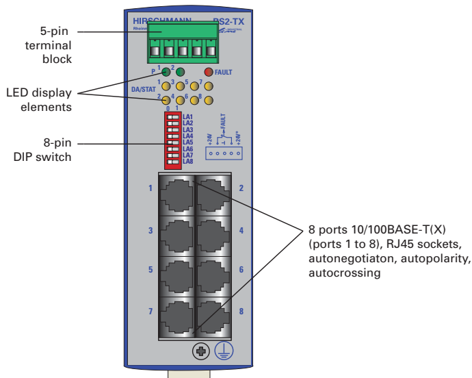
Fig. 1: Overview interfaces, display elements and controls of the RS2-TX
