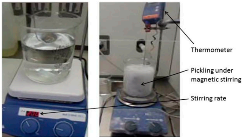
Figure 3. Pickling setup.
