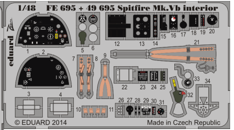
49695 Spitfire Mk.Vb interior S.A. 1/48 Airfix
