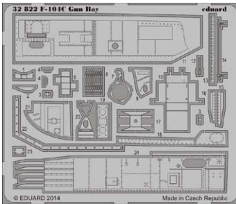
32822 F-104C gun bay 1/32 Italeri
