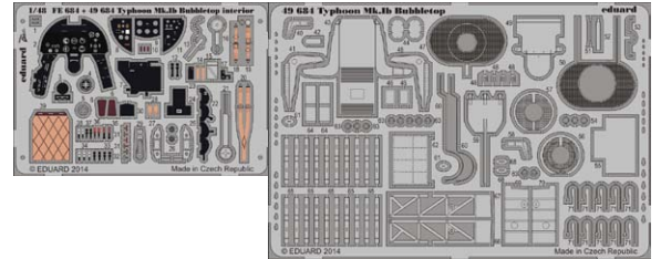
49684 Typhoon Mk.Ib Bubbletop interior S.A. 1/48 Italeri/Hasegawa
