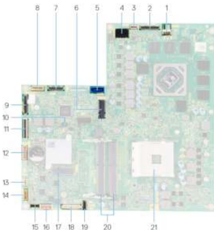
Figure 2. System-board components
