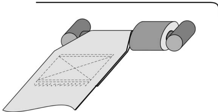
A fold in webbing installed to a bell bar system with a spacer.
