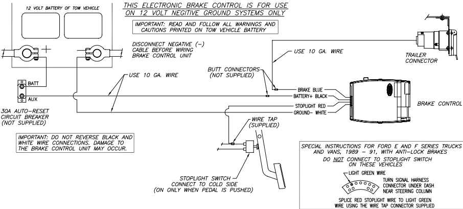
WIRING DIAGRAM
