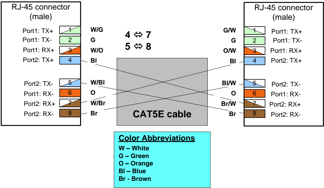
Figure 11 Protection Signaling Cable Pinouts
