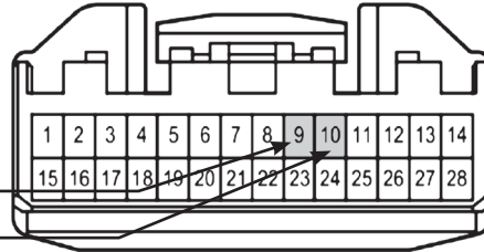
(this is the pin view of the factory harness)
