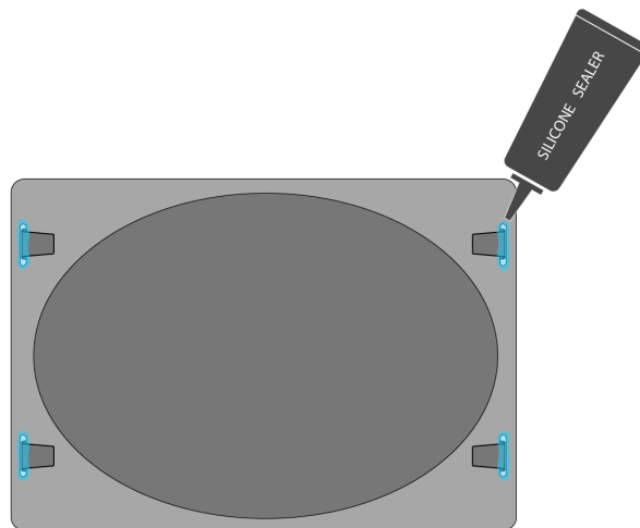
Silicone the Speaker Grill Tab Openings
