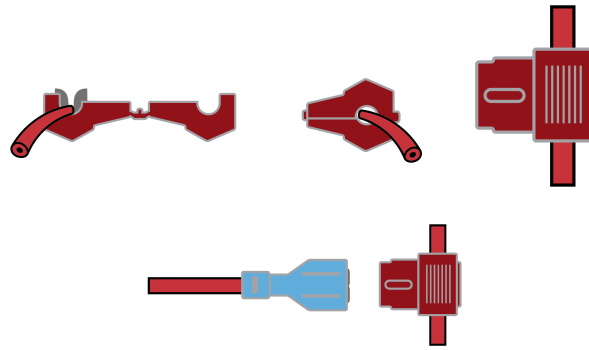
T-Tap Wire Connectors
