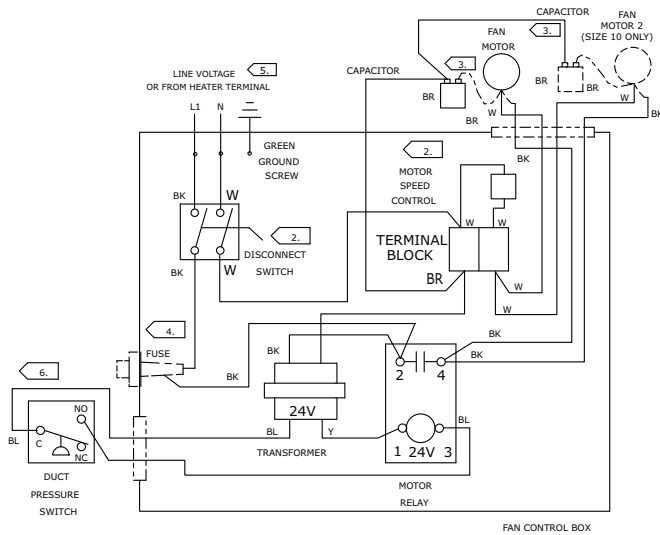
Fan-Powered Low-Height Control Box Duct Pressure Switch Option
