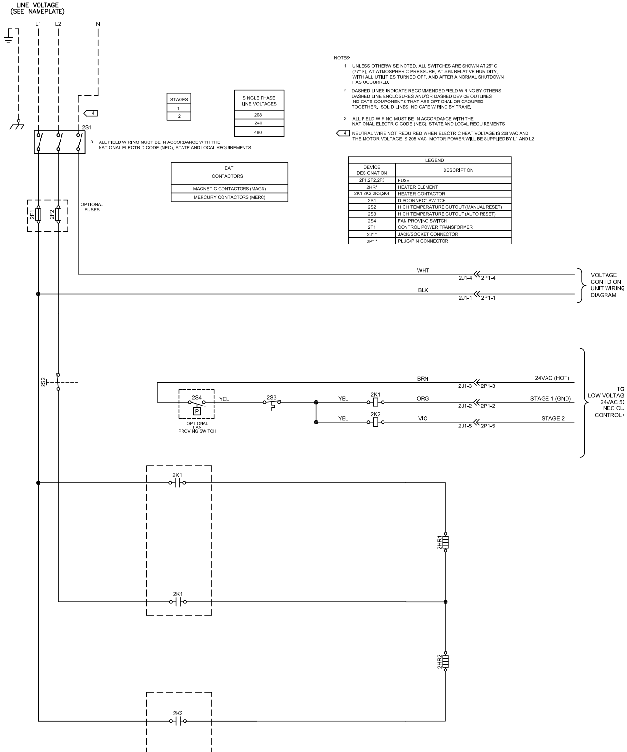
Figure 34. Fan powered, single phase, 2 legs, 2 stages
