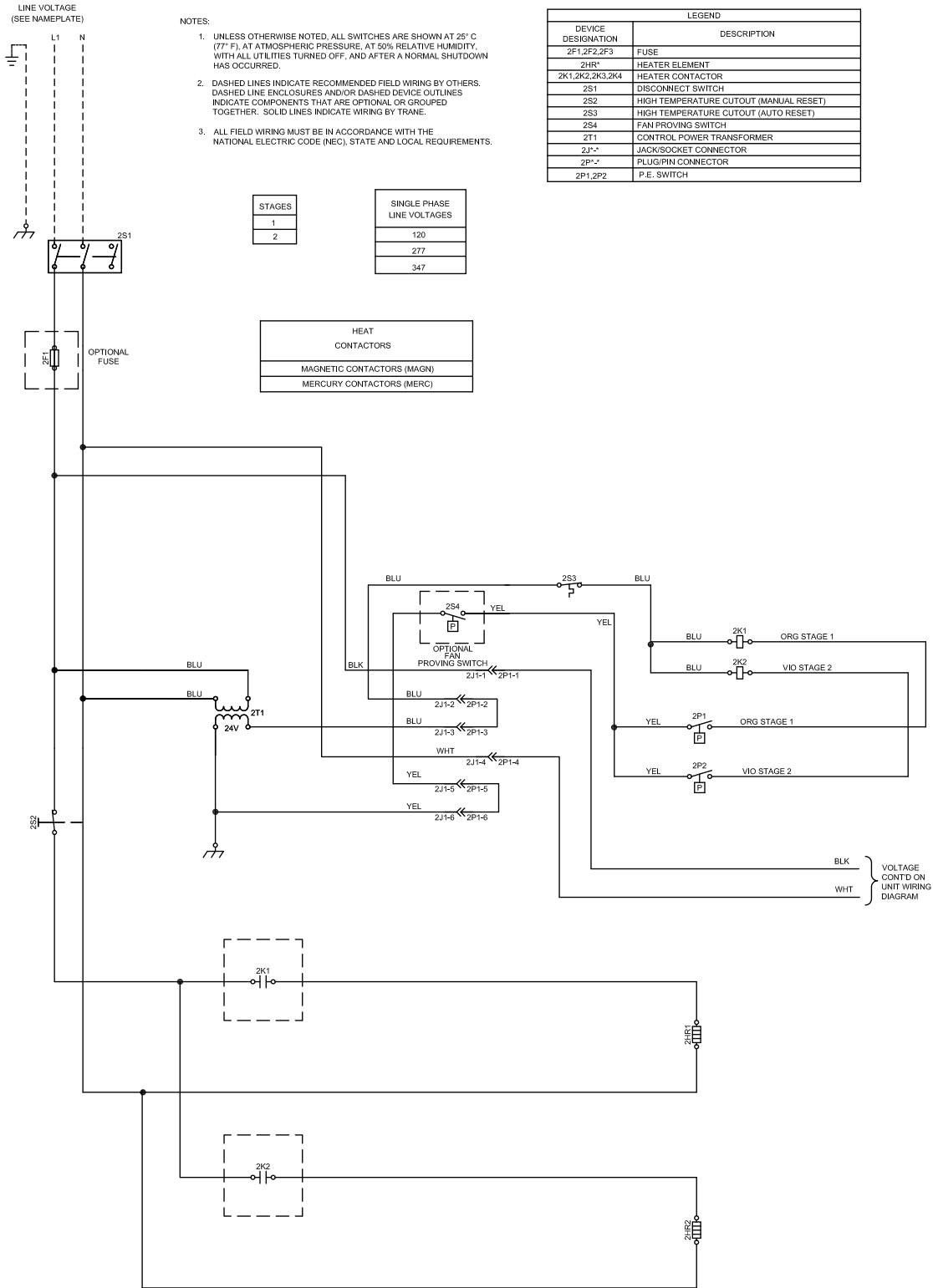
Figure 36. Fan powered, single phase, 1 leg, 2 stages
