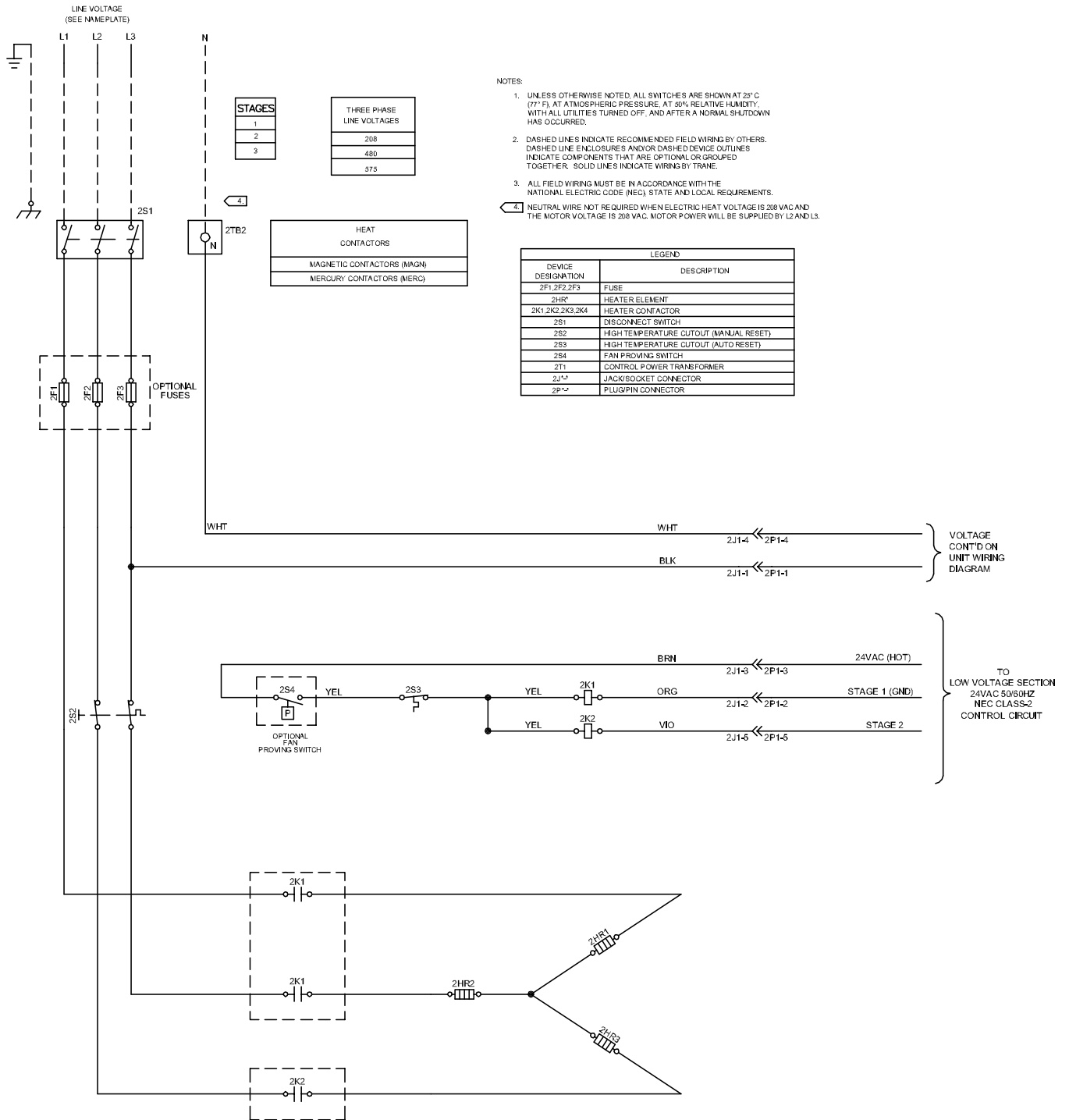
Figure 35. Fan powered, three phase, wye, 2 stages
