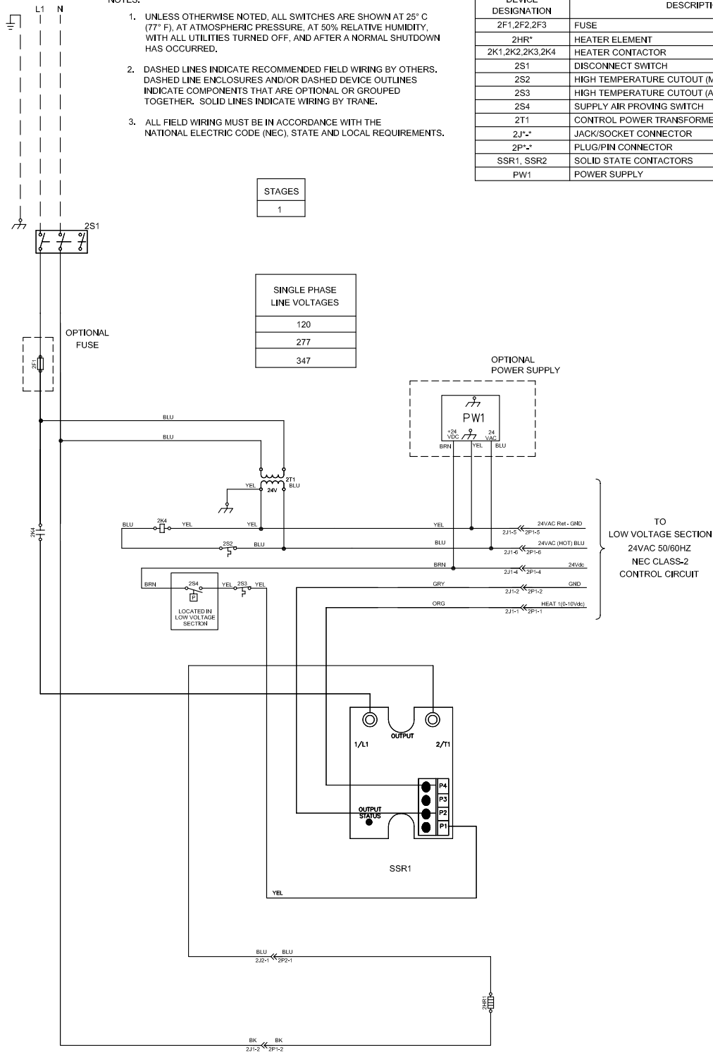
Figure 29. Single duct, single phase, SCR, 1 leg, 1 stage
