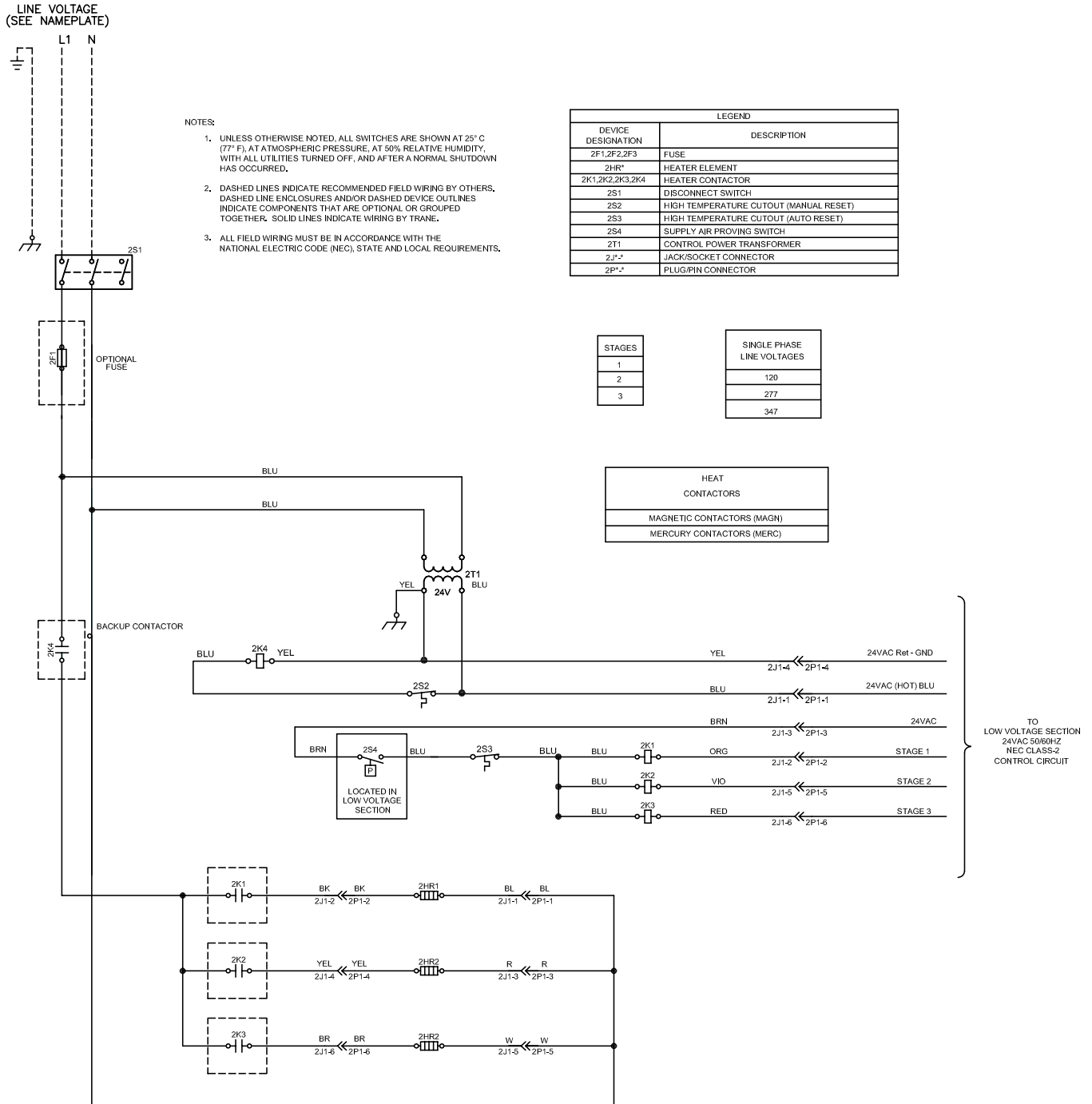
Figure 26. Single duct, single phase, 1 leg, 3 stages
