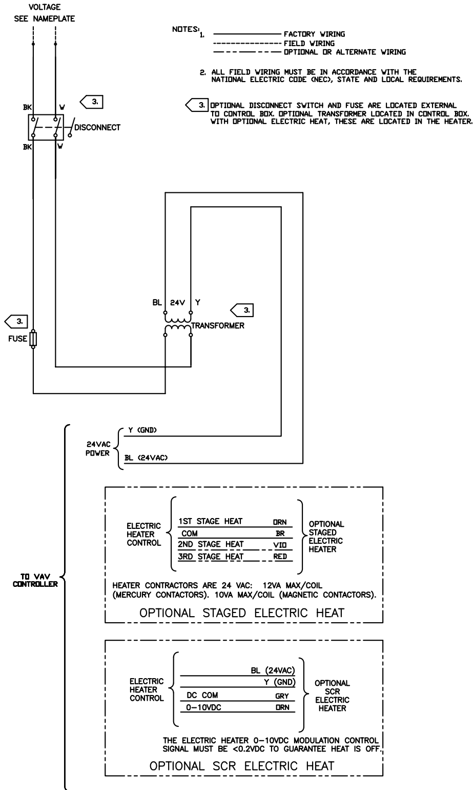
Figure 39. Single duct control box
