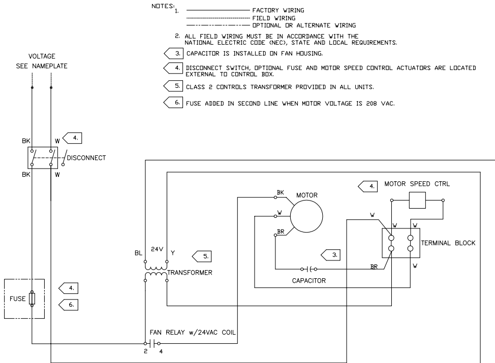
Figure 40. Fan-powered units with PSC motors
