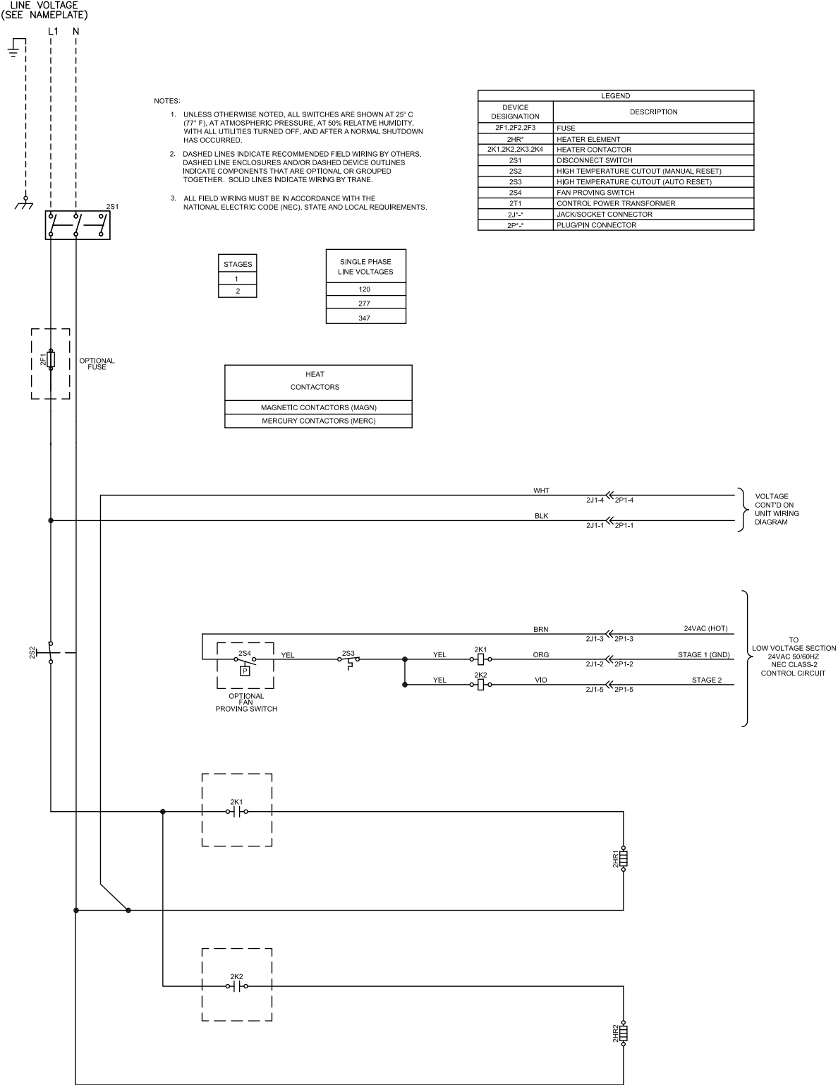
Figure 33. Fan powered, single phase, 1 leg, 2 stages
