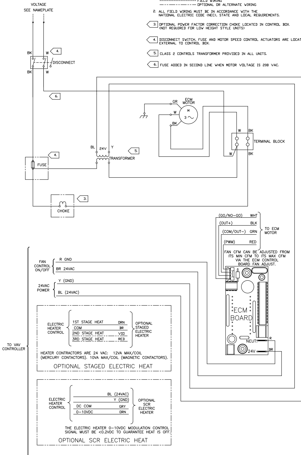
Figure 41. Fan-powered units with ECM motor
