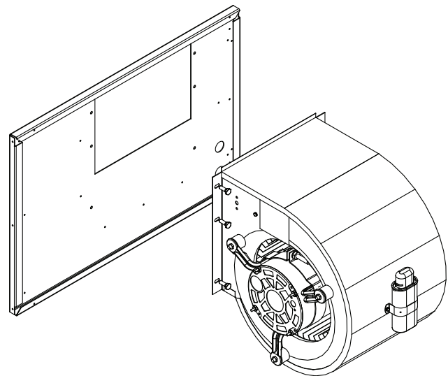
Figure 47. Standard motor removal
