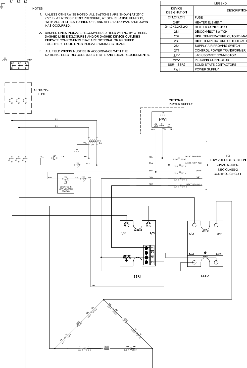
Figure 31. Single duct, three phase, delta, SCR, 1 stage
