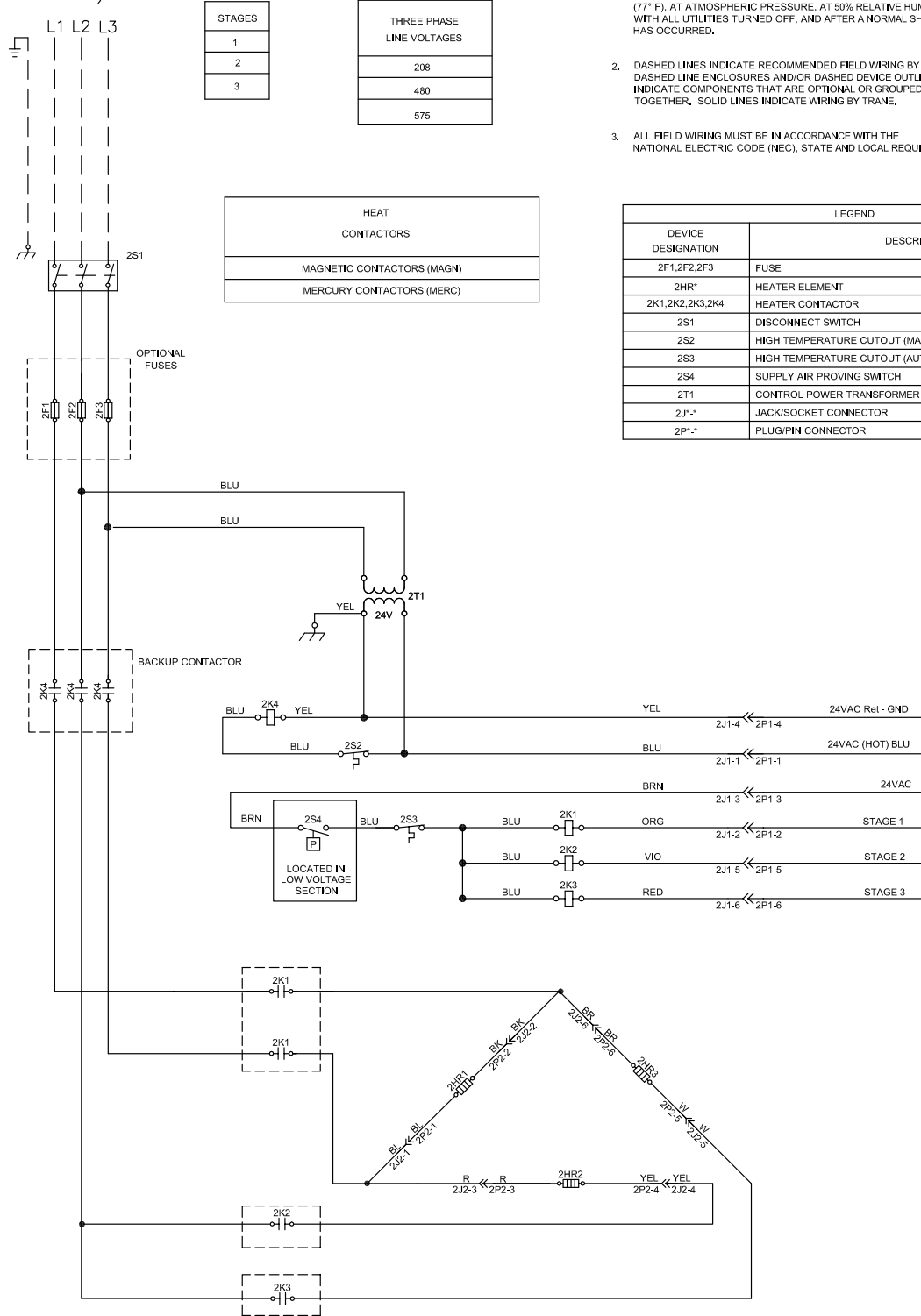
Figure 28. Single duct, three phase, delta, 3 stages
