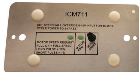
Figure 24. ECM control board – Modulating control with non-Trane unit controller
