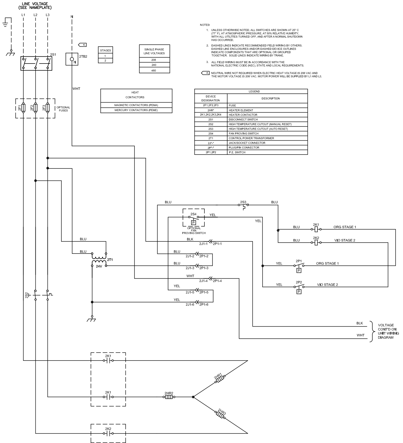
Figure 38. Fan powered, three phase, wye, 2 stages
