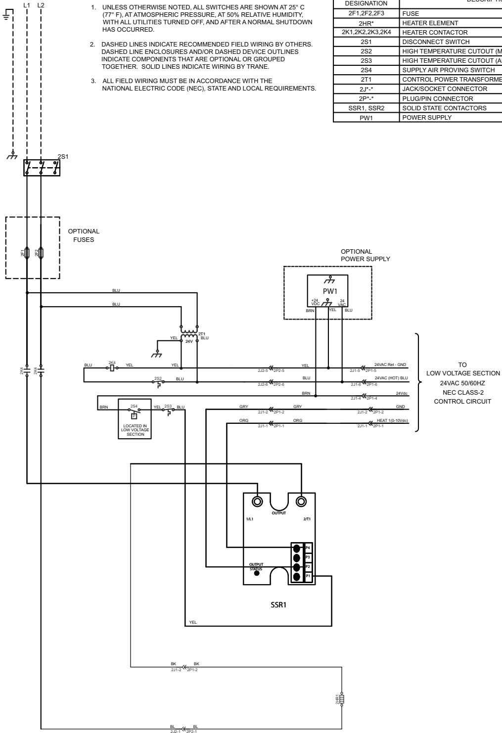
Figure 30. Single duct, single phase, SCR, 2 legs, 1 stage
