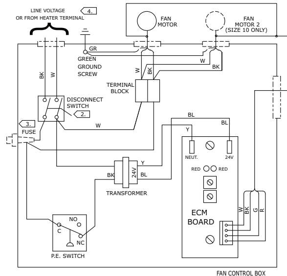
Fan-Powered Low-Height Control Box w/ ECM
