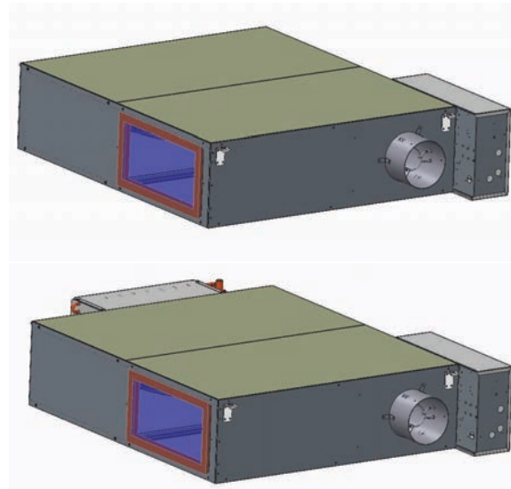
Figure 4. Low height series: LSCF (top) and low height series: LSWF (bottom)
