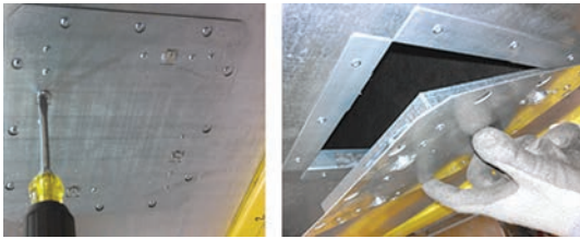
Figure 20. Bottom access
