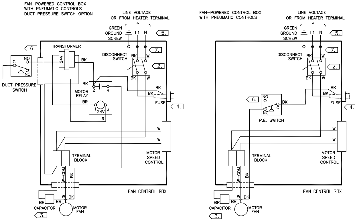
Figure 43. Fan-powered, old style
