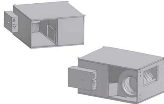
Figure 4. Low height series: LSCF (top) and low height series: LSWF (bottom)
