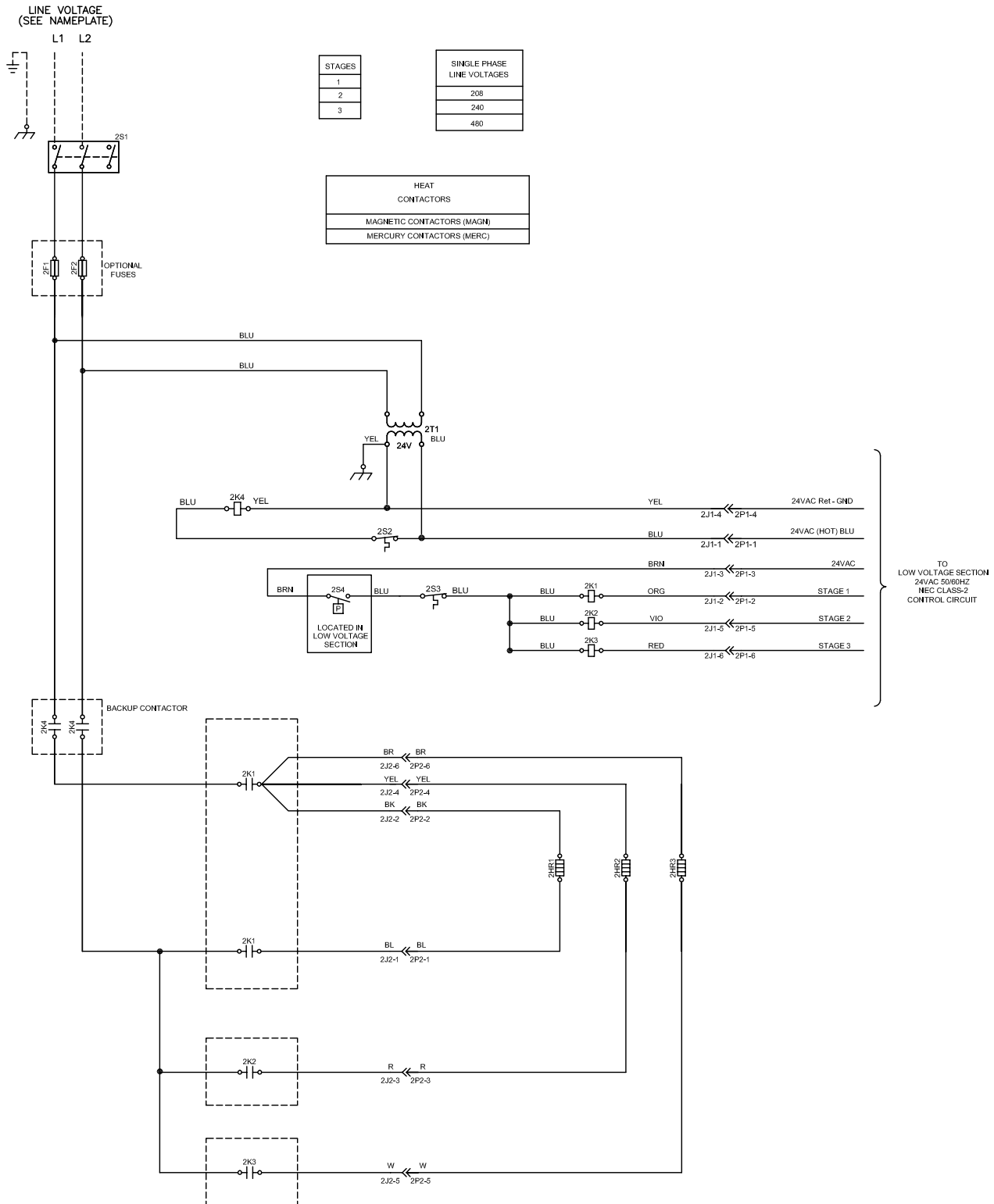
Figure 27. Single duct, single phase, 2 legs, 3 stages
