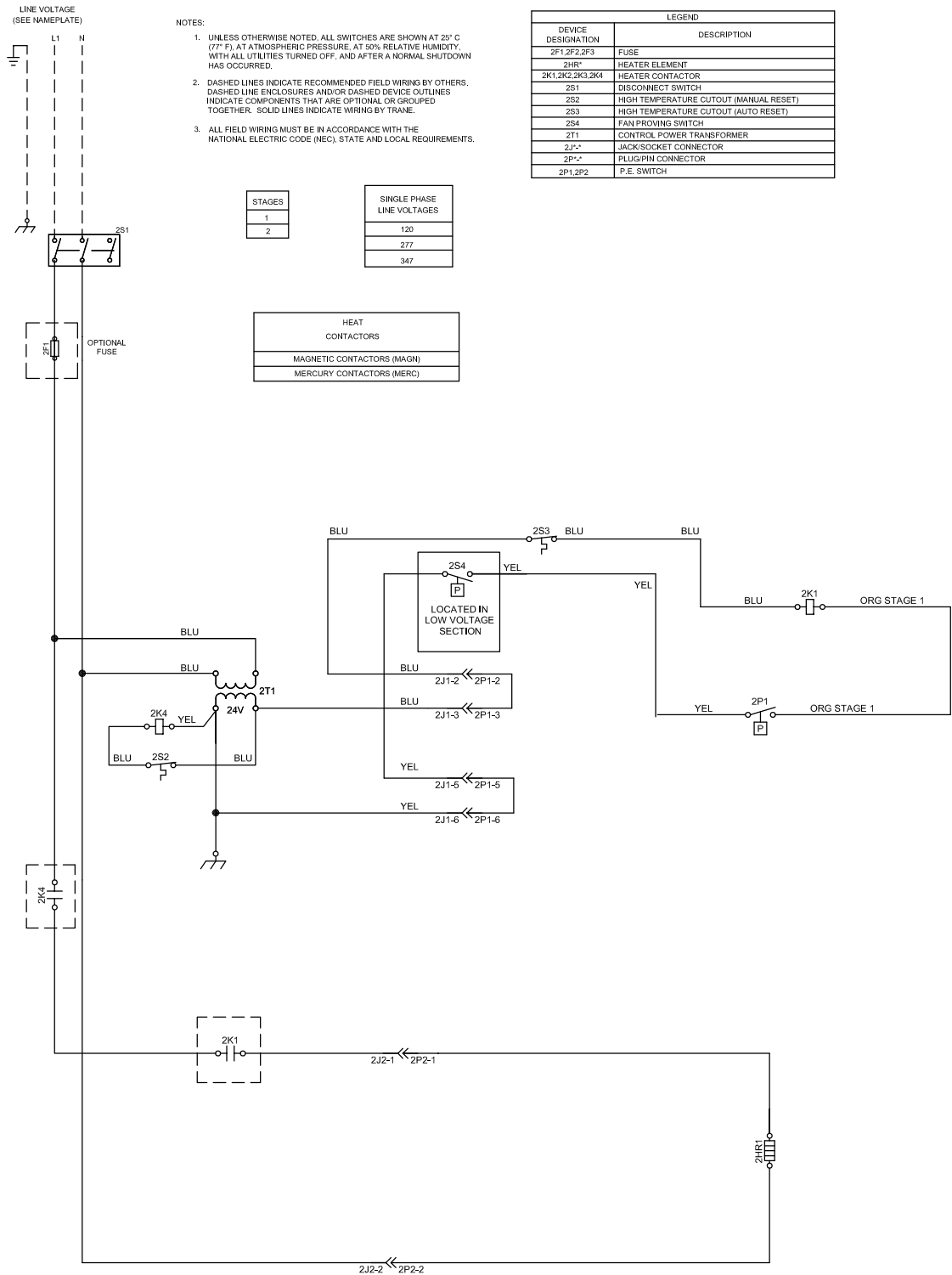
Figure 32. Single duct, single phase, 1 leg
