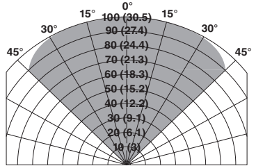
Field of View at Indicated Distance in Feet (m) for JP-5 at Medium Sensitivity (2 x 2 foot)
