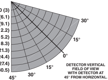
Field of View at Indicated Distance in Feet (m) for Methane at Very High Sensitivity (30 inch plume)
