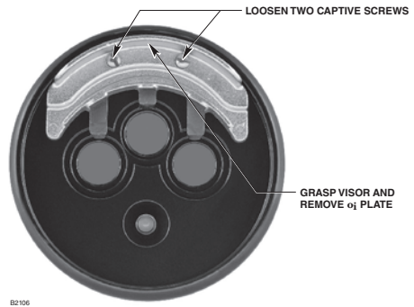
Figure 18— oi Plate Removal
