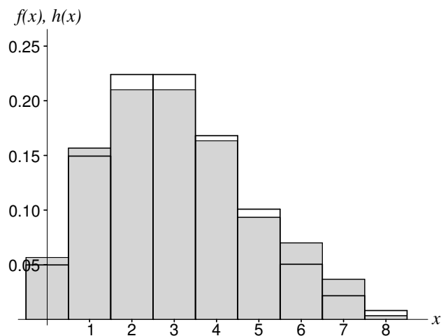
Figure 2.6-12: Background radiation
