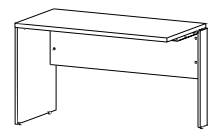
L-Unit Extension w/Support Modesty Panel KD
