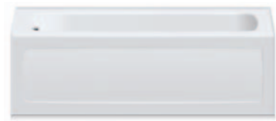
K3060 SL/SR 60 x 30 x 20.5" (152 x 76 x 52 cm) s m a w K3260 SL/SR 60 x 32 x 20.5" (152 x 81 x 52 cm) s m a w K3666 SL/SR 66 x 36 x 20.5" (168 x 91 x 52 cm) s m a w
