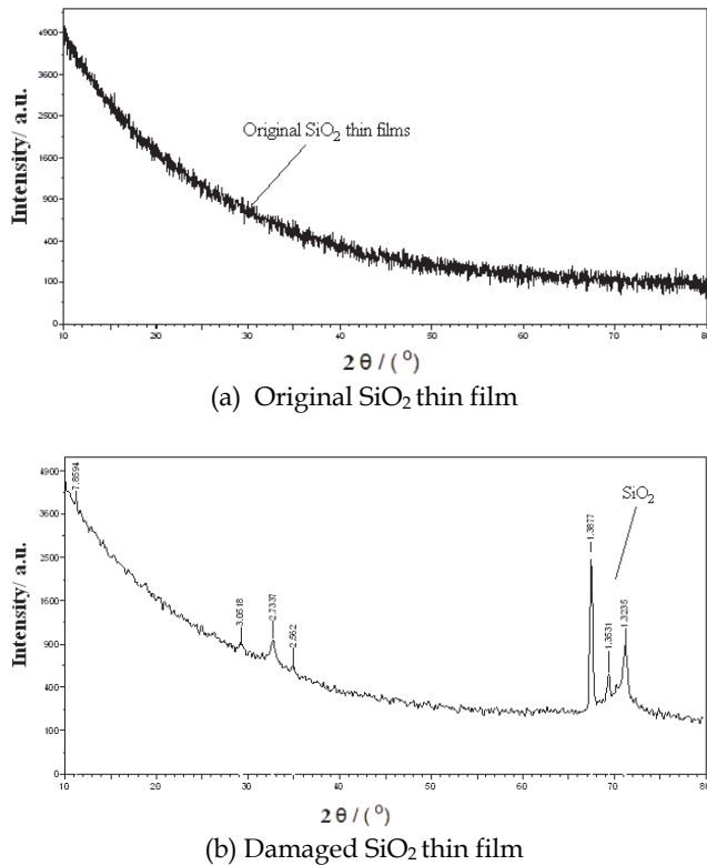
Fig. 2.5. The XRD spectra of SiO 2 thin films on lithium niobate crystal (Courtesy of Dr. Ruihua Niu)
