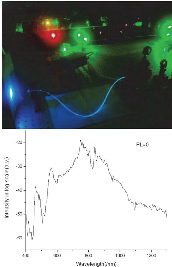
Fig. 5.2. Photonic crystal fiber and supercontinuum spectrum. (Courtesy of Dr. Ping Ying and Dr. Zairu Ma)
