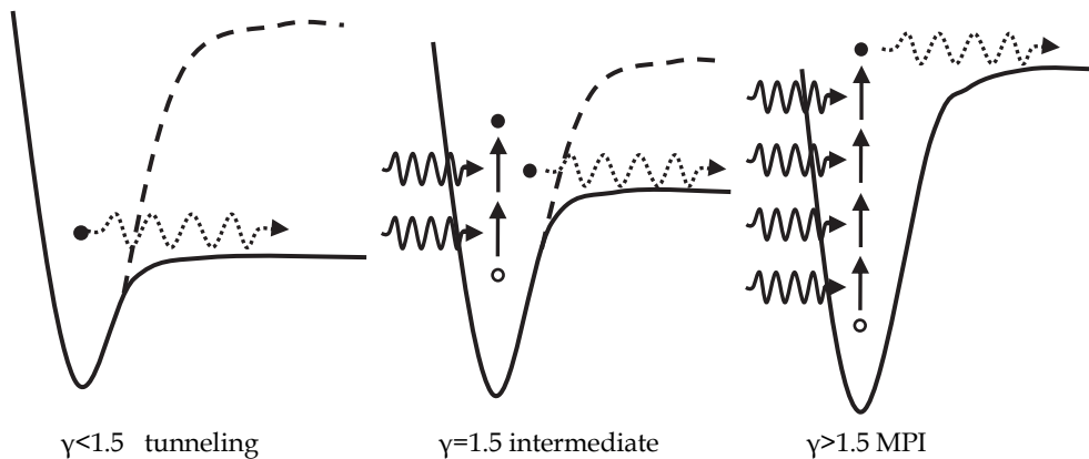
Fig. 3.1. Schematic of photo-ionization for different Keldysh parameters.
