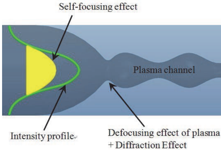
Fig. 3.3. The illustration of self-focusing filaments
