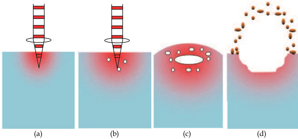
Fig. 2.6. The generation of phase explosion
