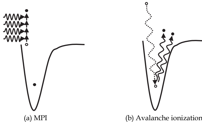
Fig. 3.2. Schematic diagram of the avalanche ionization
