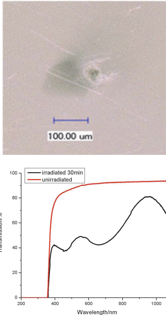
Fig. 5.4. Gray tracking in KTP crystal by 355nm laser radiation for 30min. and the transmission spectra (Courtesy of Dr. Qihui Zhang and Dr. Xiang Gao)
