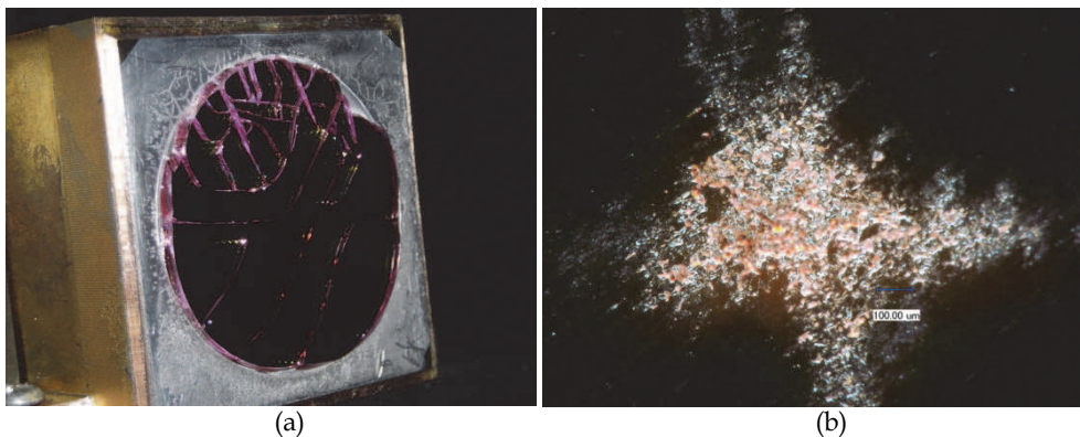
Fig. 2.1. Thermal fractures of Nd:YAG and melting of SiO 2 thin film coated on Nd:YAG in a high-energy laser (Courtesy of Dr. Huomu Yang)
