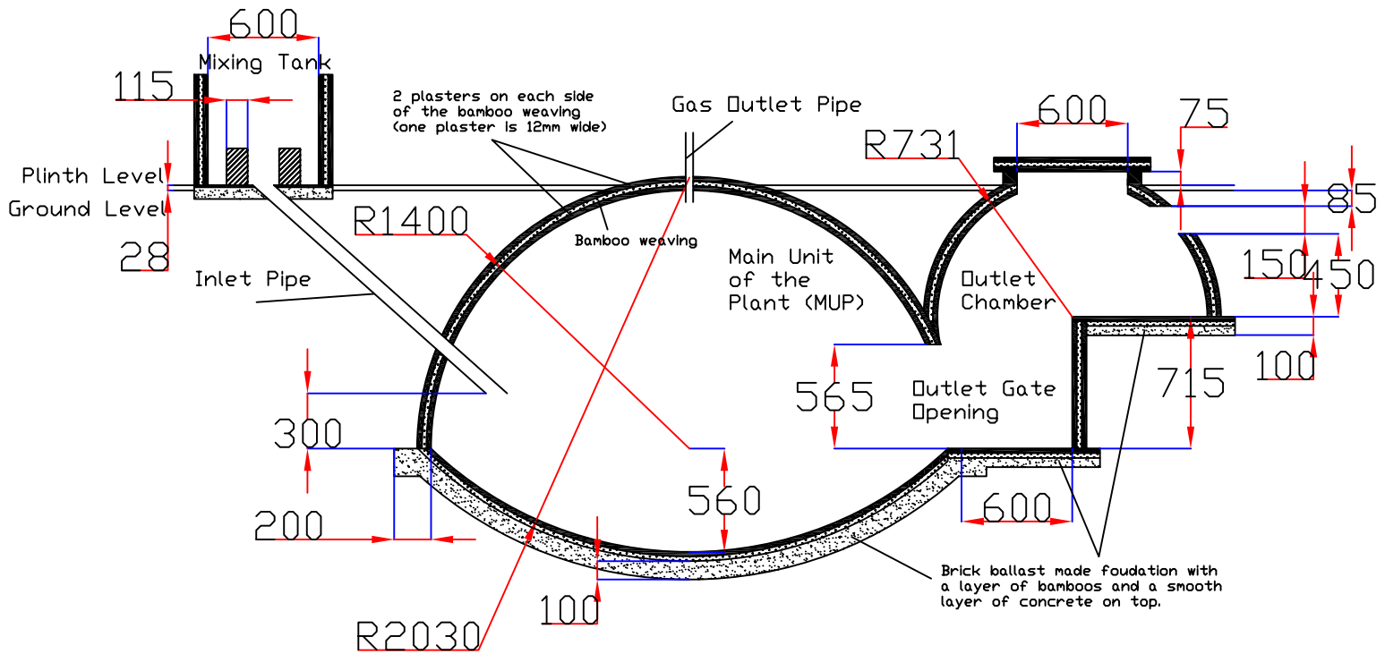
Sectional Elevation
