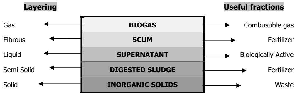
Diagram-5: By-products of Batch-fed digester
