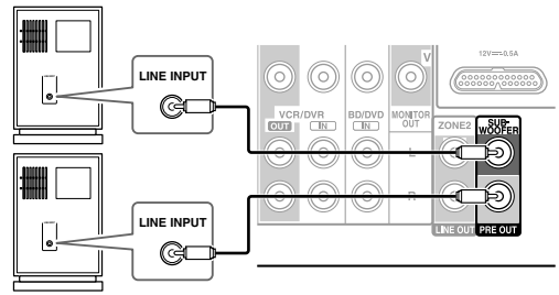
Powered subwoofer
