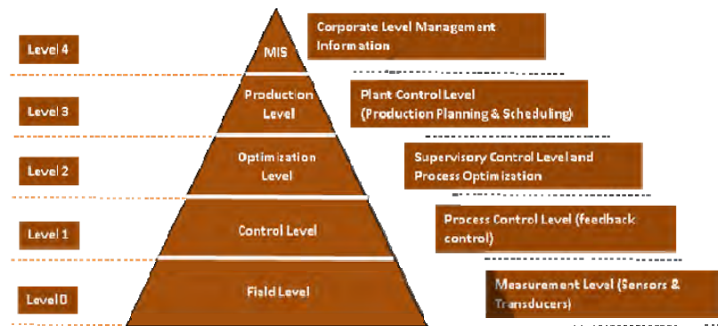
Figure 1.10 Five levels of automation hierarchy of a (hierarchical) computer based process control system
