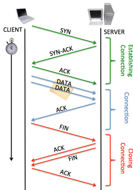
Figure 6.1: TCP protocol
