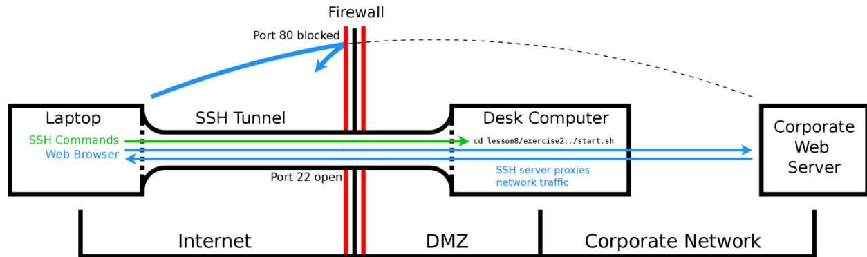
Figure 8.2: SSH tunnel
