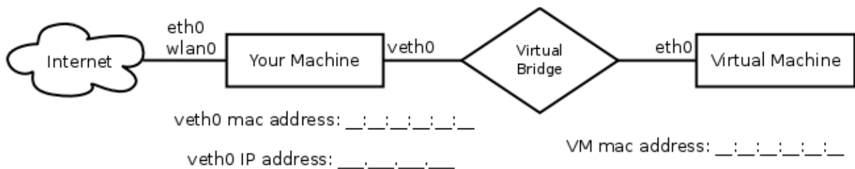
Figure 4.7: Exercise 1 topology
