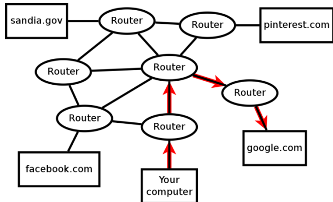
Figure 4.3: Routing
