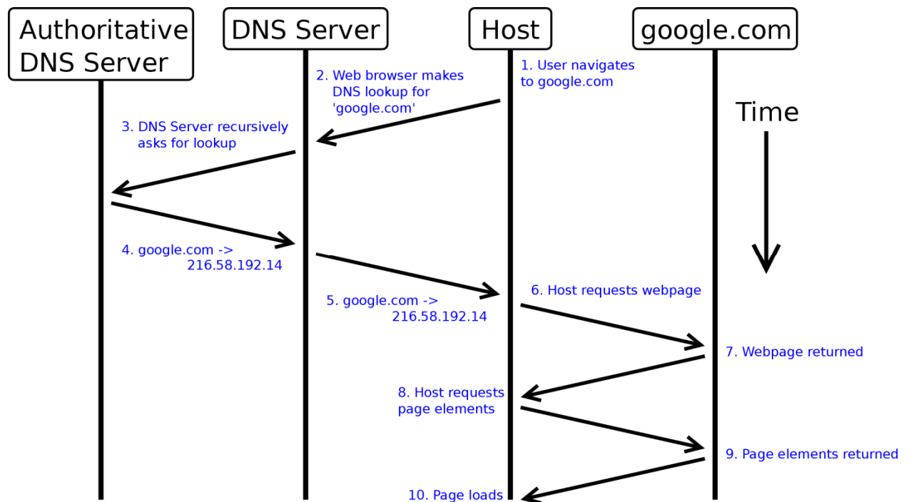
Figure 7.4: DNS Lookup
