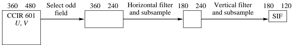
FIGURE 18.8 Generation of an SIF frame.
