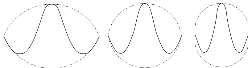
FIGURE 15.3 Three wavelet basis functions.
