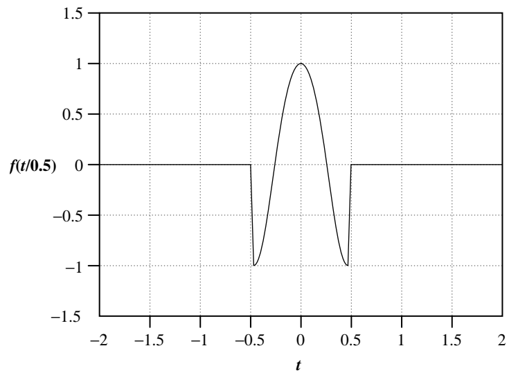
FIGURE 15. 5 The function f\left(\frac{t}{0.5}\right) .
