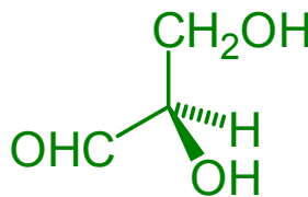
(+)-glyceraldehyde ( D-glyceraldehyde R-glyceraldehyde
