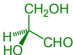
(-)-glyceraldehyde ( L-glyceraldehyde S-glyceraldehyde
