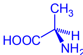
(-)-alanine ( D-alanine R-alanine
