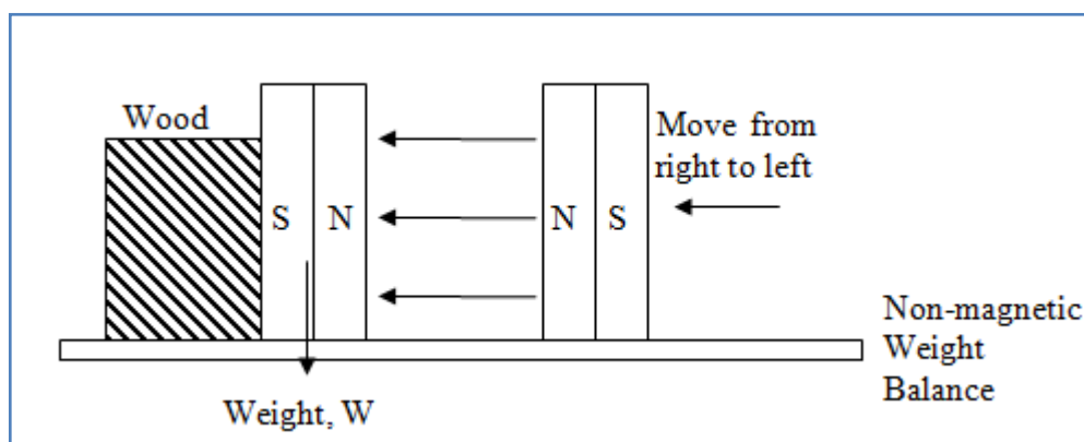
Figure 3.7: Tangential Force Measurement
