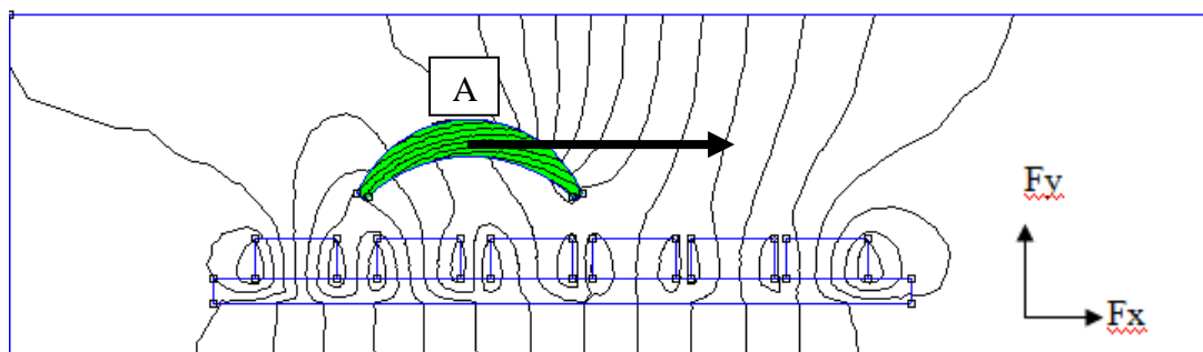
Figure 4.4: Magnetic Field Distribution between the Magnets at Position A
