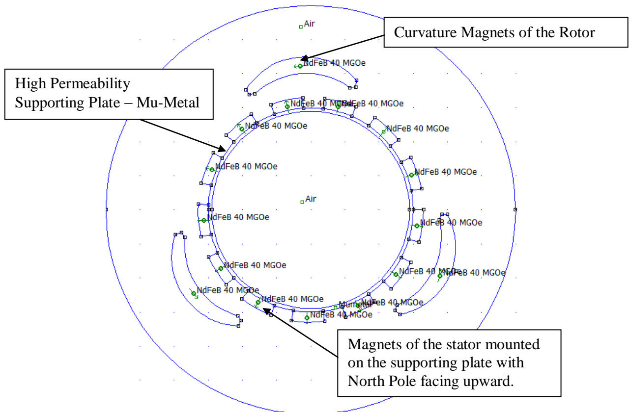
Figure 3.33: Geometry Model of Howard Johnson Motor
