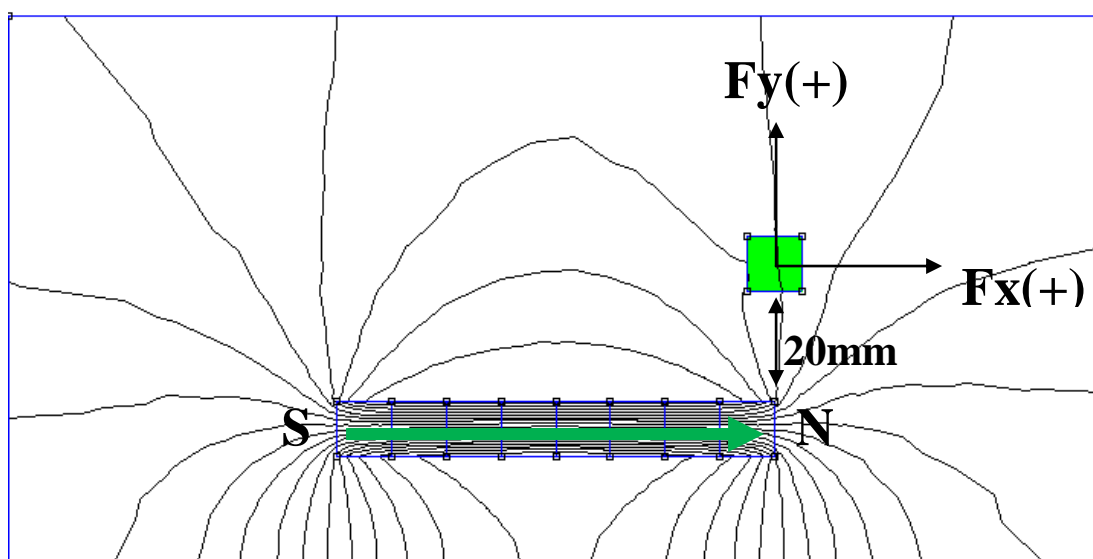
Figure 4.20: Magnetic Field Distribution for 1 st Test
