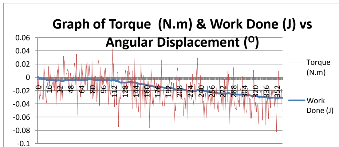
Figure 4.25: Comparison of Work Done & Torque versus the Angular Displacement of Circular Arrangement of Magnets
