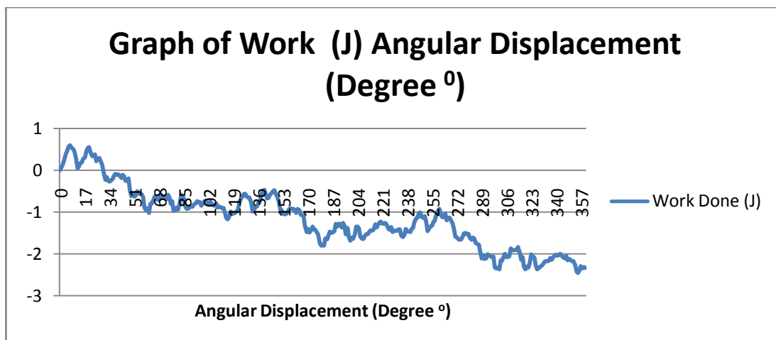
Figure 4.2: Graph of Work Done versus Angular Displacement of the rotor of Howard Johnson's Motor
