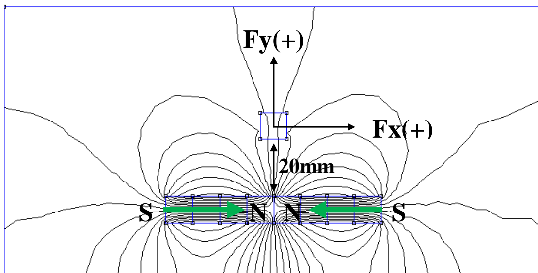
Figure 4.21: Magnetic Field Distribution for 2 nd Test
