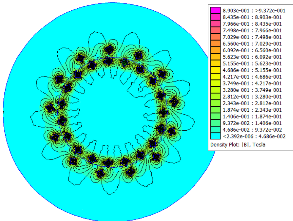
Figure 4.24: Visualization of Magnetic Field Distribution and Flux Density of Circular Arrangement of Magnets
