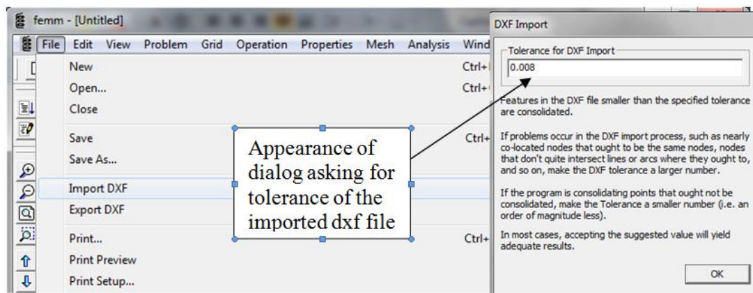
Figure 3.18: Layout of FEMM while importing dxf file
