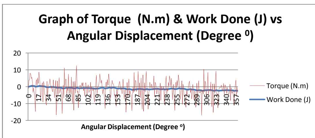
Figure 4.3: Comparison of Work Done & Torque versus the Angular Displacement of the rotor of Howard Johnson's Rotor
