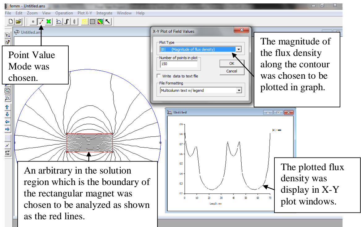
Figure 3.28: Data Extraction for Contour Mode
