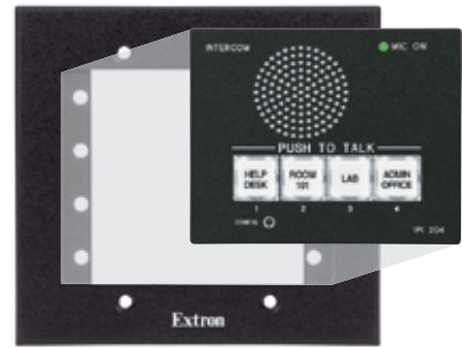
IPI 204 AAP mounted in an AAP 102 Mounting Frame
