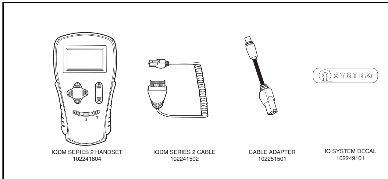
Figure 1 IQDM-P Series 2 Parts
