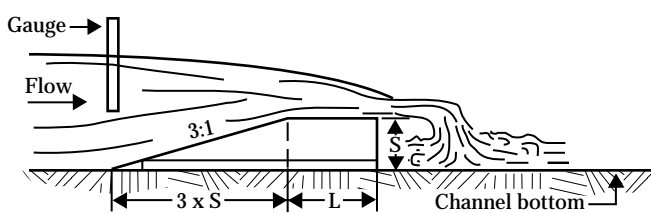
Figure 9-40 Profile of long-throated flume (from Bos, Replogle, Clemmens)
