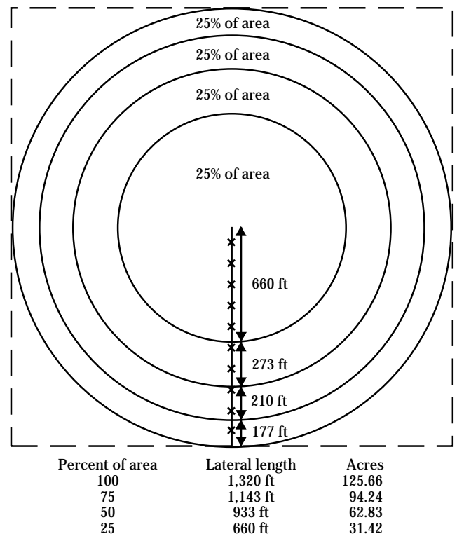
Figure 6-11 Application area along a quarter-mile-long pivot system lateral
