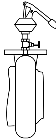
Figure 12-10 Priming arrangements for centrifugal pumps (courtesy of Cornell Pump Company)
