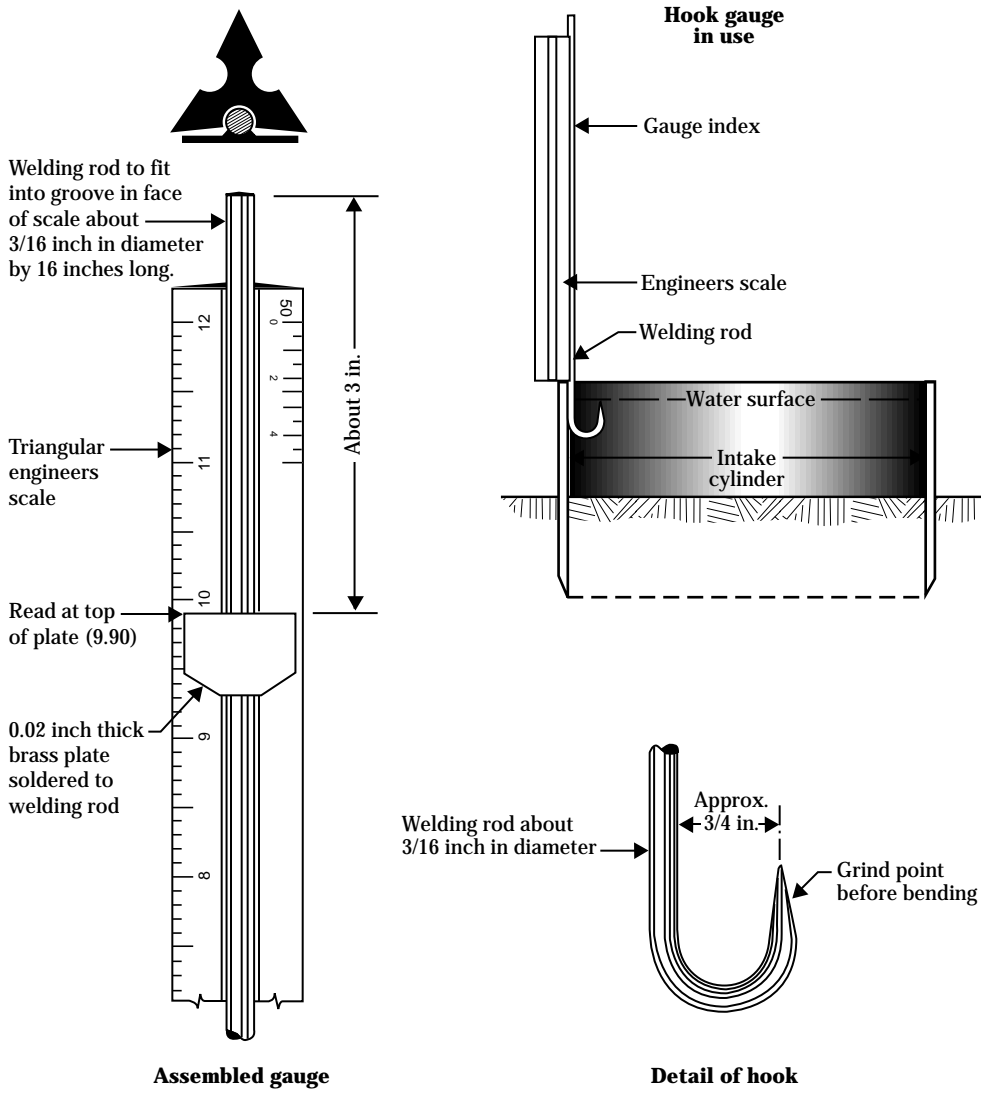
Figure 9-32 Cylinder infiltrometer—Continued
