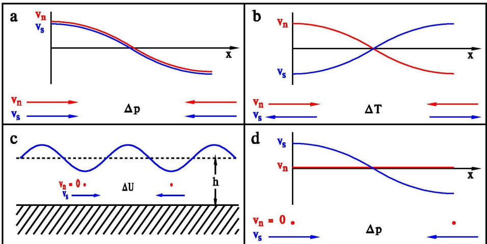
Figure 2. Schematic representation of four of the six sound modes that can be excited in superfluid helium. The red lines and arrows indicate the velocity of the normal fluid component ( \vec{v}_n ) and the blue lines and arrows indicate the velocity of the superfluid component ( \vec{v}_s ). a: First sound is restored by the pressure difference ( \Delta p ). b: Second sound is restored by a temperature difference ( \Delta T ). c: Third sound is a surface wave in atomically thin helium layers of thickness, h , adsorbed on a solid substrate. The surface wave's restoring force is provided by the van der Waals attraction ( \Delta U ) between the helium and the substrate. Only the superfluid can move (i.e., \vec{v}_n = 0 ) because the normal fluid is immobilized by its non-zero viscosity. d: Fourth sound propagates in porous media where the small pore size immobilizes the normal fluid component while the superfluid component can oscillate since it has no viscosity. Pressure differences ( \Delta p ) provide the restoring force for fourth sound. Fifth sound is not shown, but it also is present in porous media if the pressure is relieved by a free surface or in thick helium films. Temperature gradients provide the restoring force for fifth sound.
