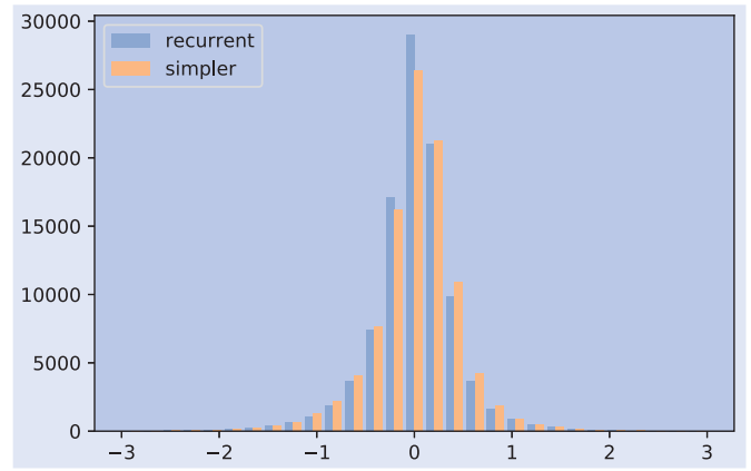
Figure 4. Comparison of deep hedging strategies with recurrent structure to those with a simpler network structure when no transaction costs are incurred. The figure shows a histogram of the terminal hedging error q - Z + (\delta^\theta \cdot S)_T evaluated on the test data, for both \delta_k^\theta = F^{\theta_k}(I_k, \delta_{k-1}^\theta) (recurrent) and \delta_k^\theta = F^{\theta_k}(I_k) (simpler). Both strategies were optimized with \alpha = 0.5 in (28).
