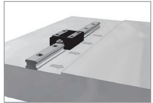
▲ Fig. 8: Align to a machined alignment edge.
