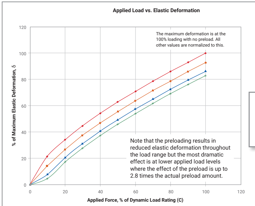
Fig. 3: Effect of bearing preload on the elastic deformation of the bearing/race system.
