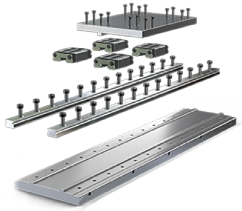
Fig. 14: Components of a Bearing Block System.
