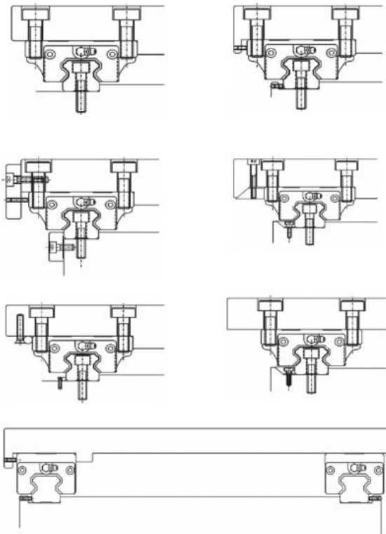
▲ Fig. 10: Common methods to attach bearing blocks and rails.
