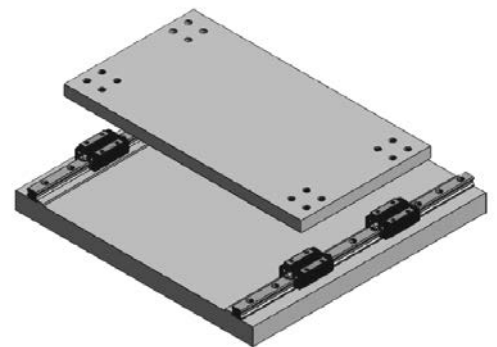
▲ Fig. 9: Two rails in parallel. Each has a machined alignment edge to rest against.
