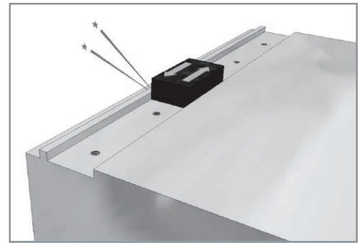
▲ Fig. 7: Remove dents, burrs, and dirt from the mounting surface.
