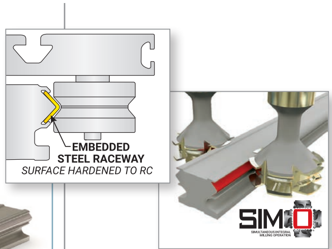
◀ Fig. 12: Example of an IVT Rail and Carriage System with schematic of IVT system
