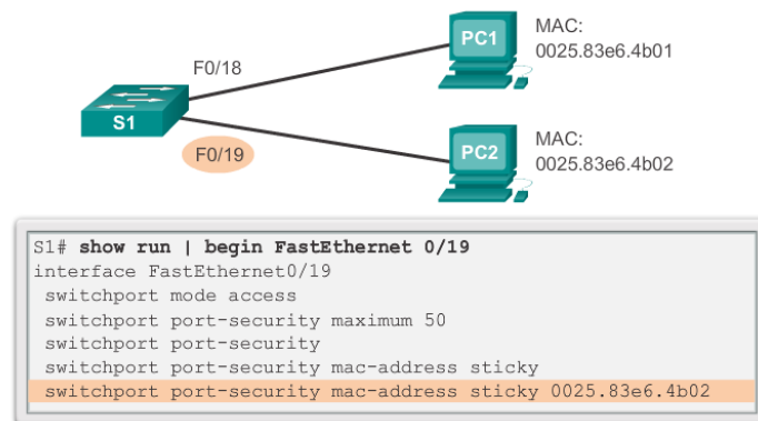
Fig. 2.12 Melihat Port Security Sticky Running Config
