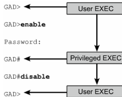
Fig. 2.2 Perubahan User EXEC Privileged EXEC
