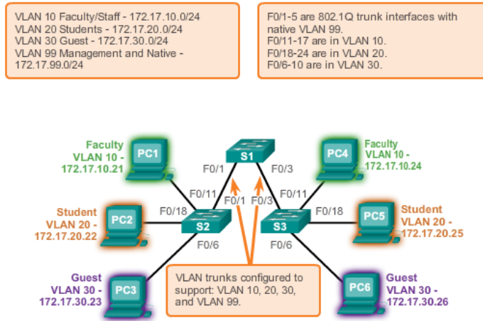
Fig. 3.3 VLAN Trunk
