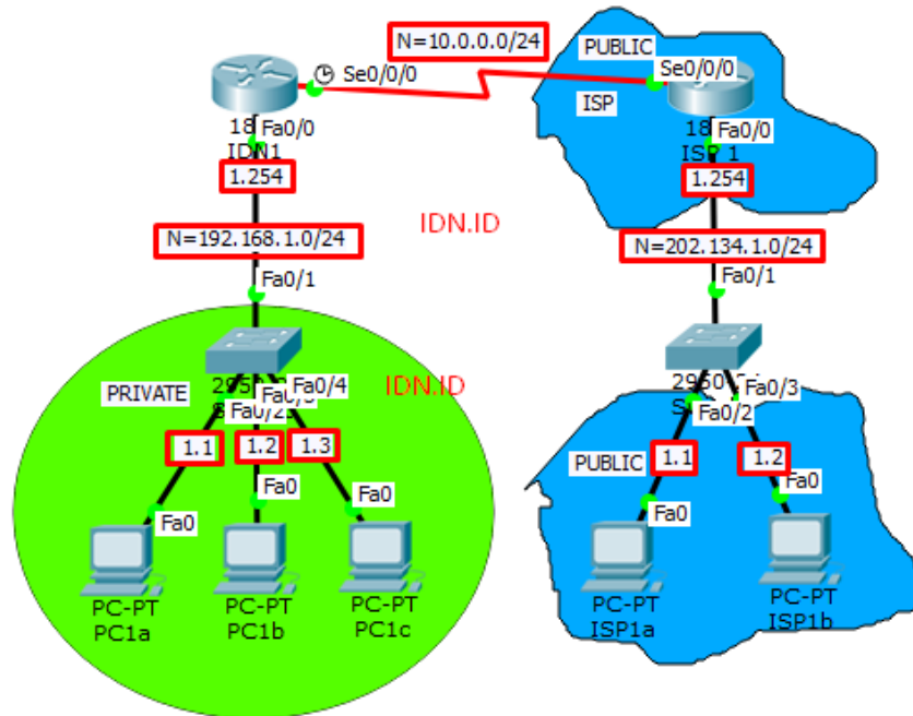
Fig. 11.8 NAT Dinamis
