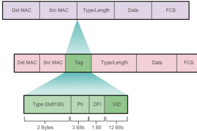
Fig. 3.4 Field Ethernet 802.1Q Frame
