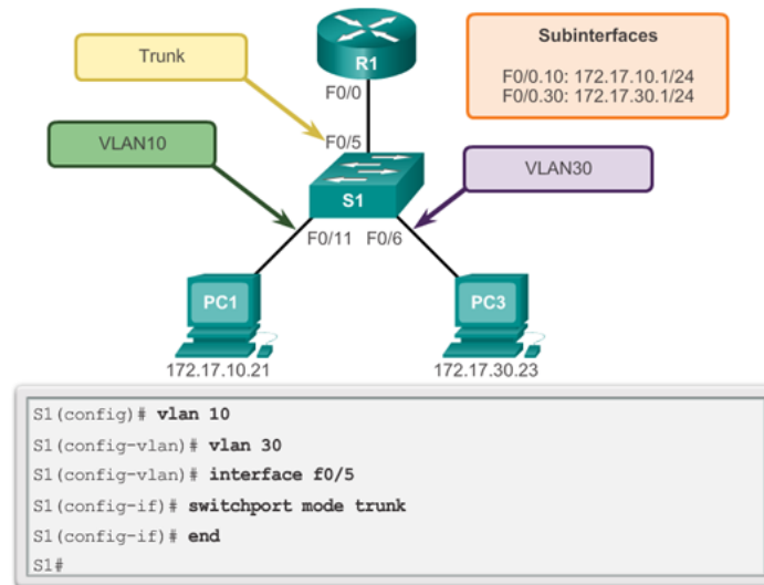
Fig. 5.3 Topologi Router On A Stick
