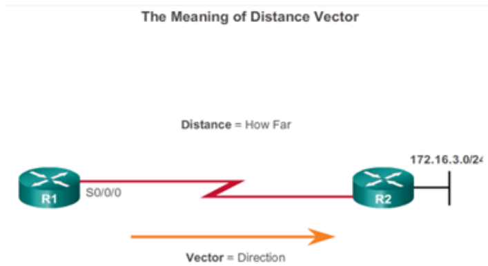
Fig. 7.10 Protokol Routing Distance Vector
