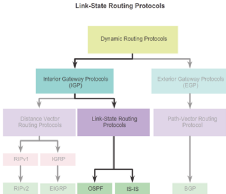
Fig. 7.17 Protokol Routing Link State
