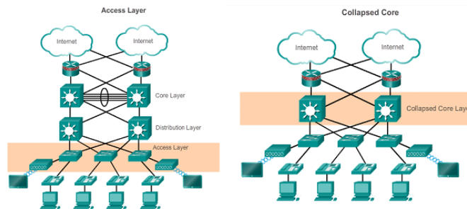
Fig. 1.6 Hierarchy Networks
