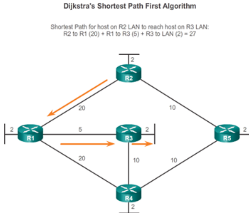
Fig. 7.18 Disjark Algorithm
