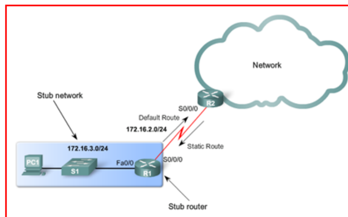
Fig. 6.1 Stub-network
