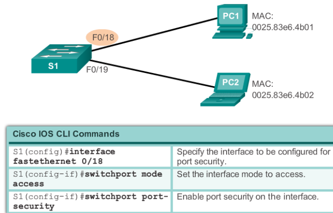
Fig. 2.10 Konfigurasi Dynamics Port Security
