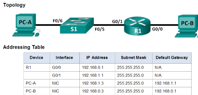
Fig. 4.11 Lab Topology
