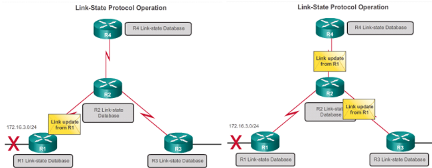
Fig. 7.11 Protokol Routing Link State
