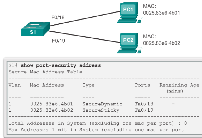
Fig. 2.13 Melihat Port Security Secure Mac Address
