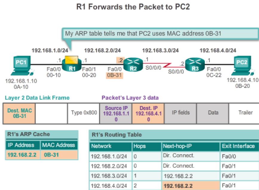
Fig. 4.15 Forward paket
