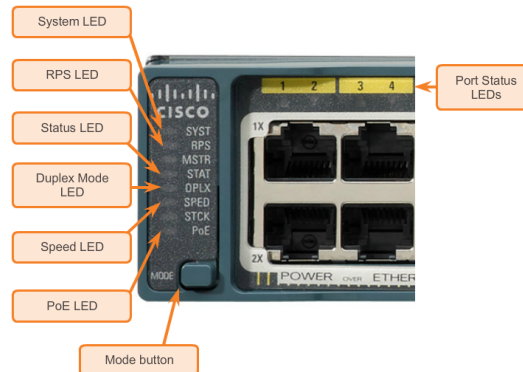
Fig. 2.3 Cisco Catalyst 2960
