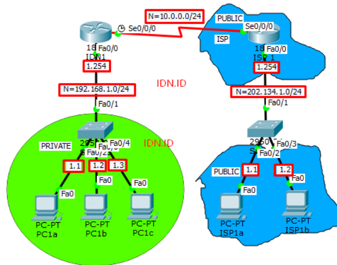
Fig. 11.4 NAT Static
