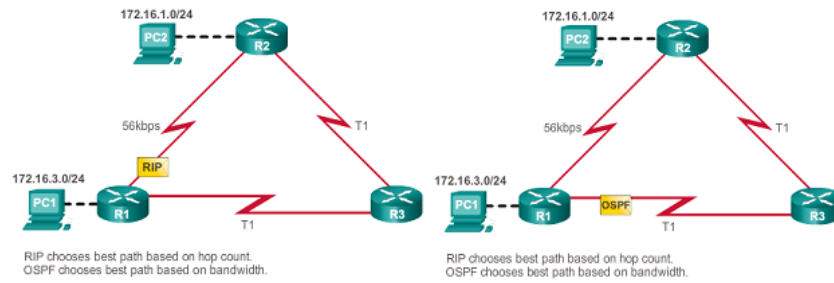
Fig. 7.13 Metrics Protokol Routing
