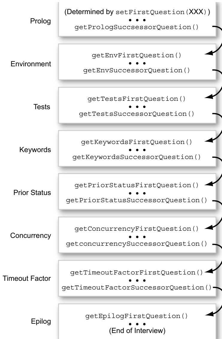
FIGURE 6-1 Interview Question Group First/Next Question Methods
